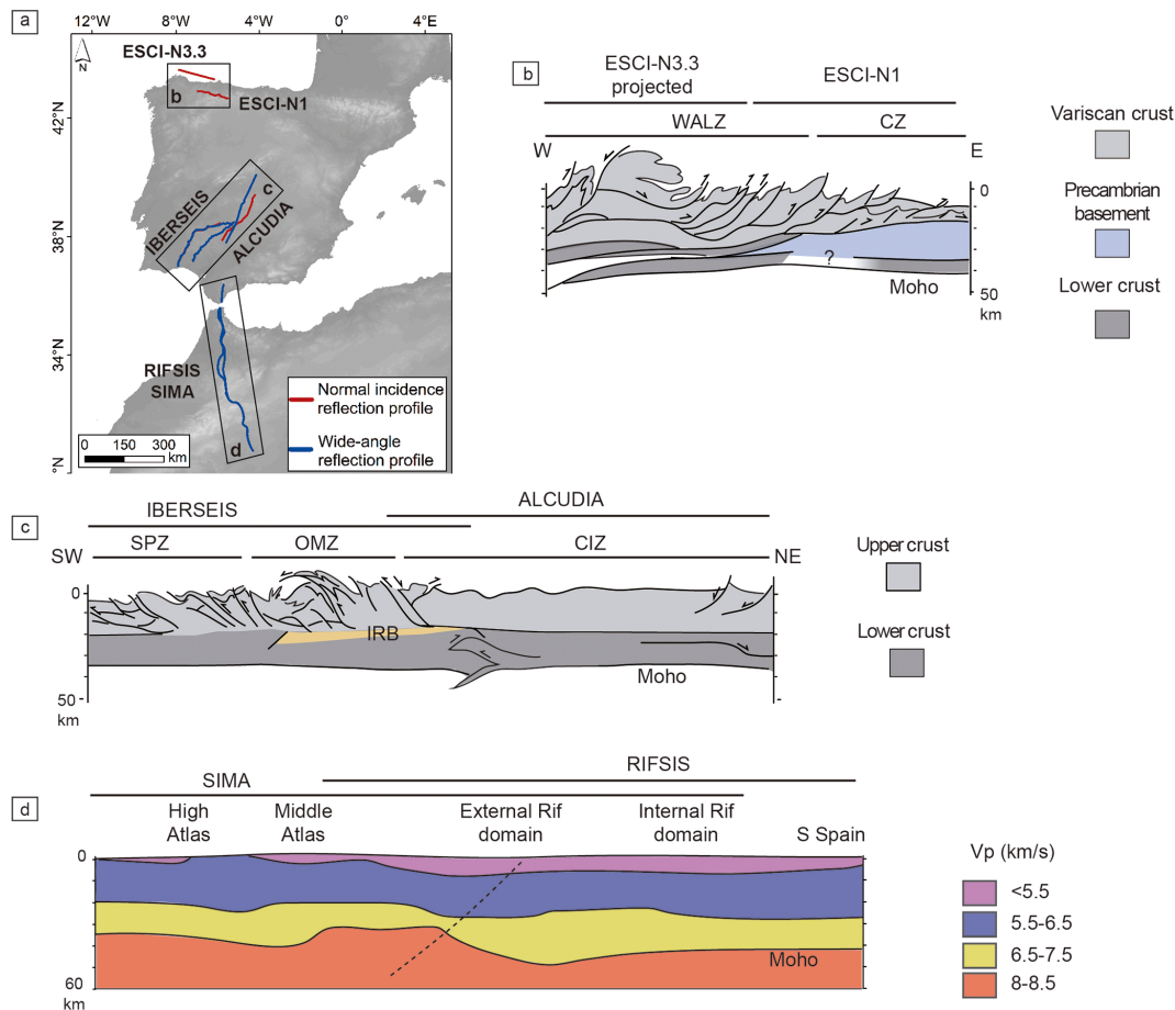
Figure 4. (a) Map of the Iberian Peninsula and north of Africa with the location of the ESCI-N, IBERSEIS, ALCUDIA, RIFSIS, and SIMA projects. The topography is from OpenTopography (Ryan et al., 2009); (c) crustal structure of the southern Iberian Massif (SPZ: South Portuguese Zone; OMZ: Ossa Morena Zone; and CIZ: Central Iberian Zone; IRB: Iberian Reflective Body) revealed by the IBERSEIS and ALCUDIA projects (after Simancas et al., 2013; Ehsan et al., 2015; Palomeras et al., 2009); (b) crustal structure of the northern Iberian Massif revealed by the ESCI-N1 and N3.3 profiles (WALZ: West Asturian-Leonese Zone; CZ: Cantabrian Zone) (after Ayarza et al., 1998; Pérez-Estaún et al., 1997; Simancas et al., 2013); and (d) P-wave velocity model obtained from the wide-angle reflection data of RIFSIS and SIMA (simplified from Ayarza et al., 2014; Gil et al., 2014).
