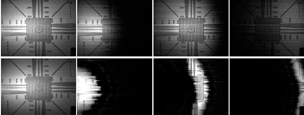
Figure 9. Comparison between original unprocessed SPAD data (Row 1) and the output of our proposed reconstruction procedure with the Poisson-VBM3D prior (Row 2). Column 1: Regular image of the scene under laser illumination. Column 2-4: Frames of the scene at different instance in time in response to a pulse of light. Our reconstructed frames show a sharp wavefront and significantly less noise when compared to the unprocessed frames.
