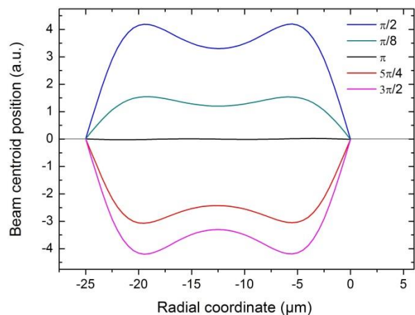
Fig. 9. Simulated peak heights for different phase shifts. (NB: the peaks look wide only due to the chosen range of interest, since the wavefront is flat on each side of the peaks)
