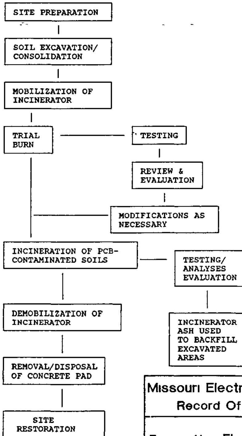
Figure 11 - Flow Diagram of PCB-Contaminated Soils- Remedial Action
