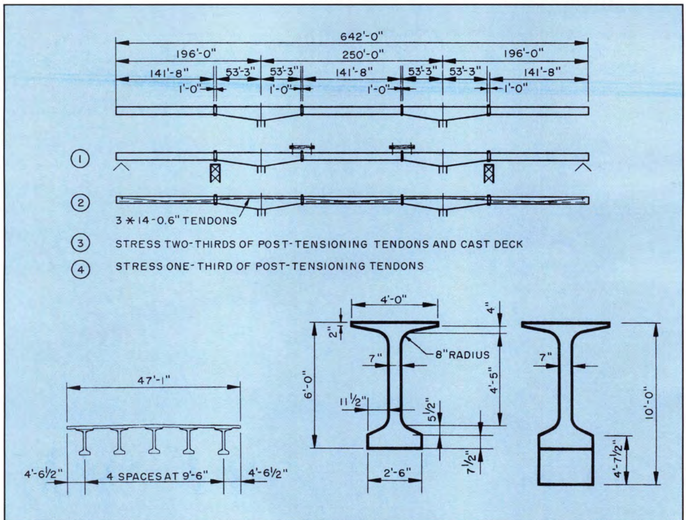
Fig. 4. Elevation of three-span section, erection steps, deck section and cross-sectional dimensions of bulb-tee girders.
