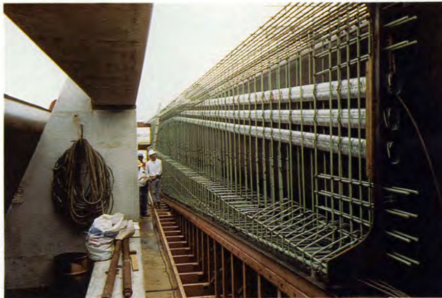
Fig. 7. Forms, post-tensioning ducts and mild steel reinforcement used in casting haunched girder section.
