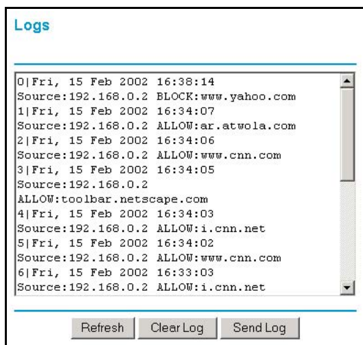
Figure 5-5: Logs menu
