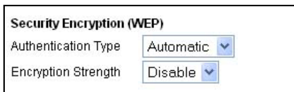
Figure 4-3: Encryption Strength
