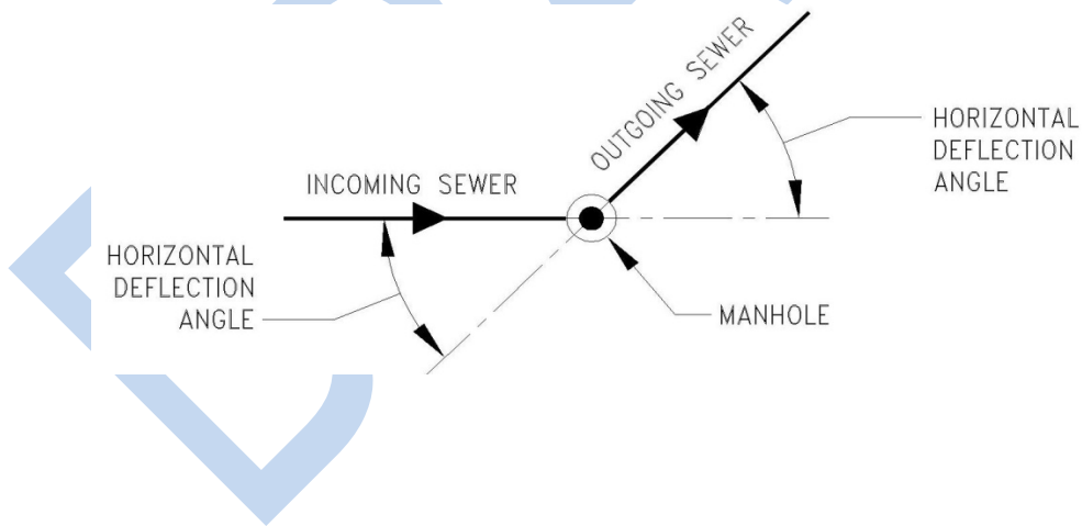
Figure 5.1 Horizontal Deflection Angles (Plan View)
