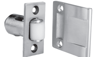
1898 Extended Cast Strike = 2-1/8" x 2-1/4" Roller latch face = 1-1/8" x 2-1/4" Maximum roller projection = 1/2"
