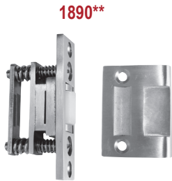
1890** Cast Strike = 1-11/16" x 2-1/4" Roller latch face = 1" x 3-3/8" Maximum roller projection = 5/16"
