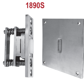
1890S Custom Strike = Contact factory Roller latch face = 1" x 3-3/8" Maximum roller projection = 5/16"
