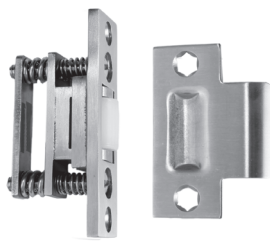
1892 T-Strike = 1-3/8" (lip to center) x 2-3/4" Roller latch face = 1" x 3-3/8" Maximum roller projection = 5/16"
