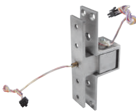
Electrified Pocket Pivot (EZ Connect shown)
