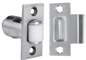
1895 T-Strike = 1-3/8" (lip to center) x 2-3/4" Roller latch face = 1-1/8" x 2-1/4" Maximum roller projection = 1/2"
