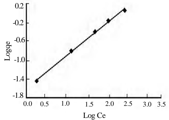
Fig. 10. Freundlich Adsorption Isotherm for As(III) adsorption onto silica ceramic at different initial concentration
