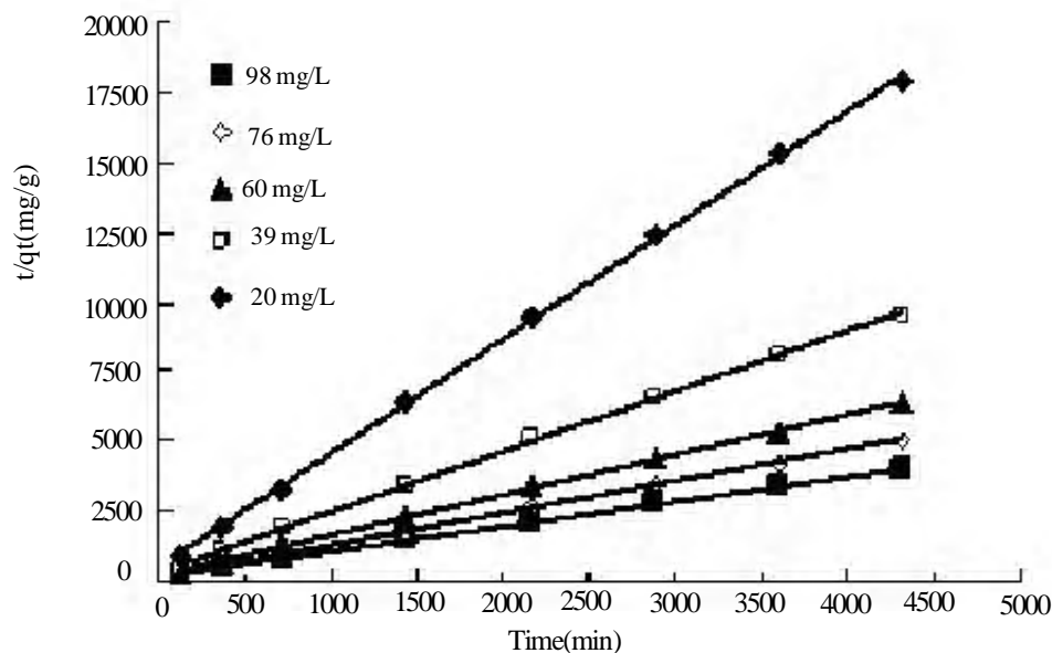
Fig. 5. Pseudo-second order kinetics for adsorption of As(III) onto silica ceramic at different initial As(III) concentration (pH 7.5, adsorbent dose 80 g/L and temperature 25°C)
