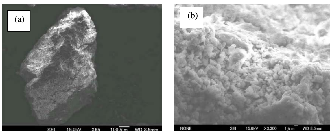
Fig. 1. SEM Photograph of silica ceramic: (a) general intra structure (× 65, 100μm) and (b) intra structure (× 3500, 1μm)
