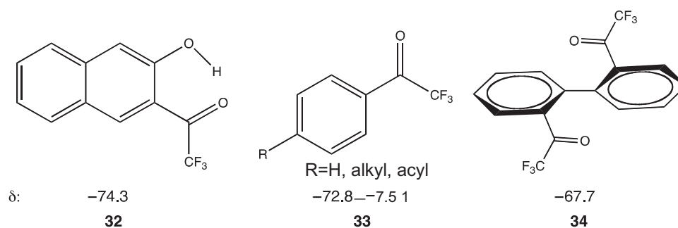
Figure 13 Trifluoroacetylated aromatics.
