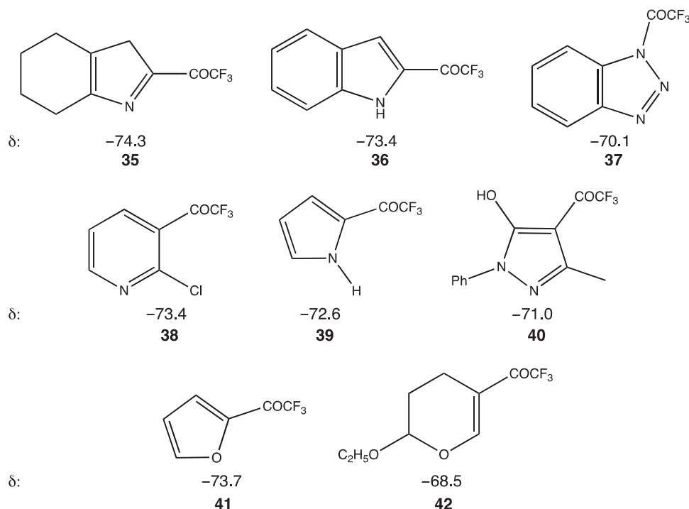
Figure 14 Trifluoroacetylated heterocycles.
