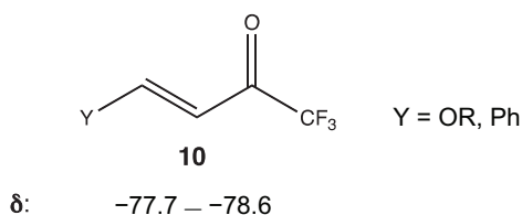
Figure 7 \alpha,\beta -Unsaturated trifluoromethyl ketones. Abbreviations: \text{CF}_3 , trifluoromethyl; OR, alkoxy; Ph, phenyl.
