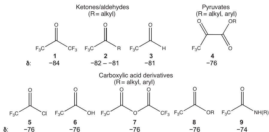
Figure 6 Isolated \alpha,\alpha,\alpha -trifluorocarbonyl species. Abbreviations: \text{CF}_3 , trifluoromethyl; R, alkyl, aryl.
