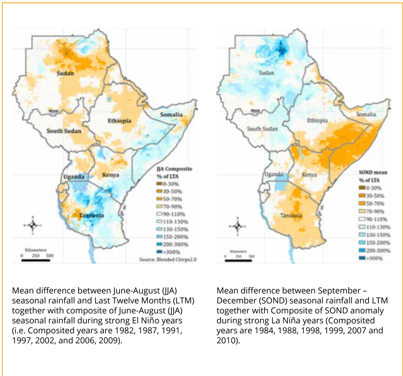
Figure 1: Rainfall variability during strong La Niña and El Niño years
