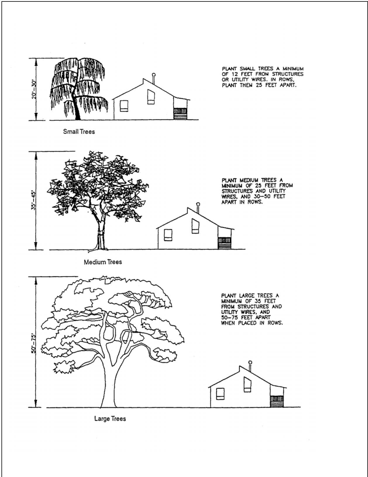
Plate 6.80b Spacing Trees for Safety and Effective Landscaping Source: Virginia DSWC
