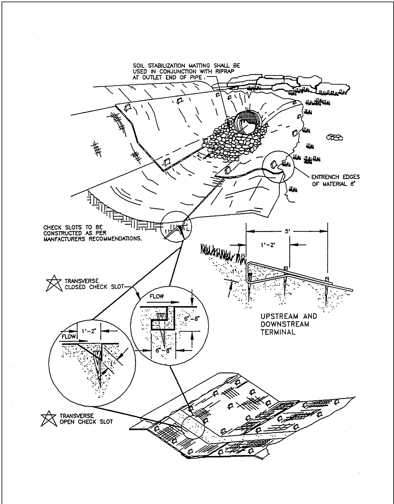
Plate 6.75f Typical Treatment 2 - Soil Stabilization Matting Installation
