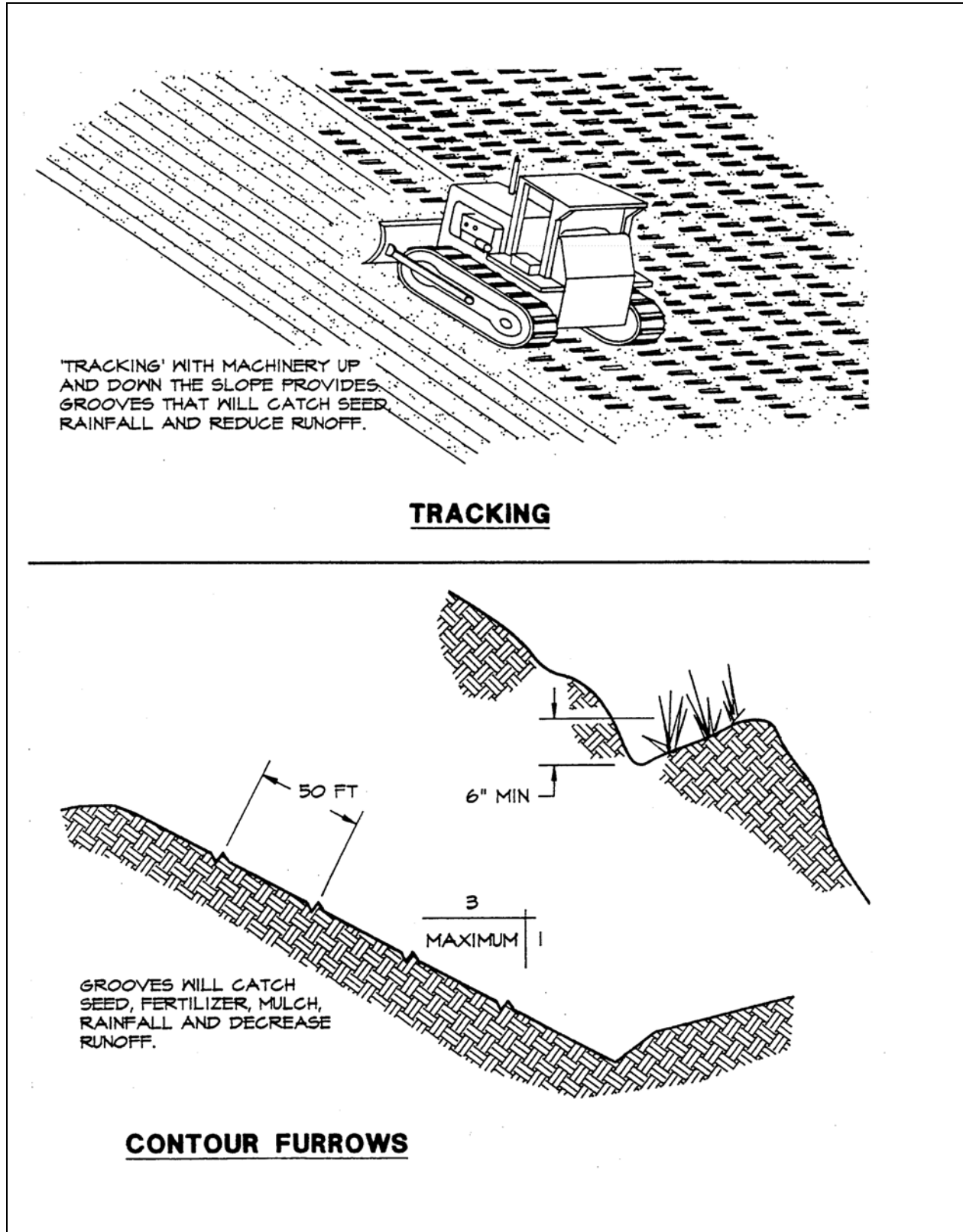
Plate 6.60d Roughening with Tracked Machinery Source: Erosion Draw
