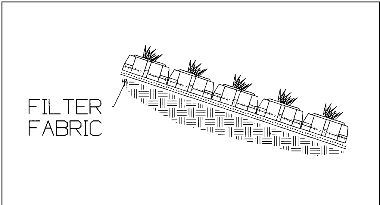
Plate 5.18c Revegetation Source: NRCS
