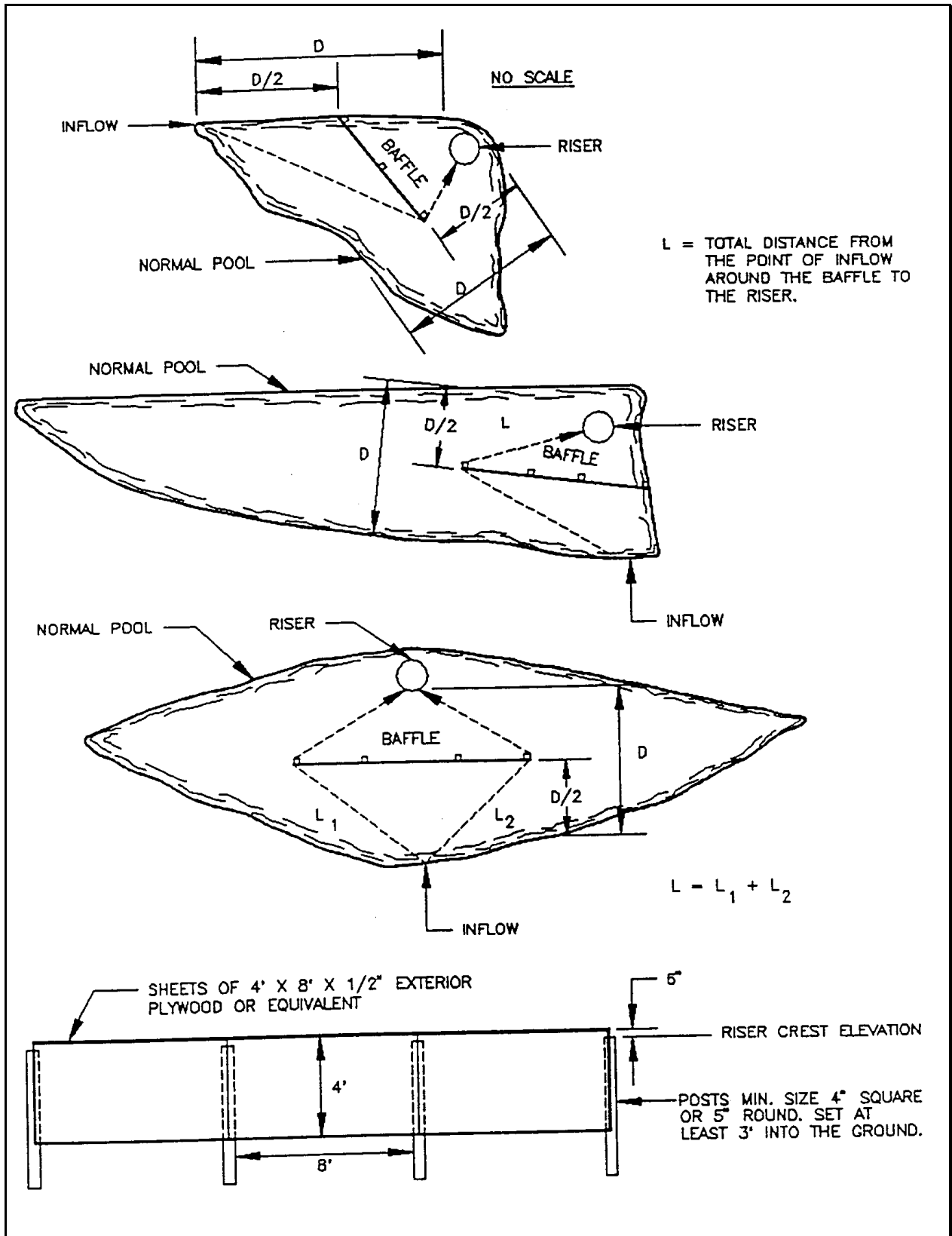
Plate 4.26h Example Plan Views of Baffle Locations in Sediment Basins
