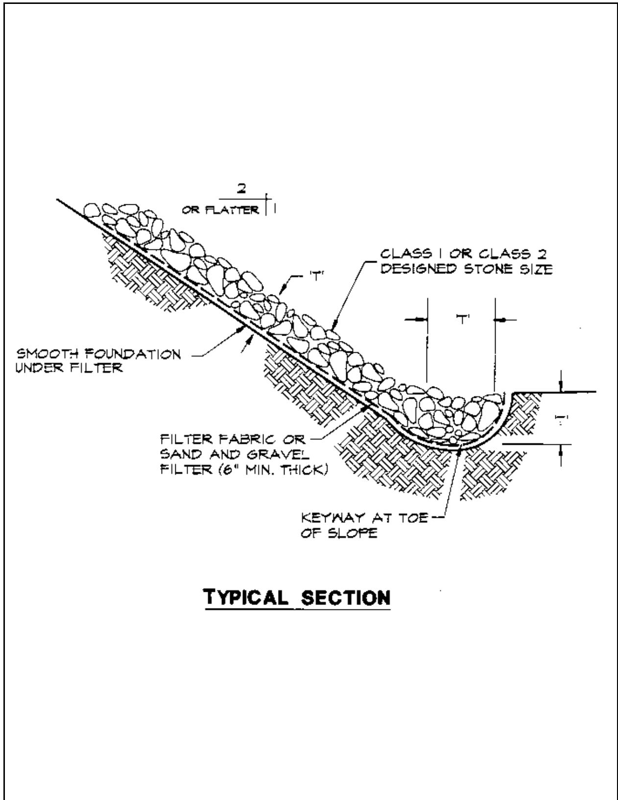
Plate 5.16b Riprap Slope Protection Source: Erosion Draw
