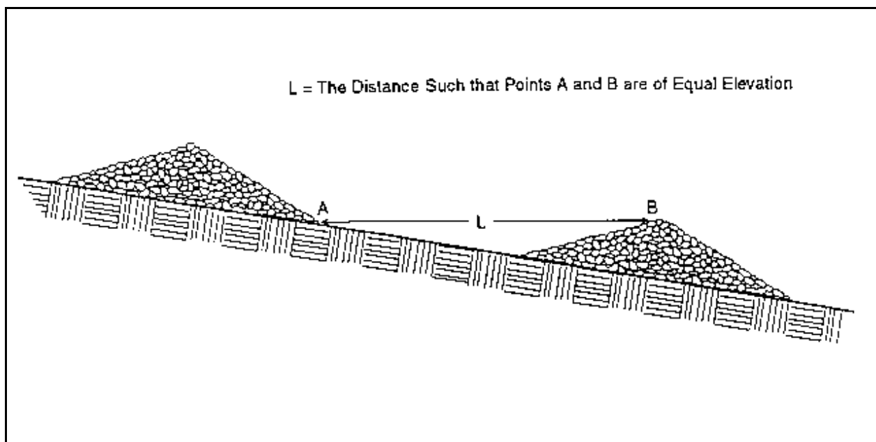
Plate 5.12c Spacing Between Check Dams
