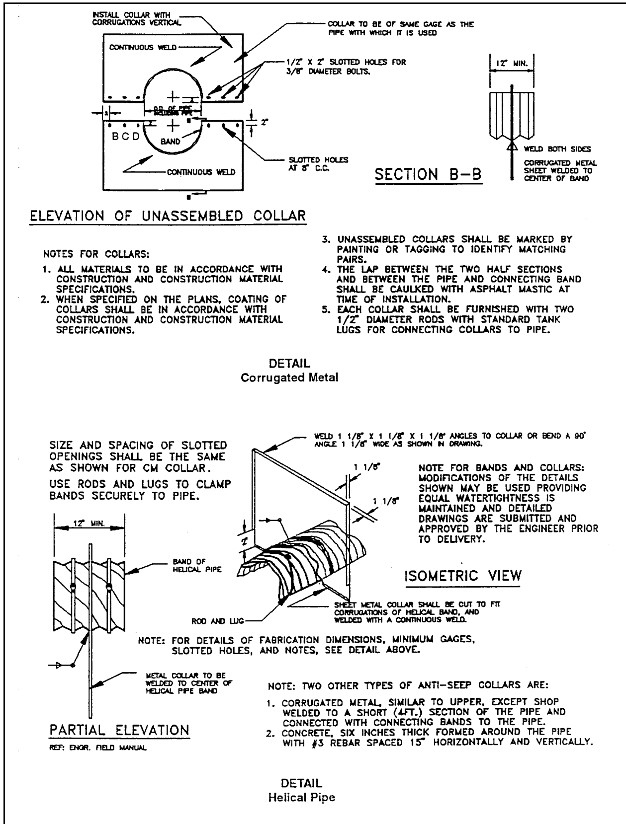
Plate 4.26L Anti-seep Collar Details
