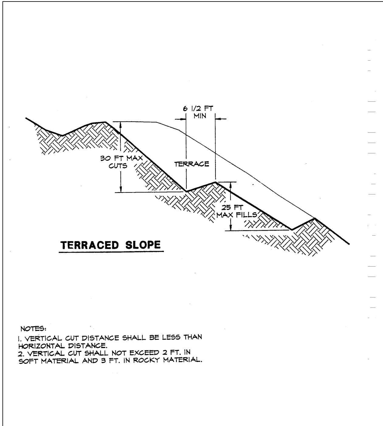
Plate 6.60c Terraced Slope Source: Erosion Draw
