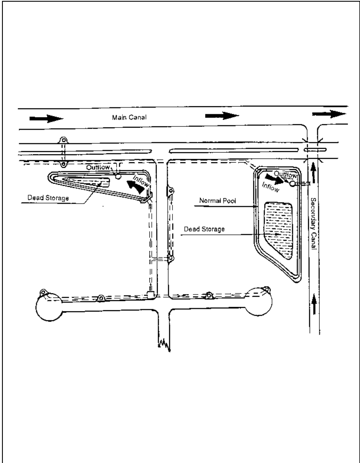
Plate 5.05b Examples of Dead Storage Areas in Wet Ponds Source: NRCS
