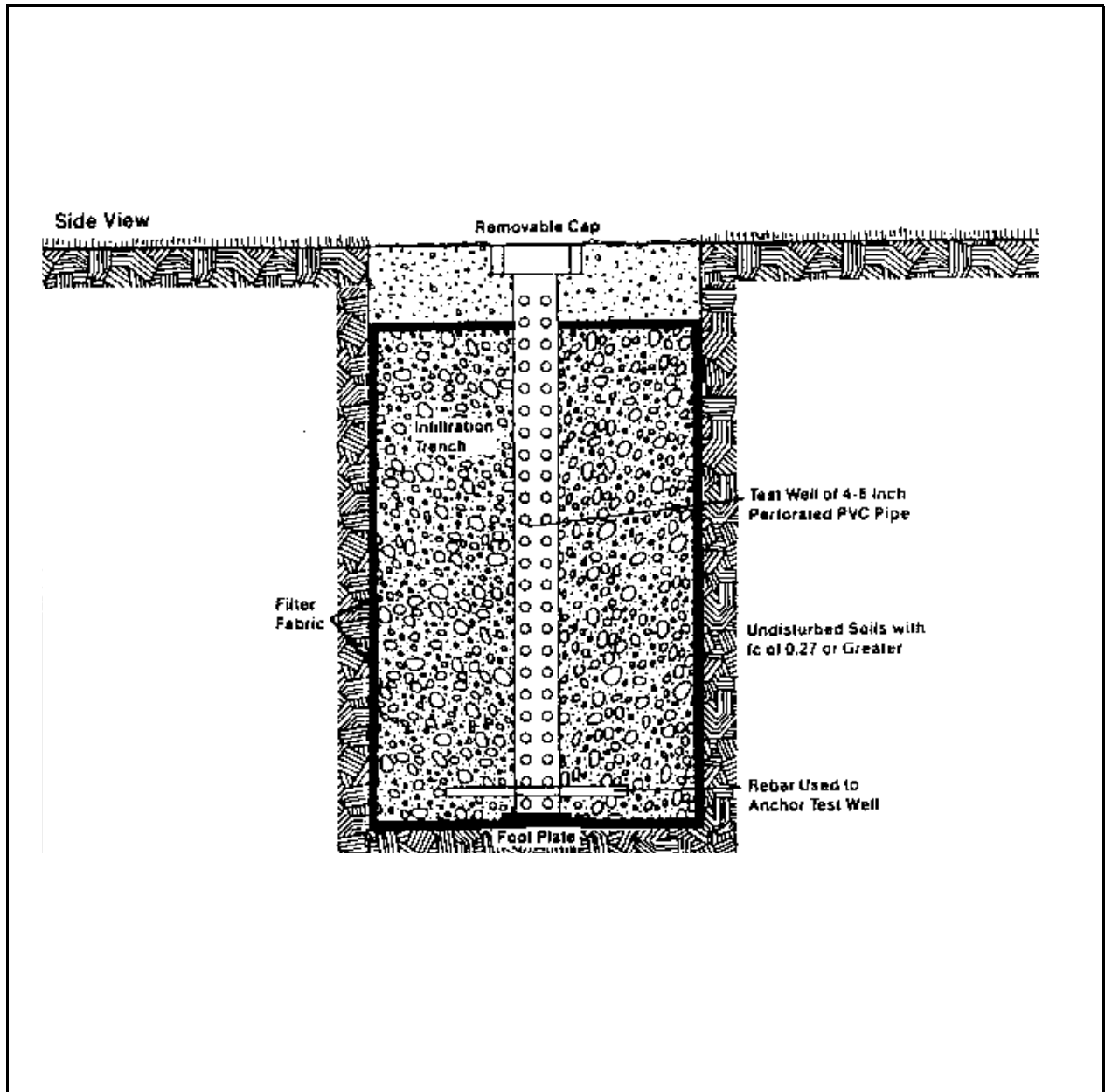
Plate 5.02e Detailed Schematic of a Typical Observation Well Source: Schueler (1987).
