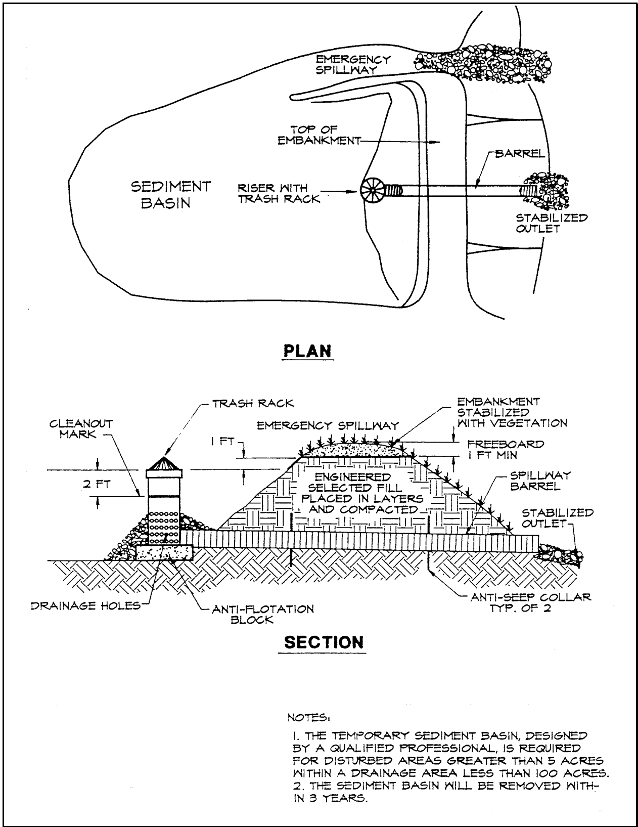
Plate 4.26g Sediment Basin
