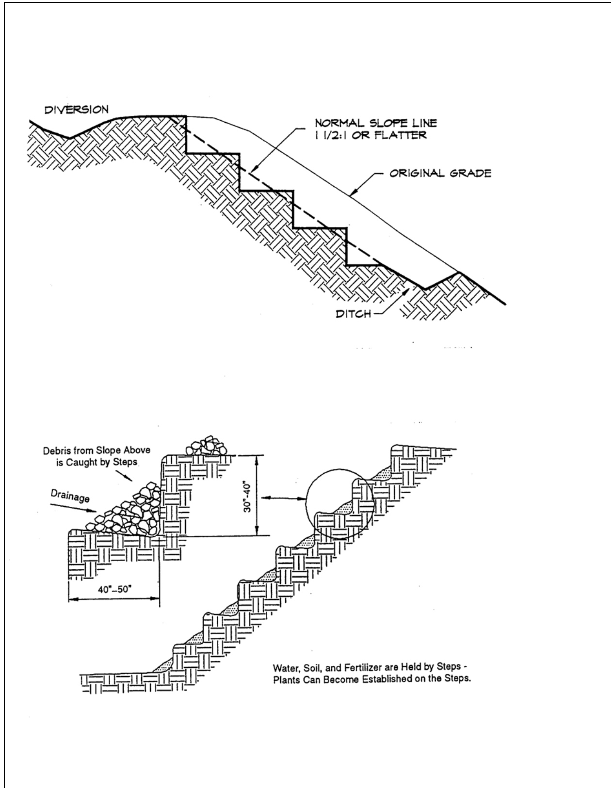
Plate 6.60a Stair Stepped Slope Source: Virginia DSWC, Erosion Draw
