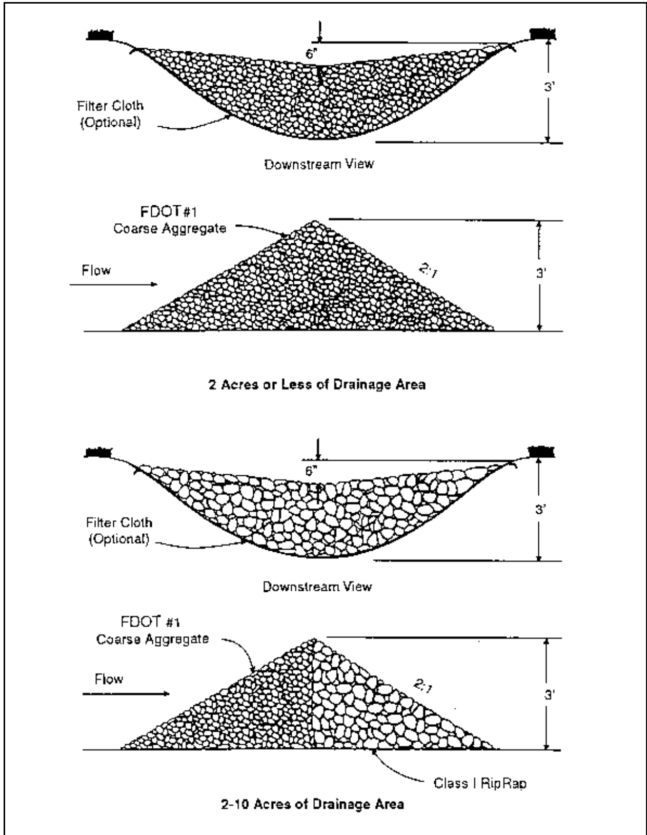
Plate 5.12b Rock Check Dam Source: Virginia DSWC
