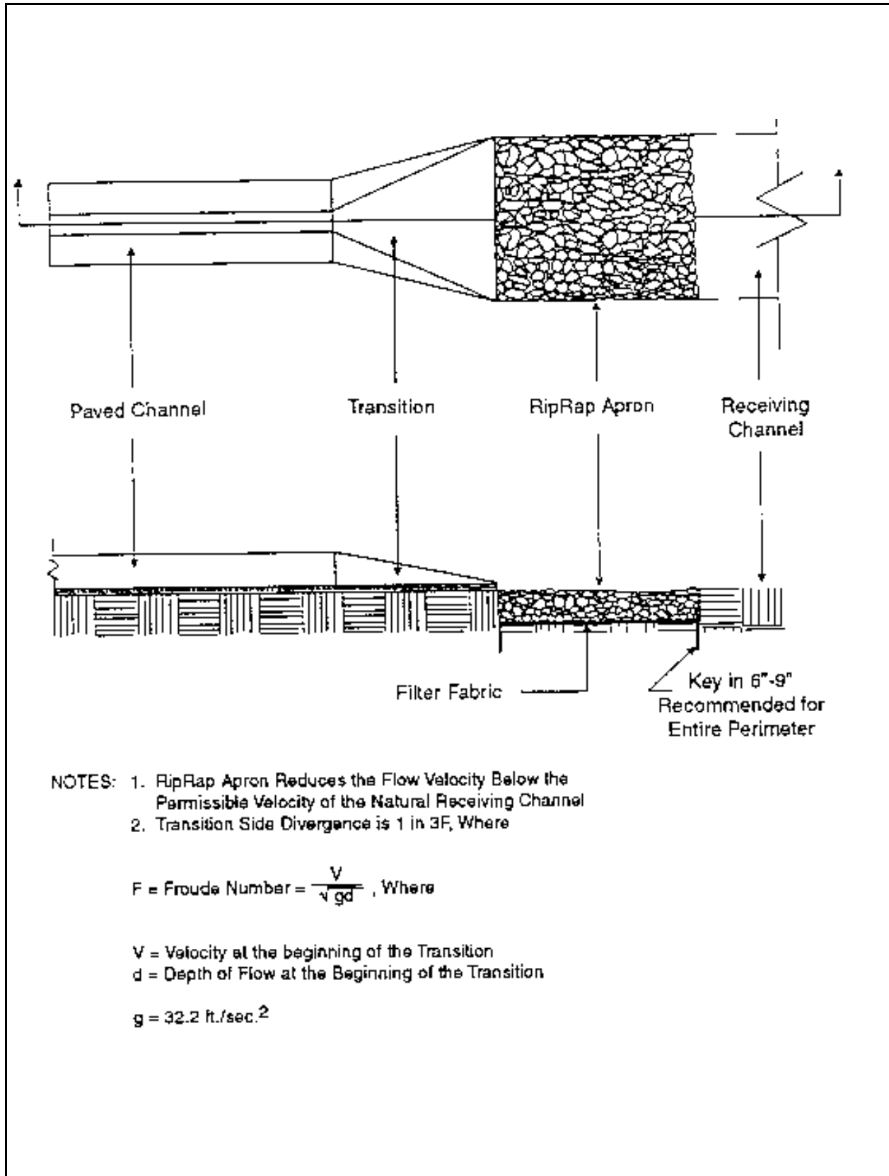
Plate 5.15d Paved Channel Outlet
