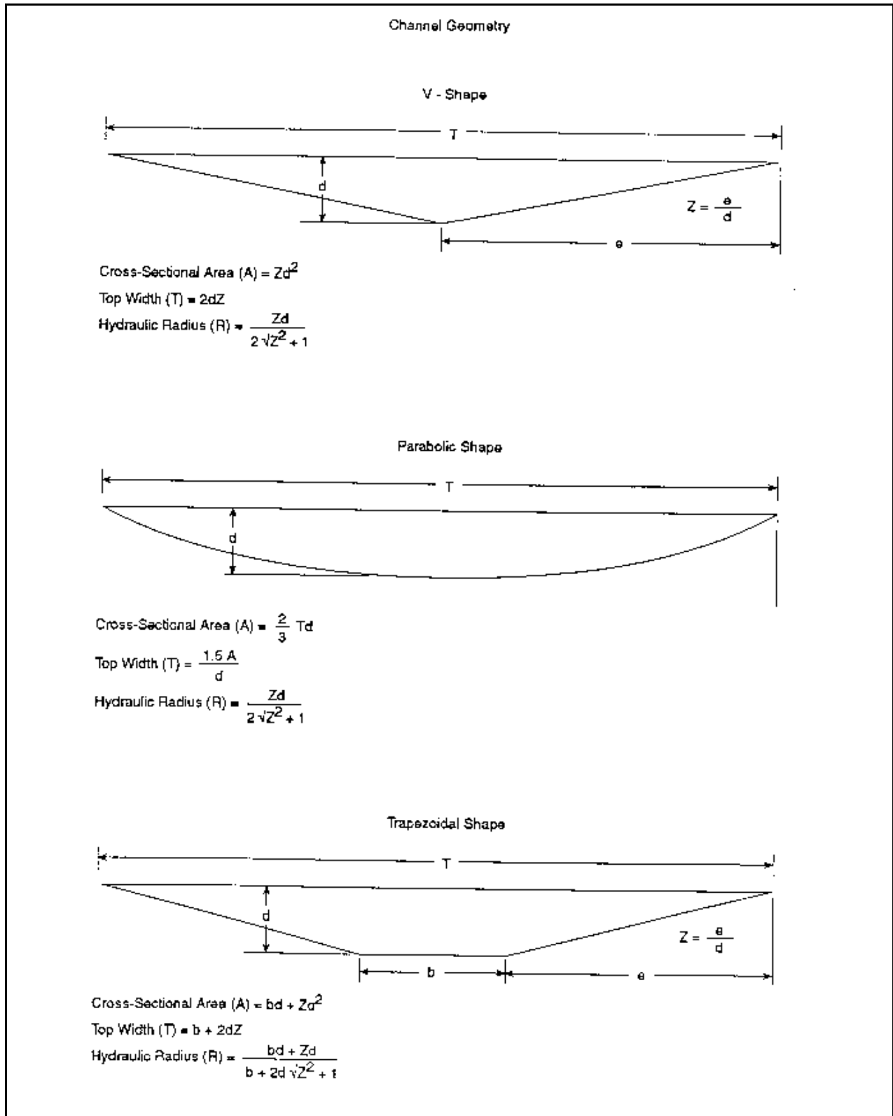
Plate 5.07a Typical Waterway Shapes and Mathematical Expressions for Calculating Cross-Sectional Area, Top Width, and Hydraulic Radius
