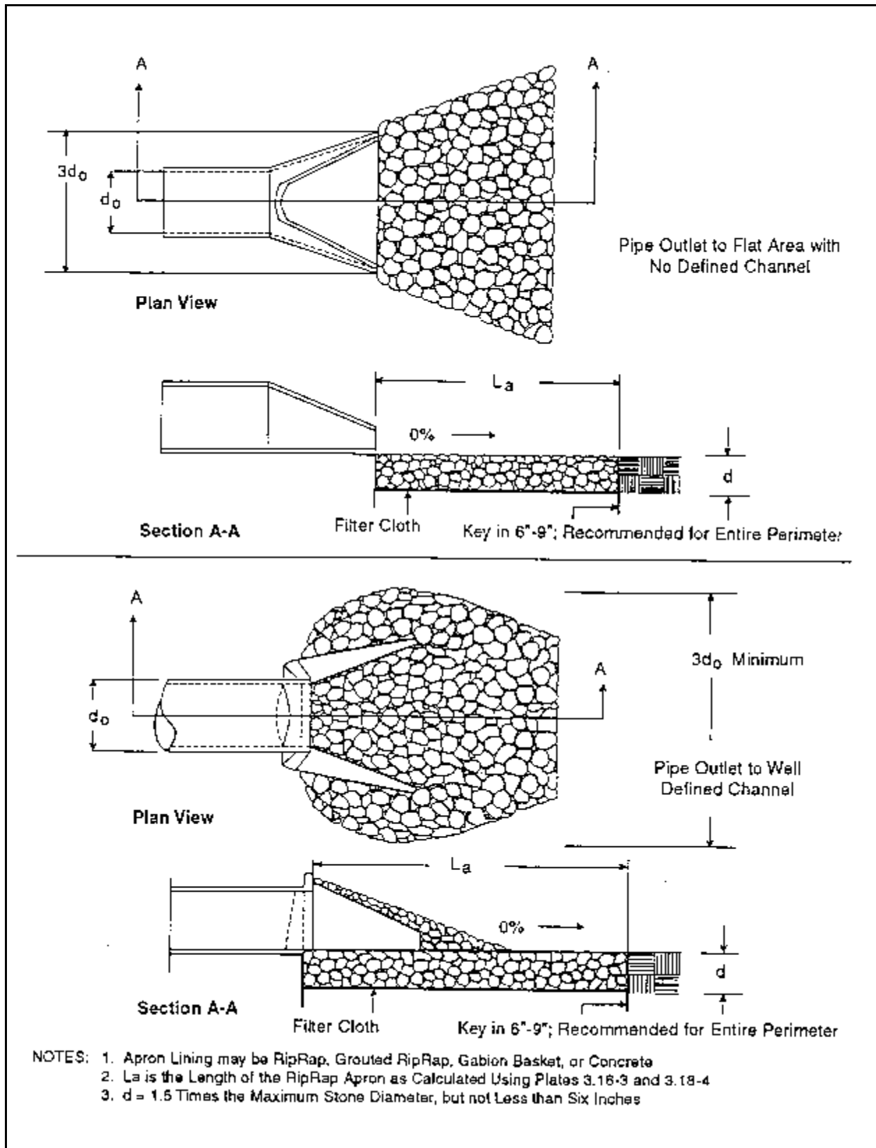
Plate 5.15c Pipe Outlet Conditions
