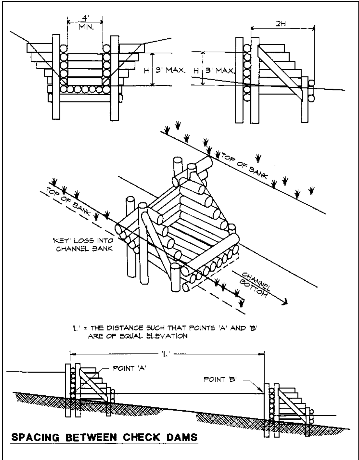
Plate 5.14b Log Grade Stabilization Structure
