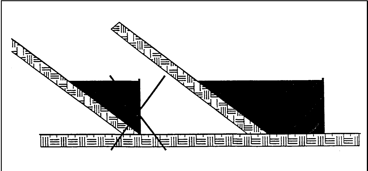
Plate 4.06f Proper Placement of a Silt Fence at the Toe of a Slope
