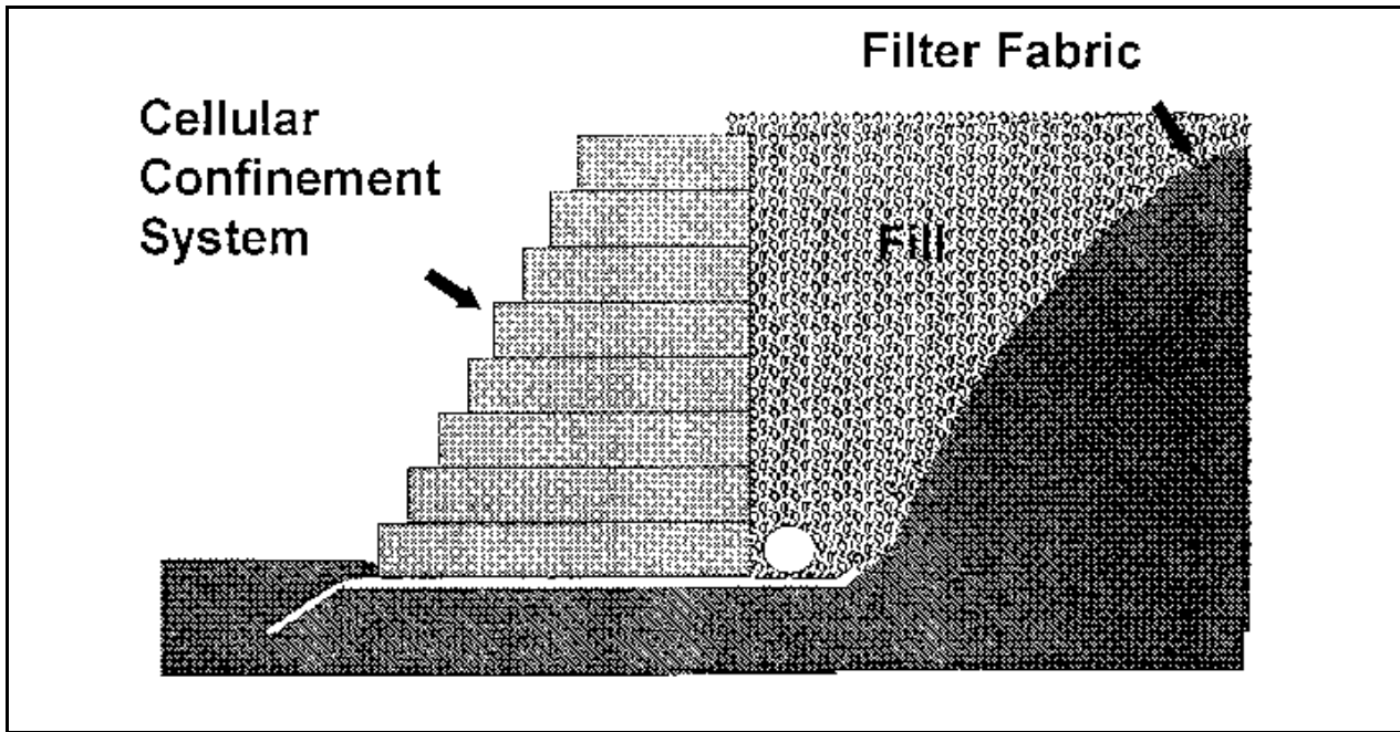
Plate 5.17d Gravity Retaining Wall Source: NRCS
