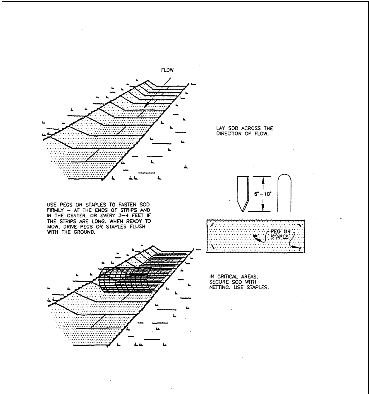
Plate 6.67b Sodding Swales and Waterways Source: Virginia DSWC
