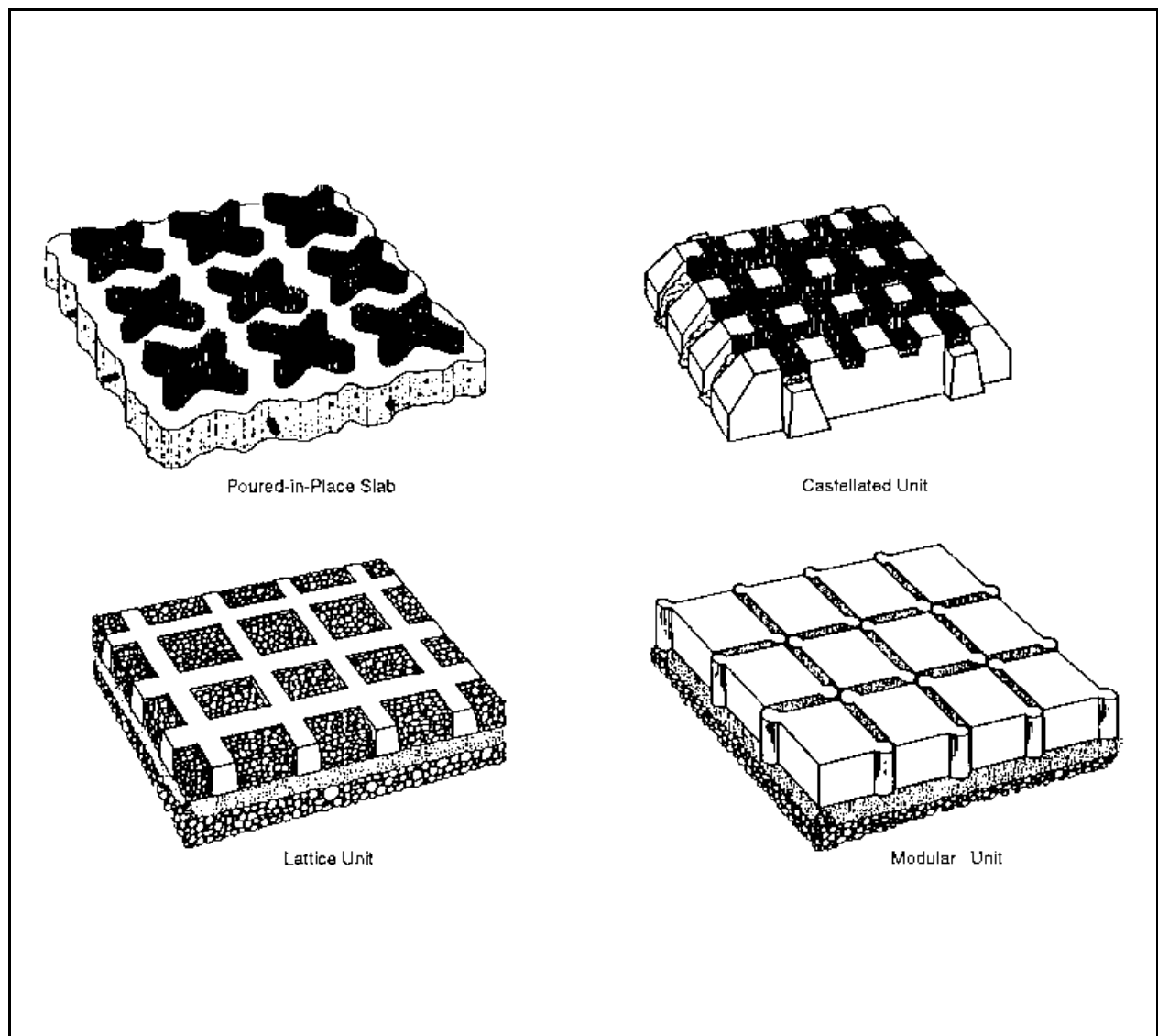
Plate 5.04a Types of Grid and Modular Pavement
