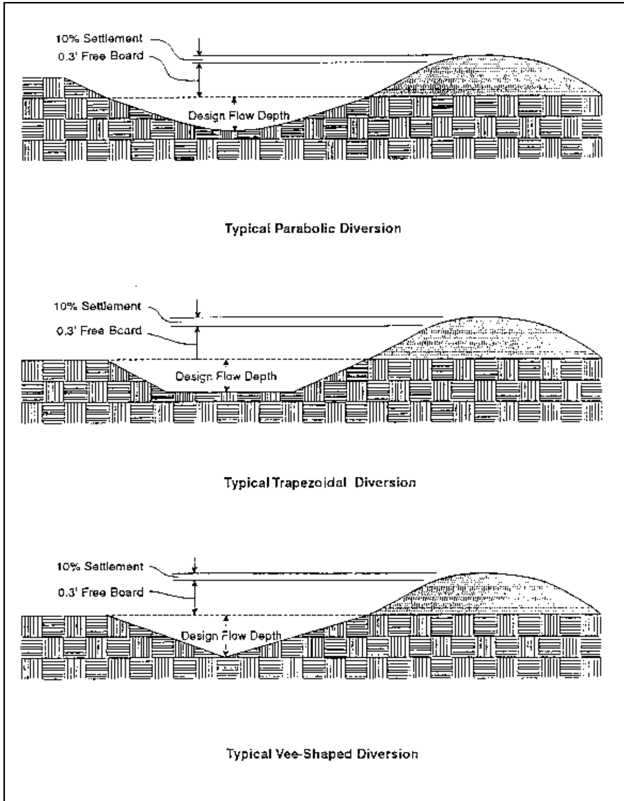
Plate 5.10a Diversions Source: Virginia DSWC
