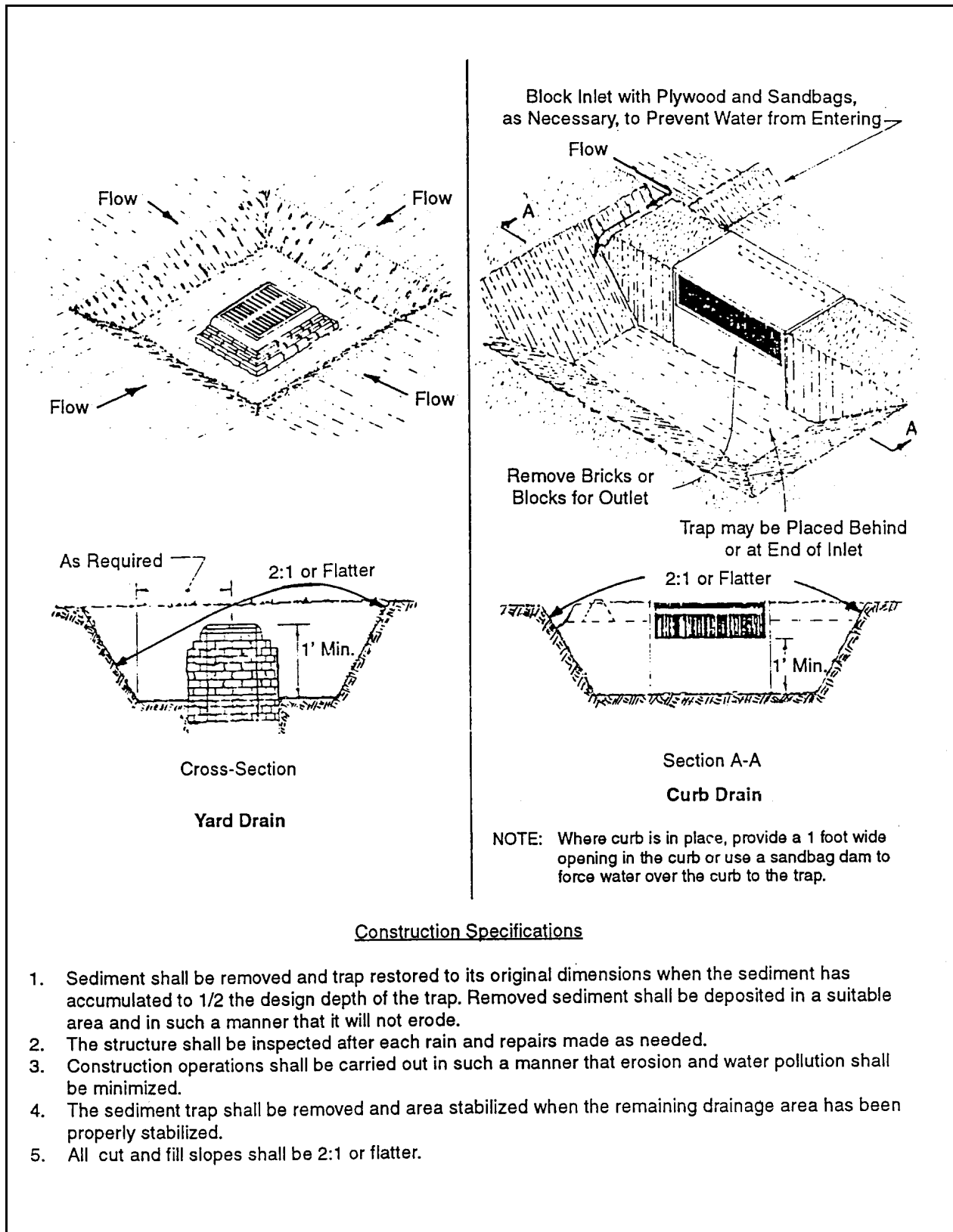
Plate 4.25f Storm Inlet Sediment Trap
