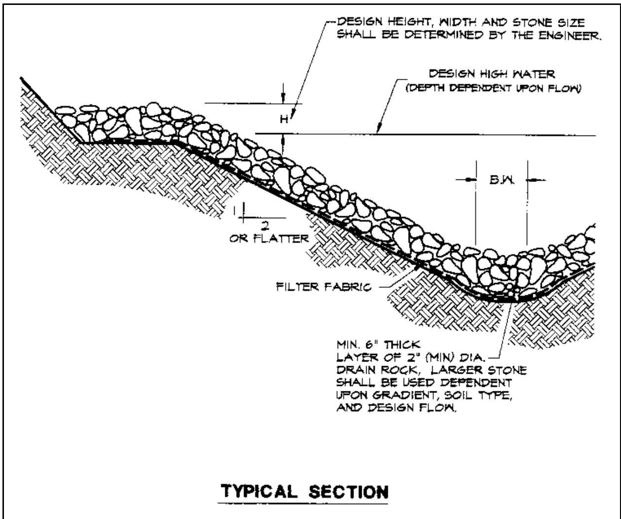
Plate 5.16a Rock-Lined Channel
