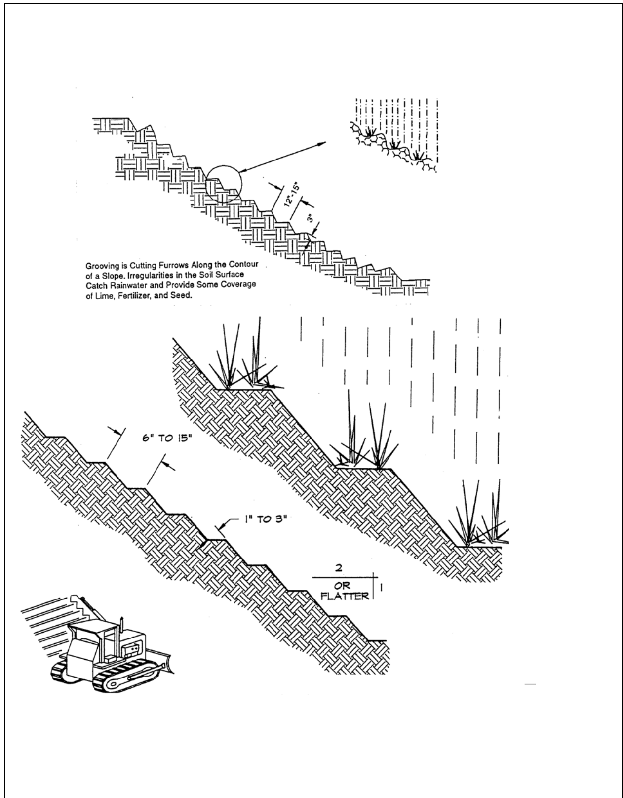
Plate 6.60b Grooved or Serrated Slope
