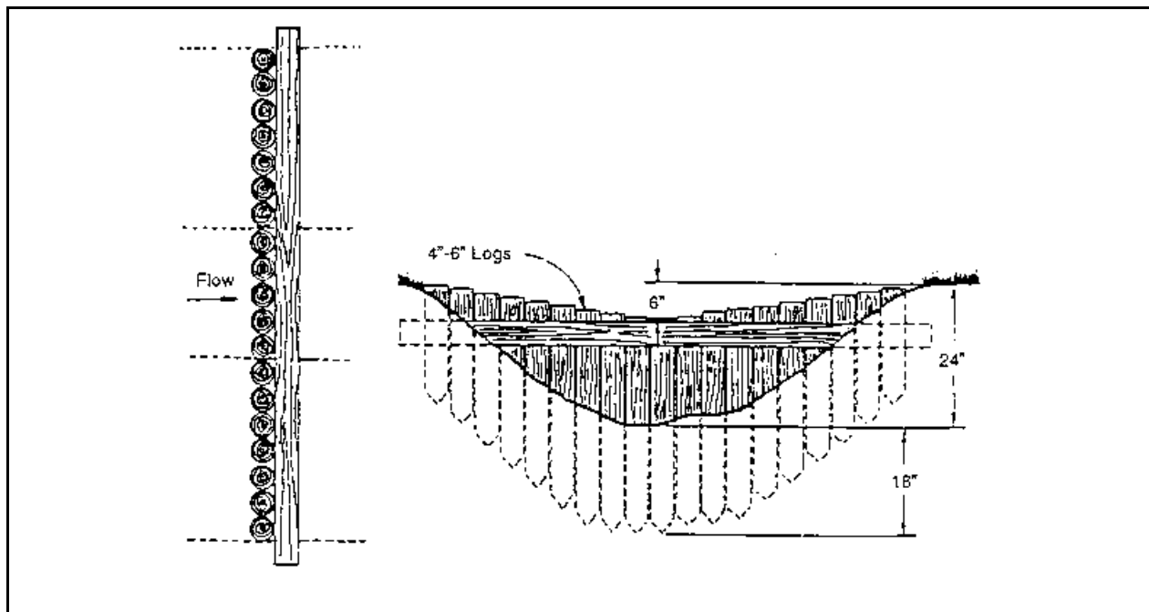
Plate 5.12a Log Check Dam Source: Virginia SWCC
