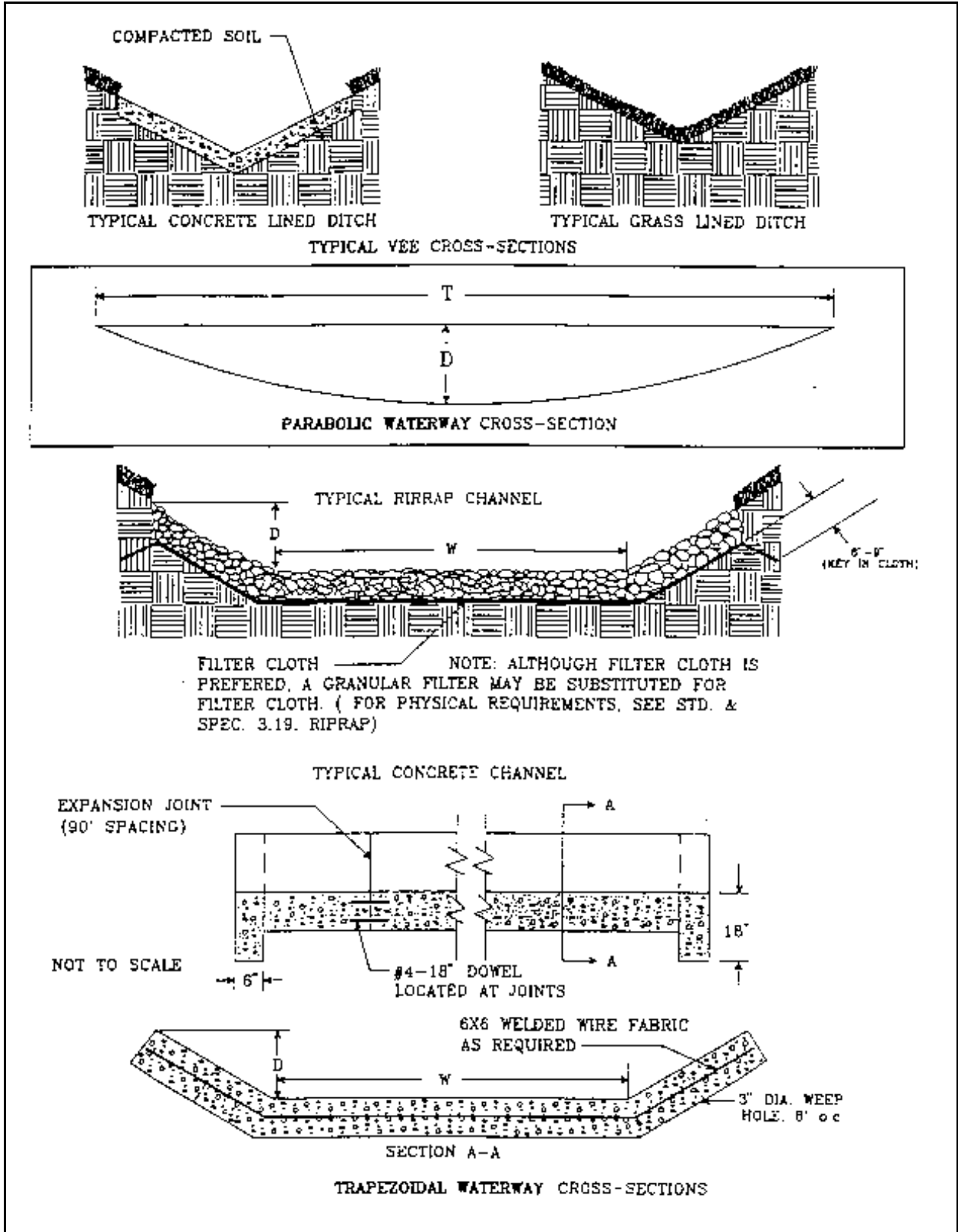
Plate 5.08a Typical Waterway Cross-Sections Source: Virginia DSWC
