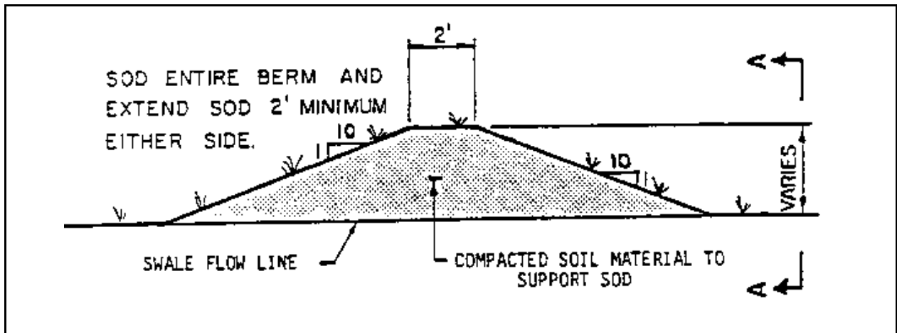
Plate 5.07b Typical Swale Block Cross-Section
