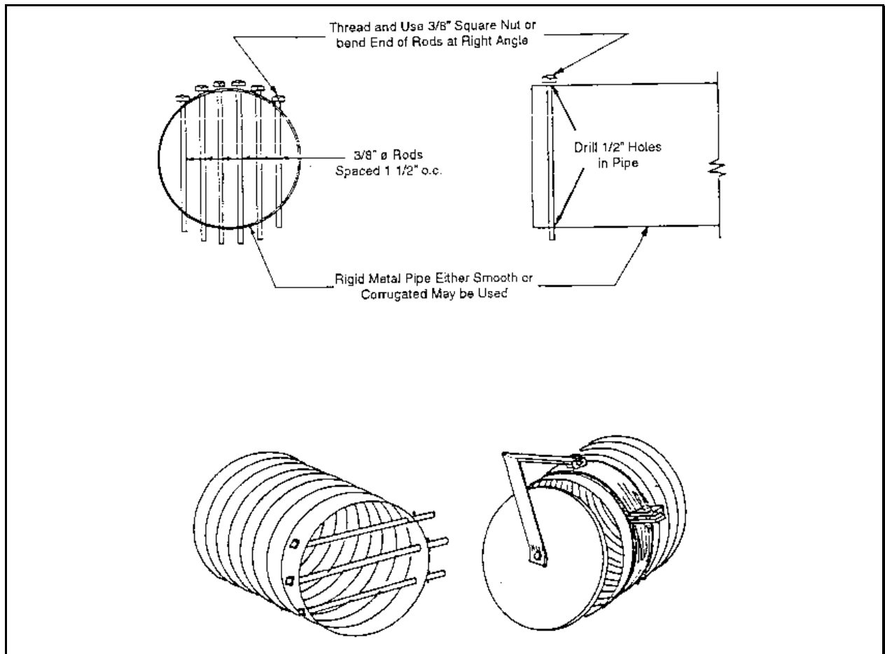
Plate 5.06i Rodent Protection for Outlet Pipes
