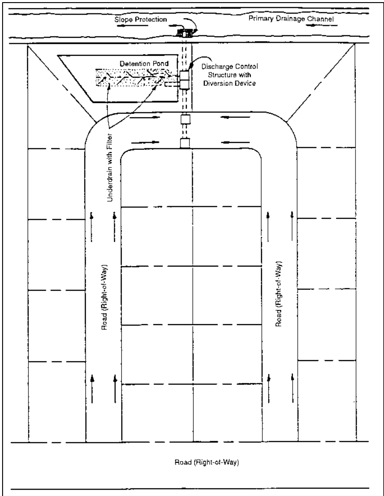
Plate 5.06f Typical Subdivision Layout Showing Off-Line Detention Pond and Outfall Source: Pinellas Park water Management District
