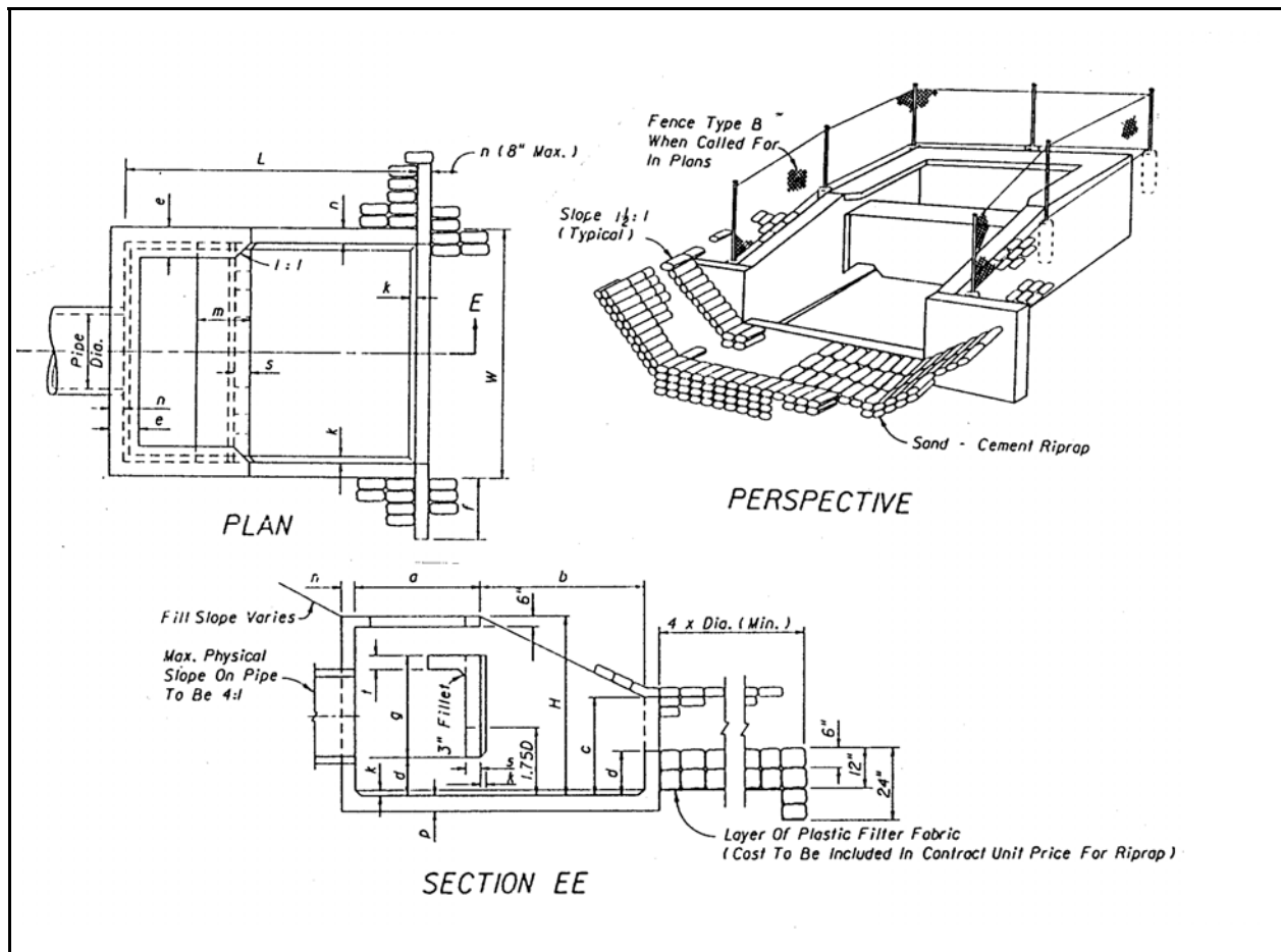
Plate 5.15a Energy Dissipator
