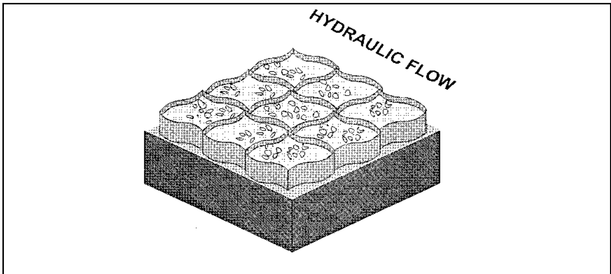
Plate 5.17a Grid Confinement System
