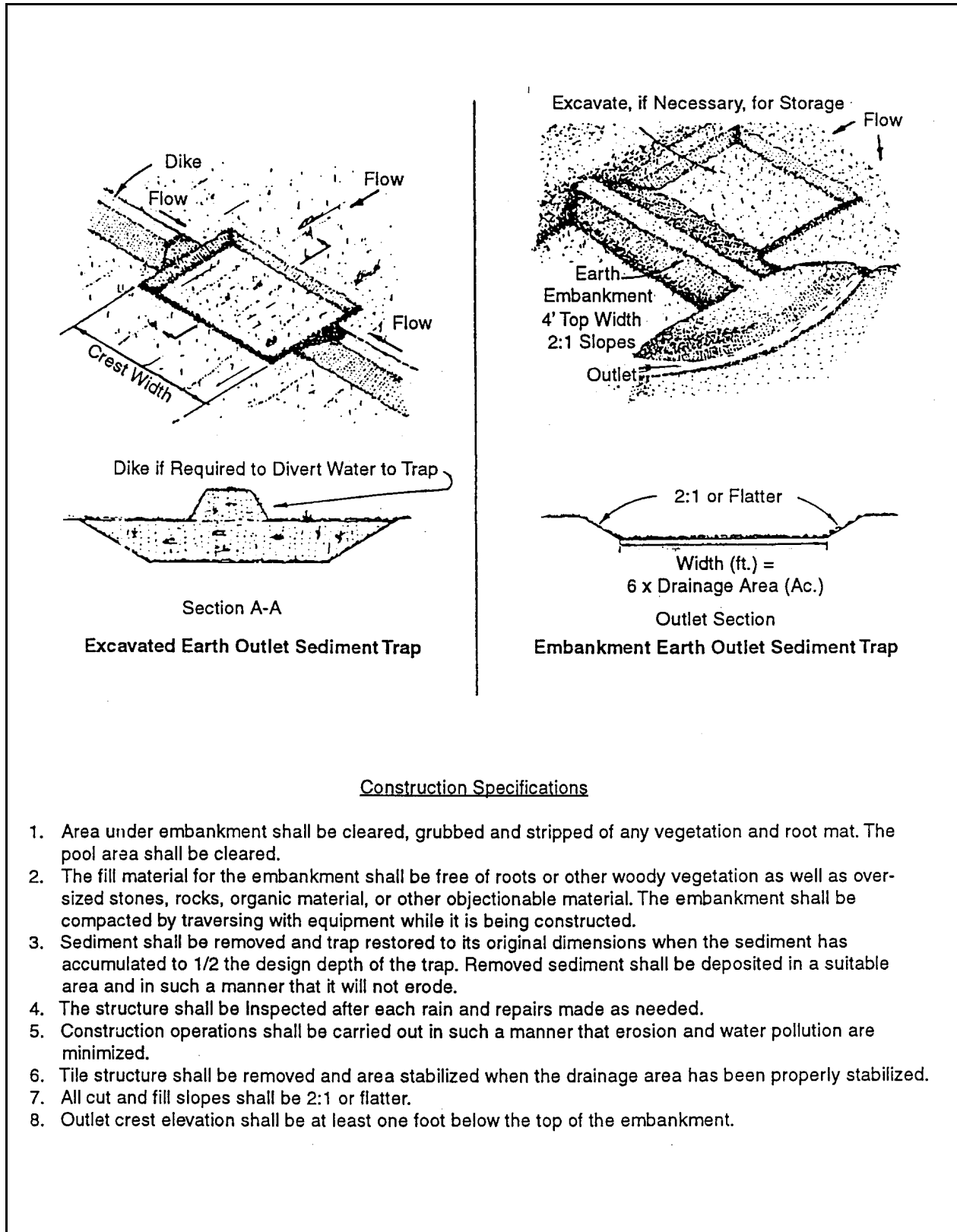
Plate 4.25a Earth Outlet Sediment Trap
