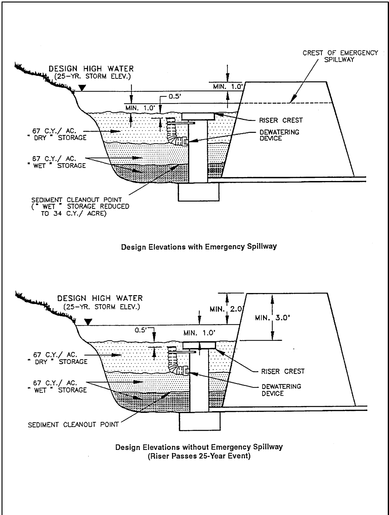
Plate 4.26b Sediment Basin Schematic Elevations
