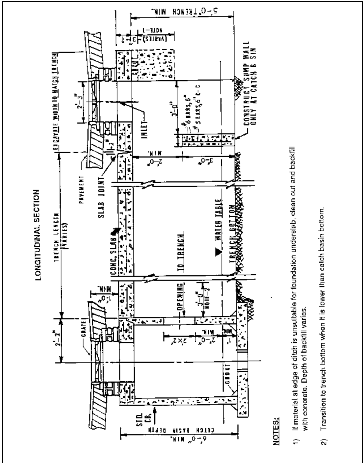
Plate 5.02b Typical Section, Slab Covered Trench, Dade County , Florida Source: NRCS
