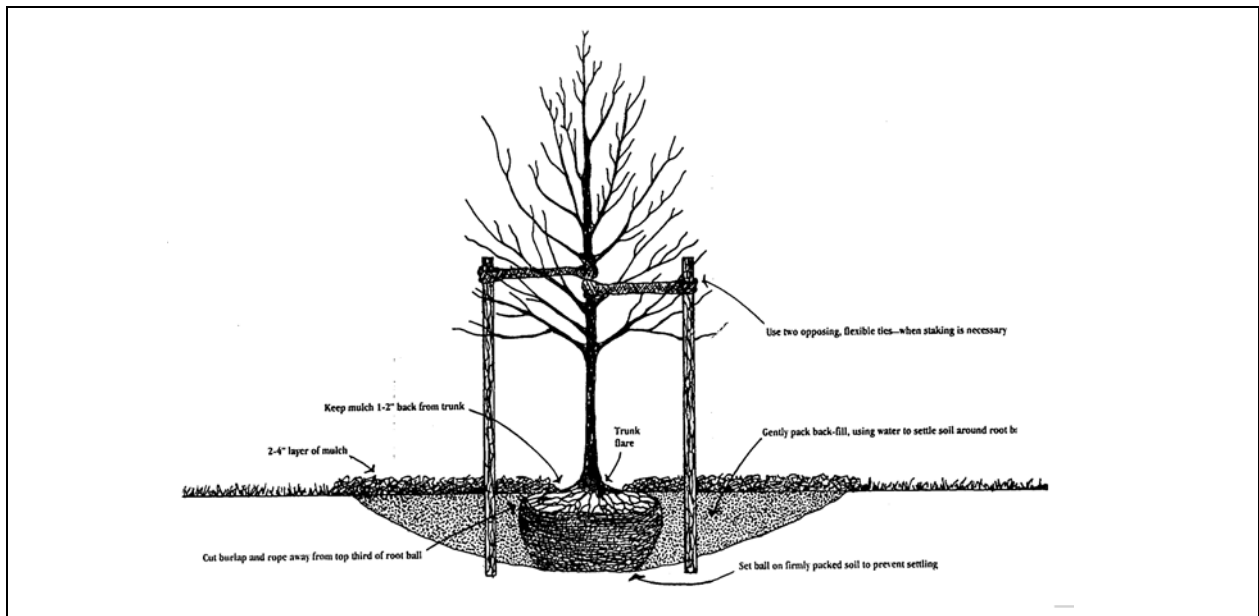
Plate 6.80d Planting Balled & Burlapped, and Container Grown Trees Source: International Society of Arboculture
