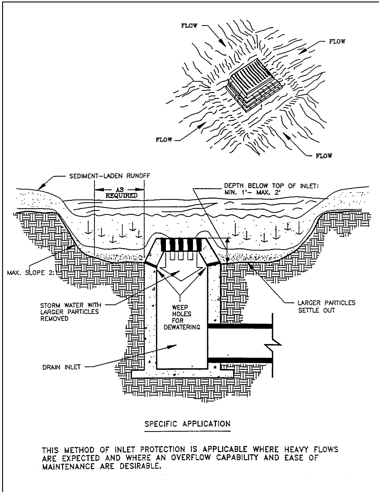
Plate 4.25e Excavated Drop Inlet Sediment Trap
