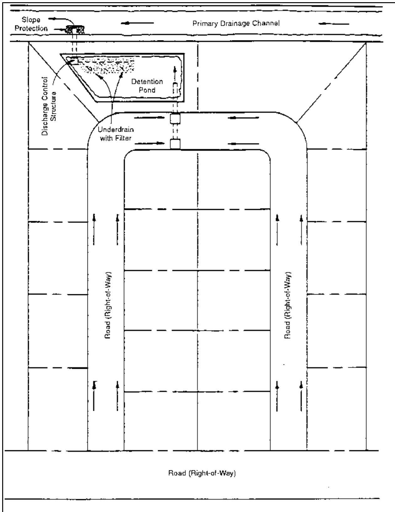
Plate 5.06d Typical Subdivision Layout Showing On-Line Detention Pond and Outfall Source: Pinellas Park Water Management District
