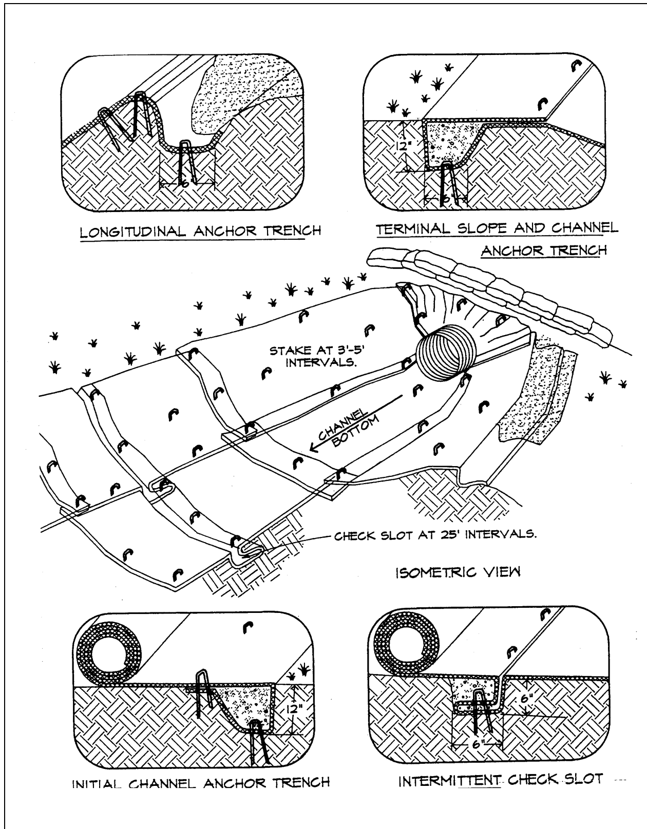
Plate 6.75e Erosion Blankets and Turf Reinforcement Mats - Channel Installation
