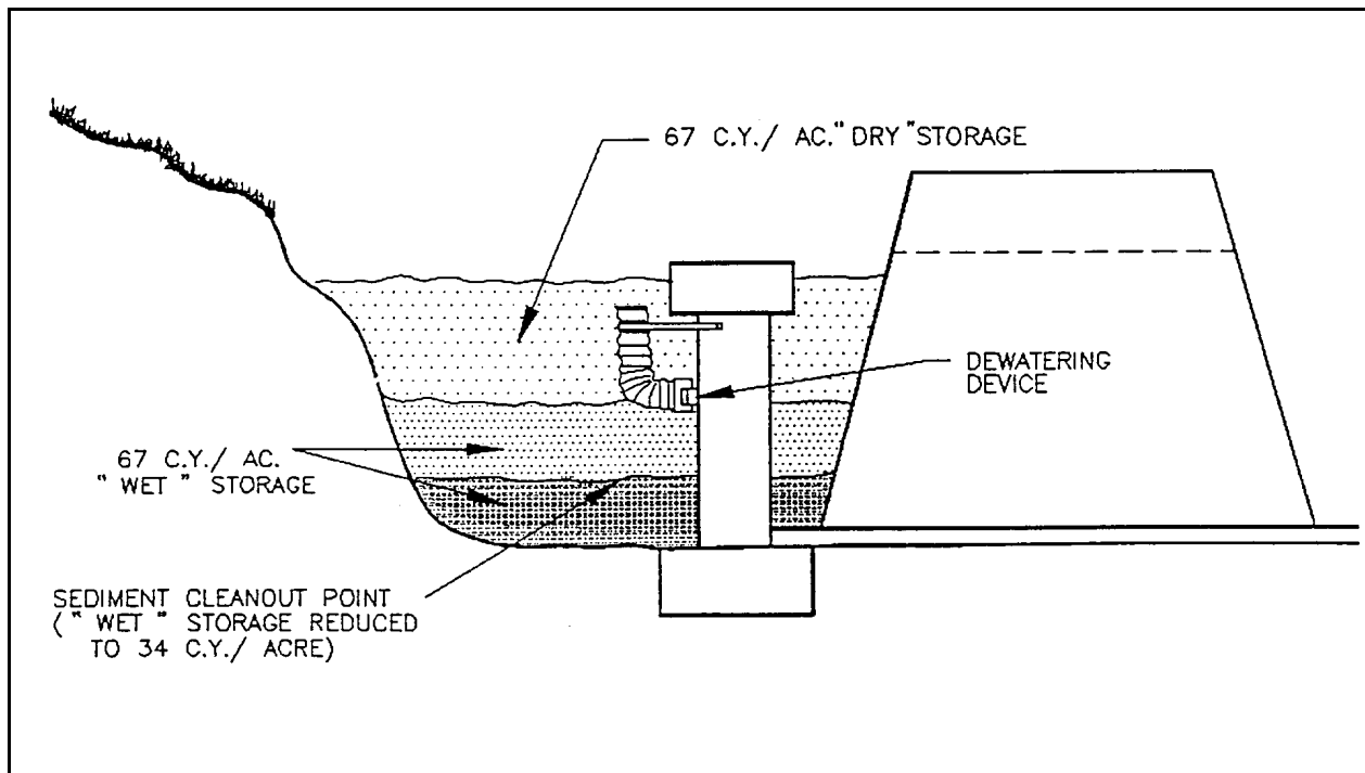
Plate 4.26a Sediment Basin Storage Volumes
