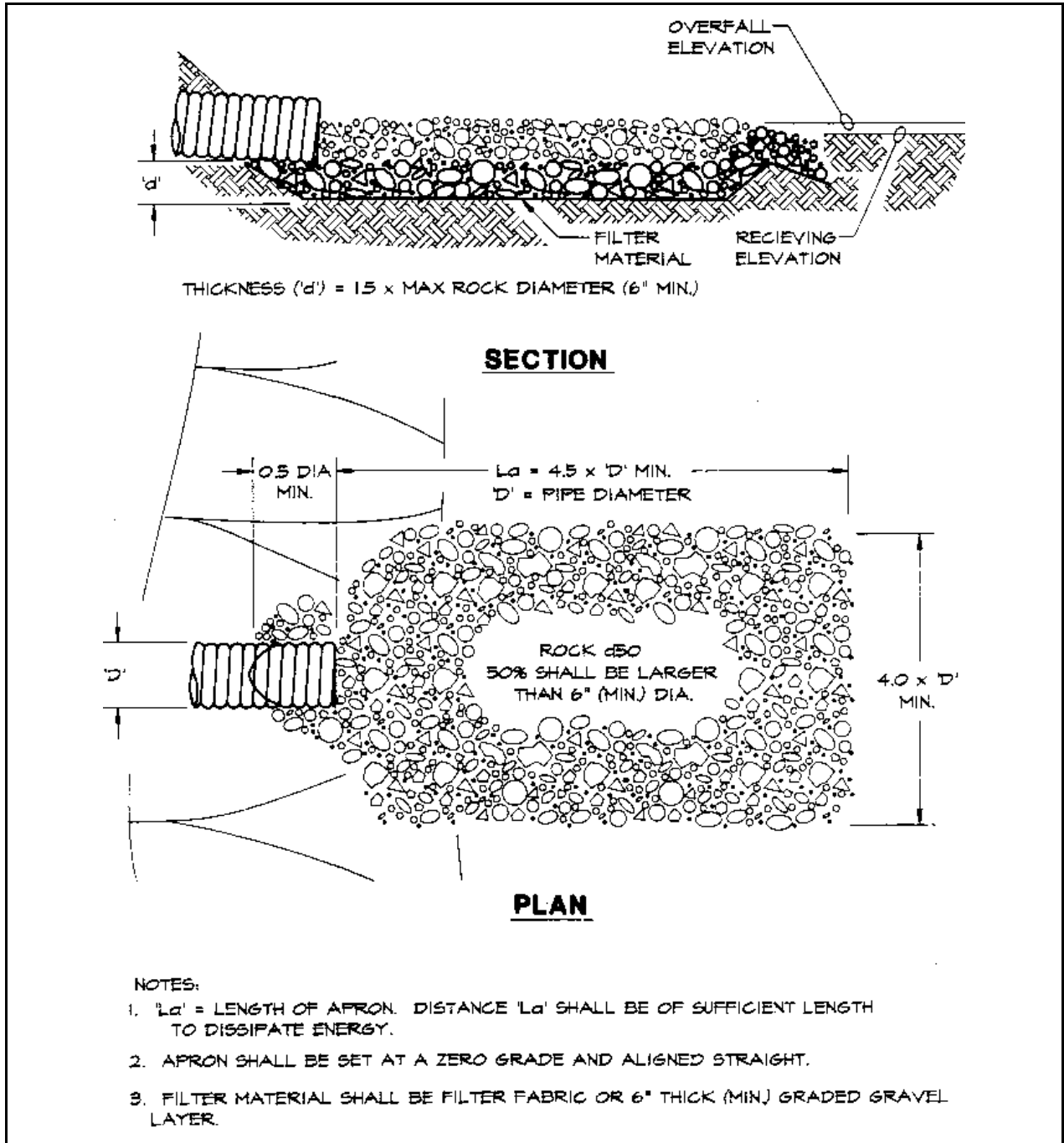
Plate 5.15b Energy Dissipator
