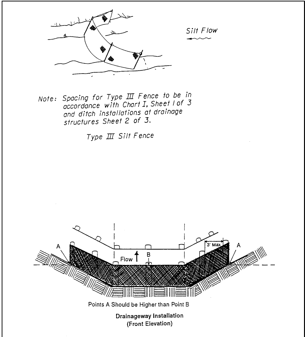
Plate 4.38d Silt Fence Check Dam
