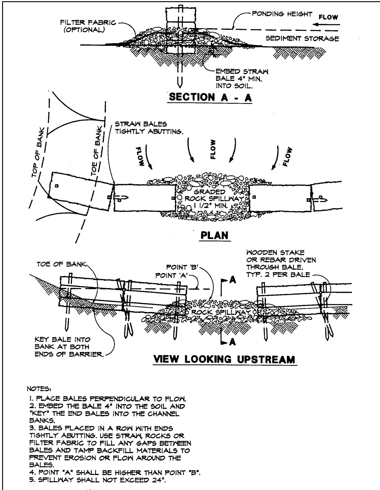
Plate 4.25d Semi-pervious Straw Bale Sediment Barrier Source: Erosion Draw
