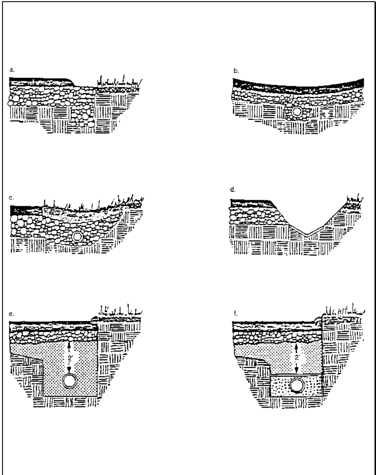
Plate 5.03a Examples of Porous Pavement Drainage Systems
