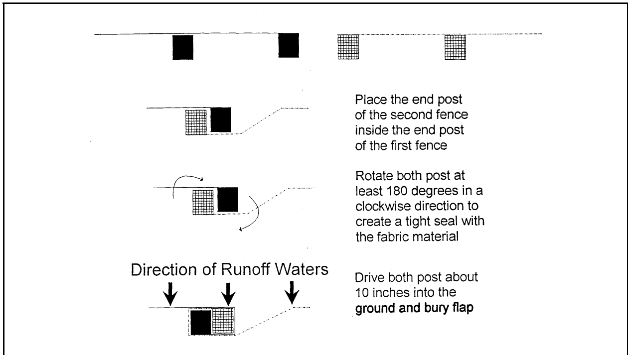
Plate 4.06g Attaching Two Silt Fences
