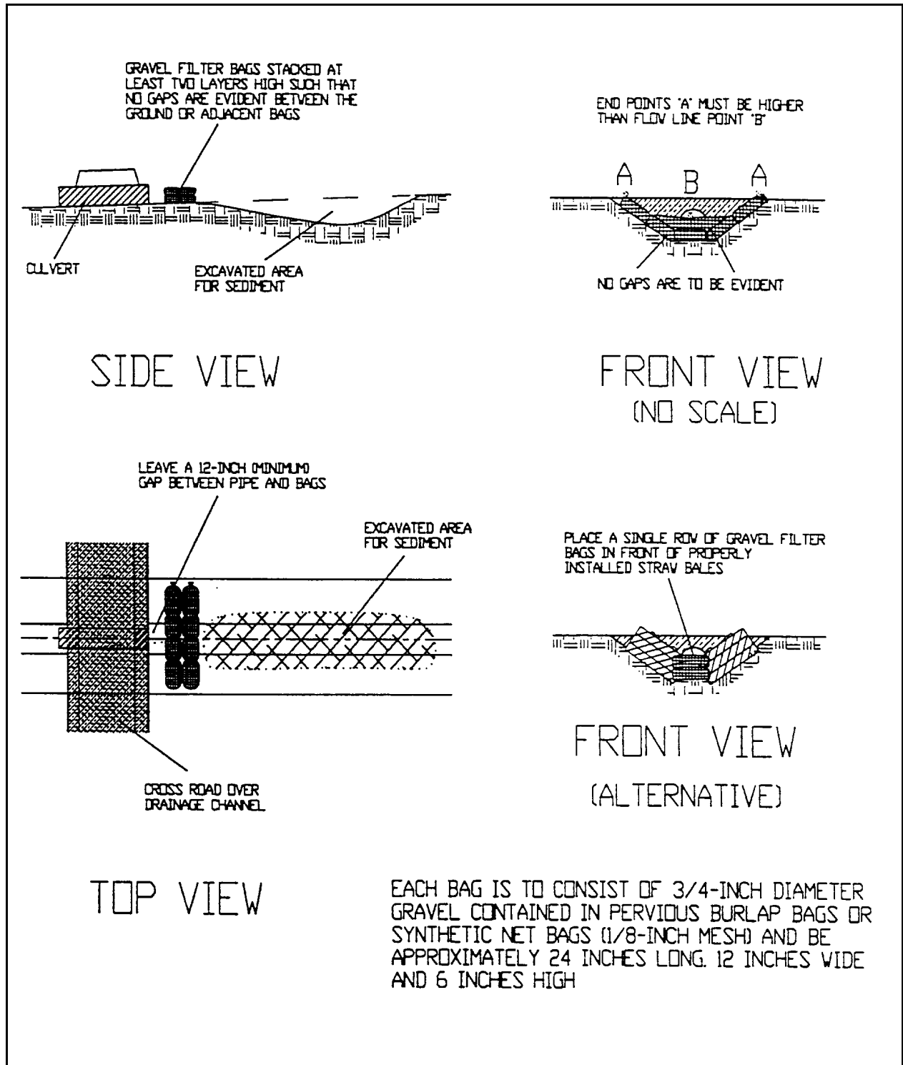
Plate 4.25g Small Sediment Trap Located within a Stormwater Conveyance Channel
