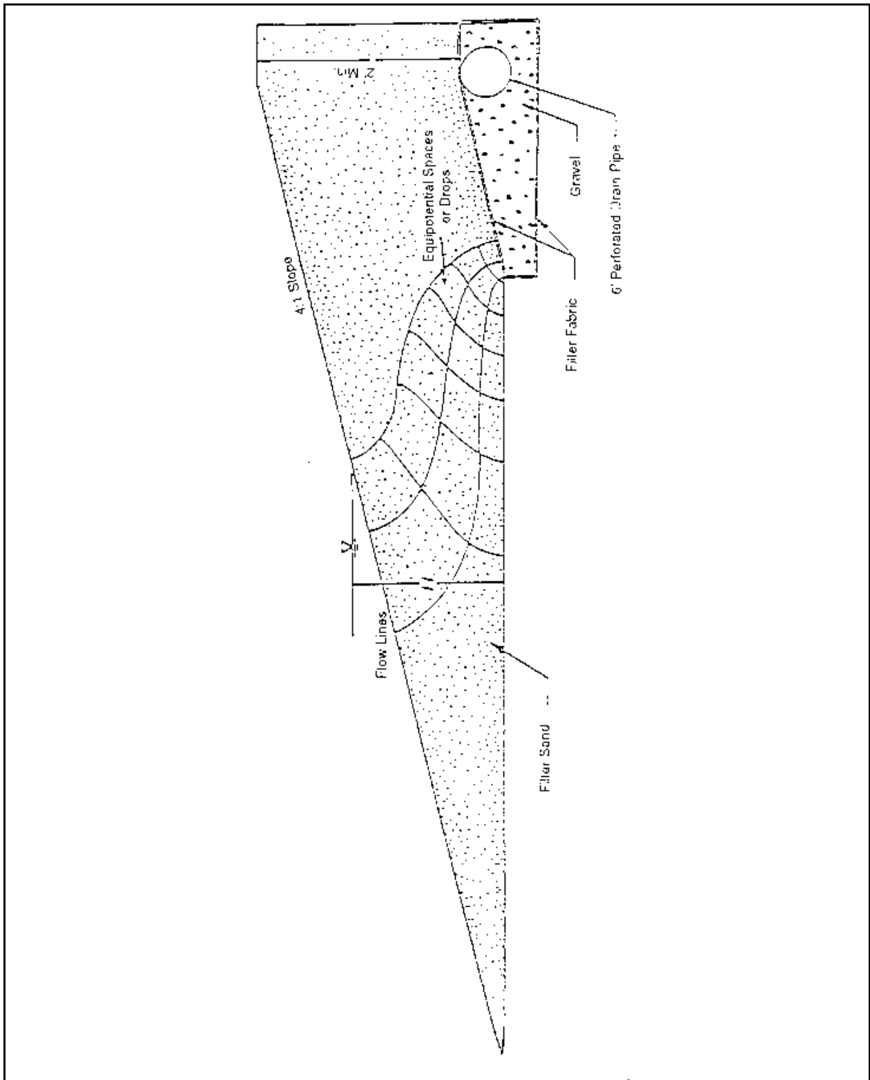
Plate 5.06j Flow Net Diagram Illustrating Lines of Seepage Through a Typical Bank Filtration System.
