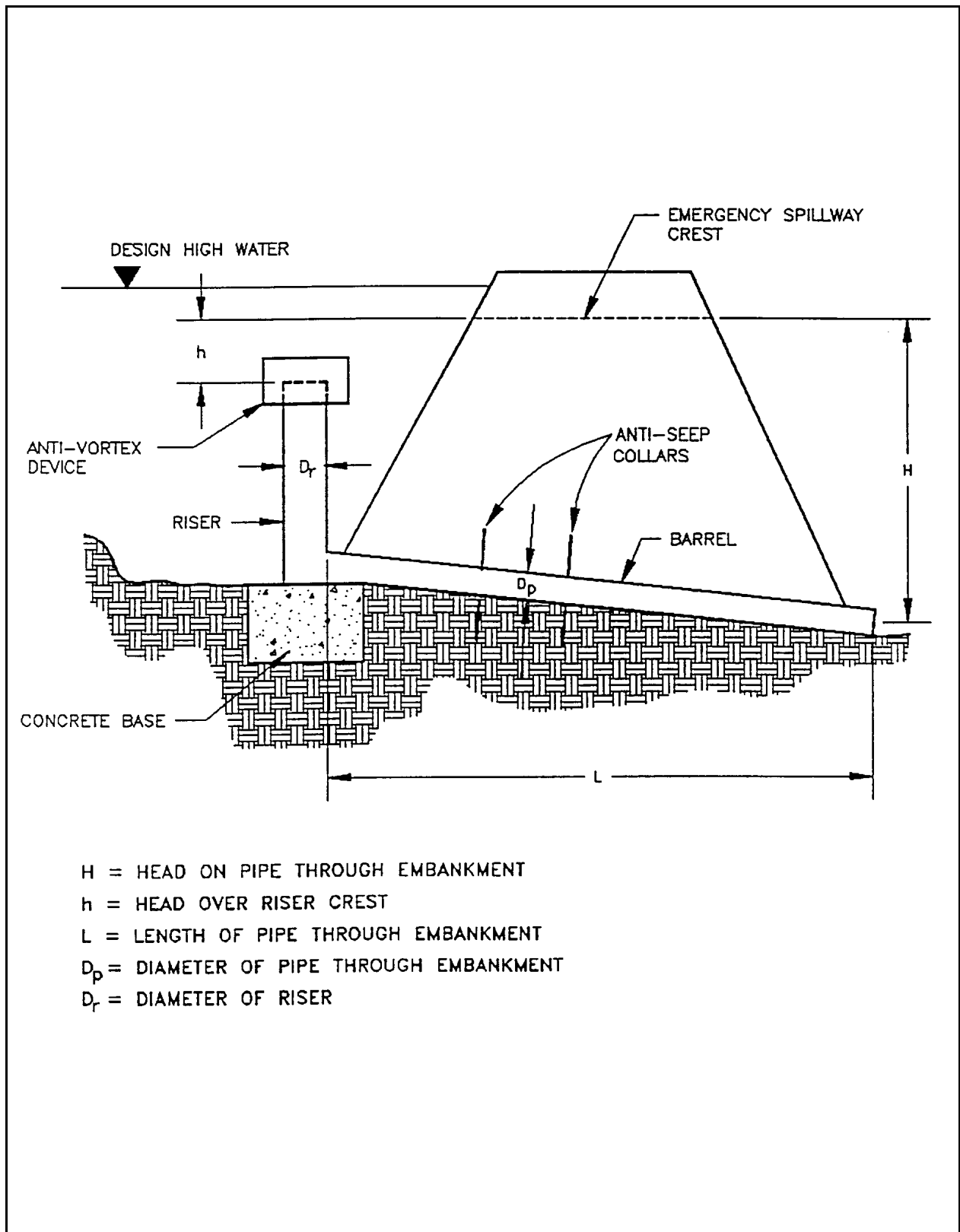
Plate 4.26i Principal Spillway Design Source: Virginia DSWC
