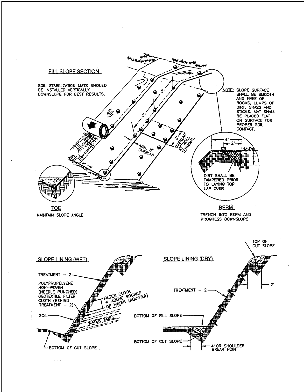
Plate 6.75d Typical Treatment 2 - Soil Stabilization Matting Slope Installation
