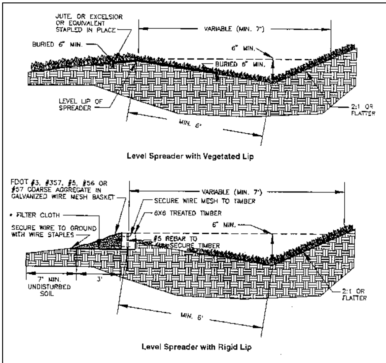
Plate 5.11b Level Spreader Cross-Section
