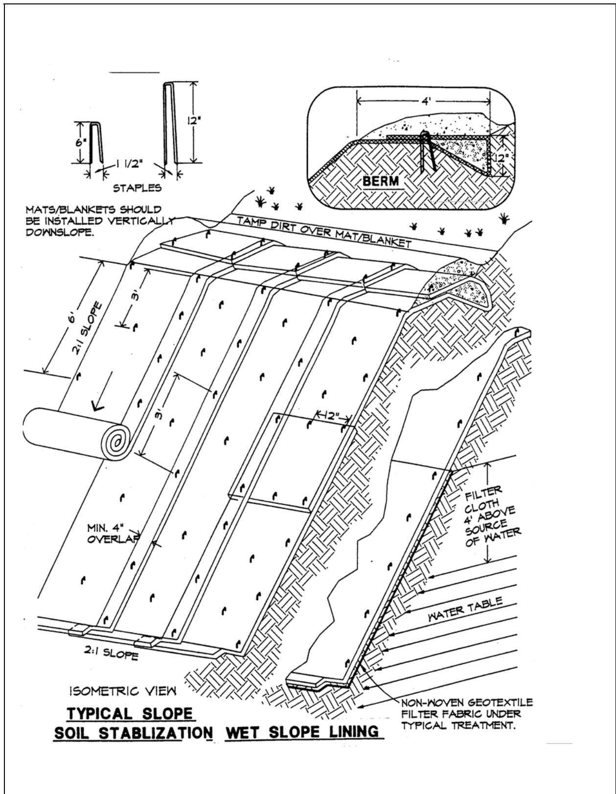
Plate 6.75c Erosion Blankets and Turf Reinforcement Mats - Slope Installation
