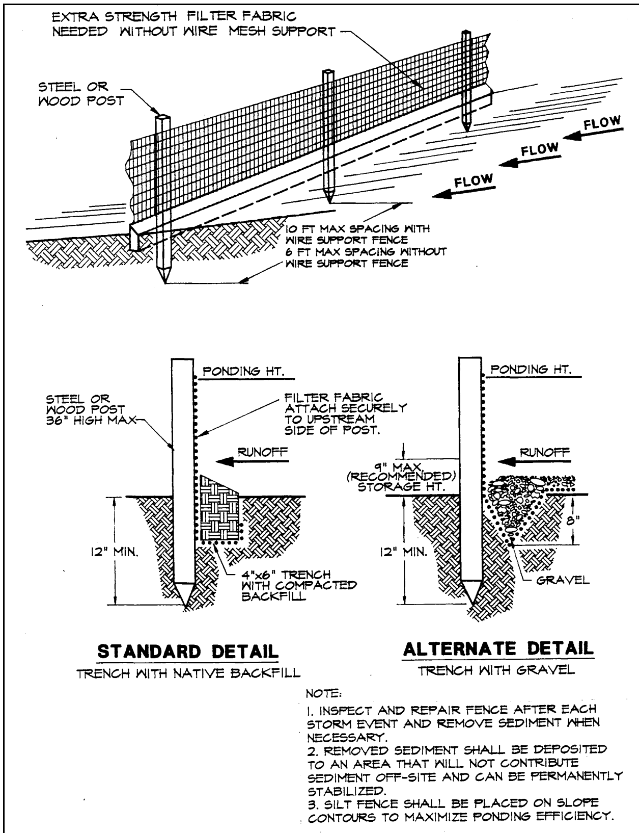
Plate 4.06e Silt Fence
