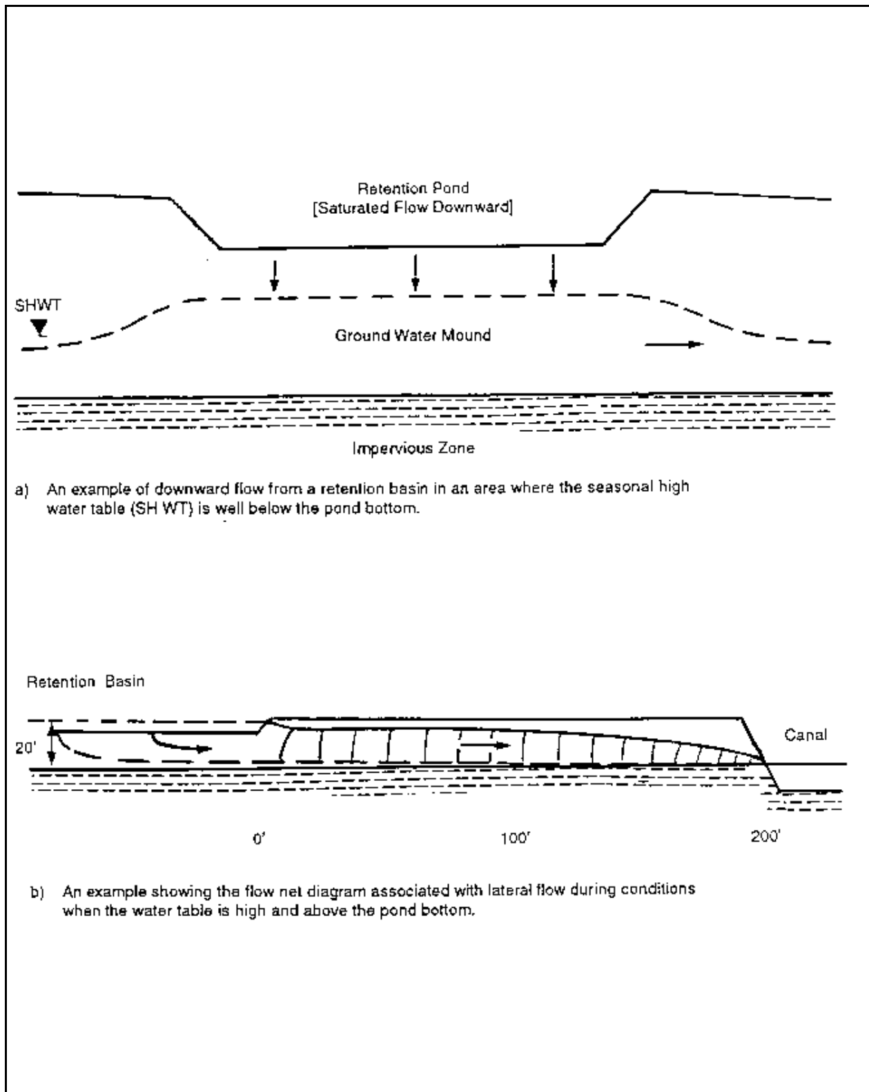
Plate 5.01b Schematic of Flow Characteristics Associated with Infiltration from Retention Ponds during Low and High Water Table Conditions
