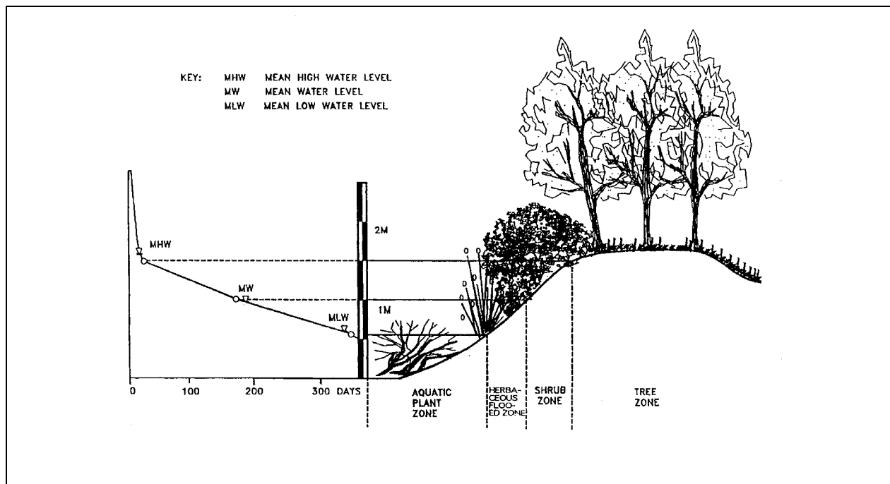
Plate 6.98a Typical Annual Curve of Water Levels Correlated with Typical Vegetative Zones
