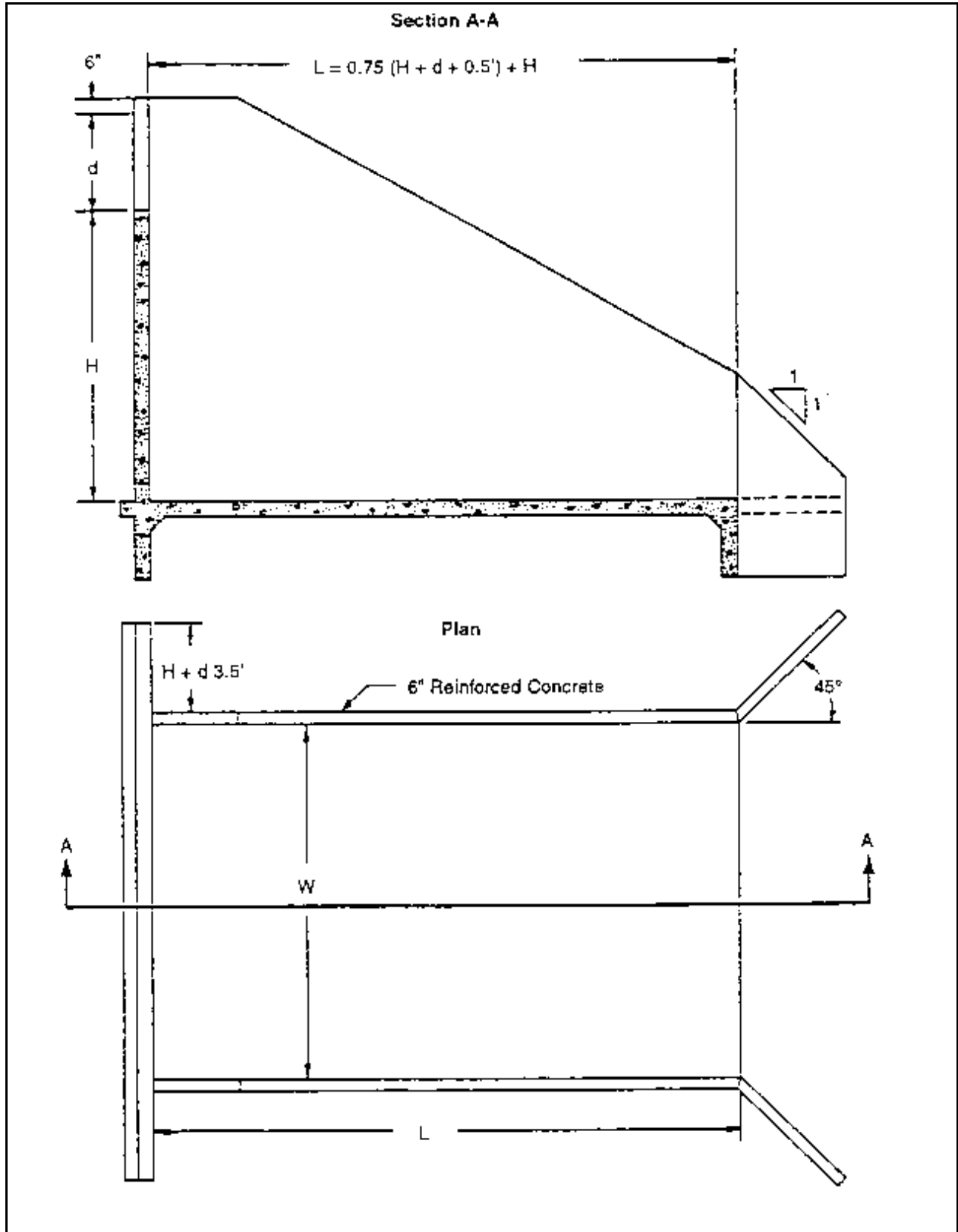
Plate 5.14c Waterway Drop Structure Details Source: Soil and Water Conservation Engineering , Schwab et al
