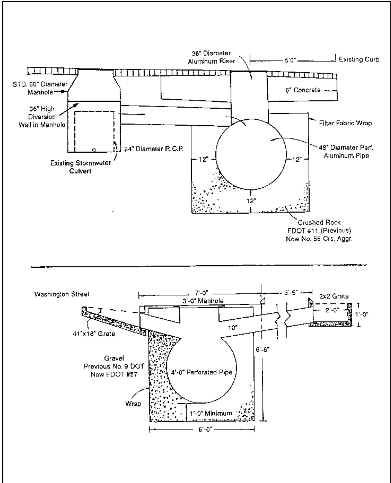
Plate 5.02d Examples of Typical Underground Percolation Systems for Retrofitting Existing Stormsewer Systems in Orlando, Florida. Source: NRCS
