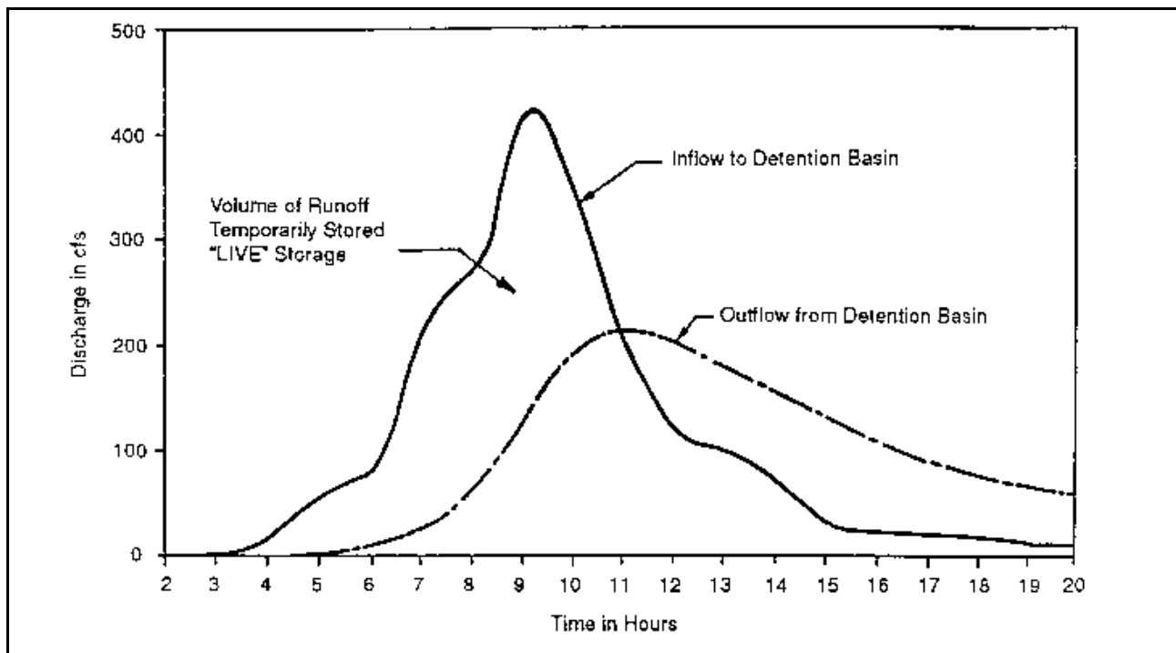
Plate 5.05a Typical Detention Basin Hydrographs
