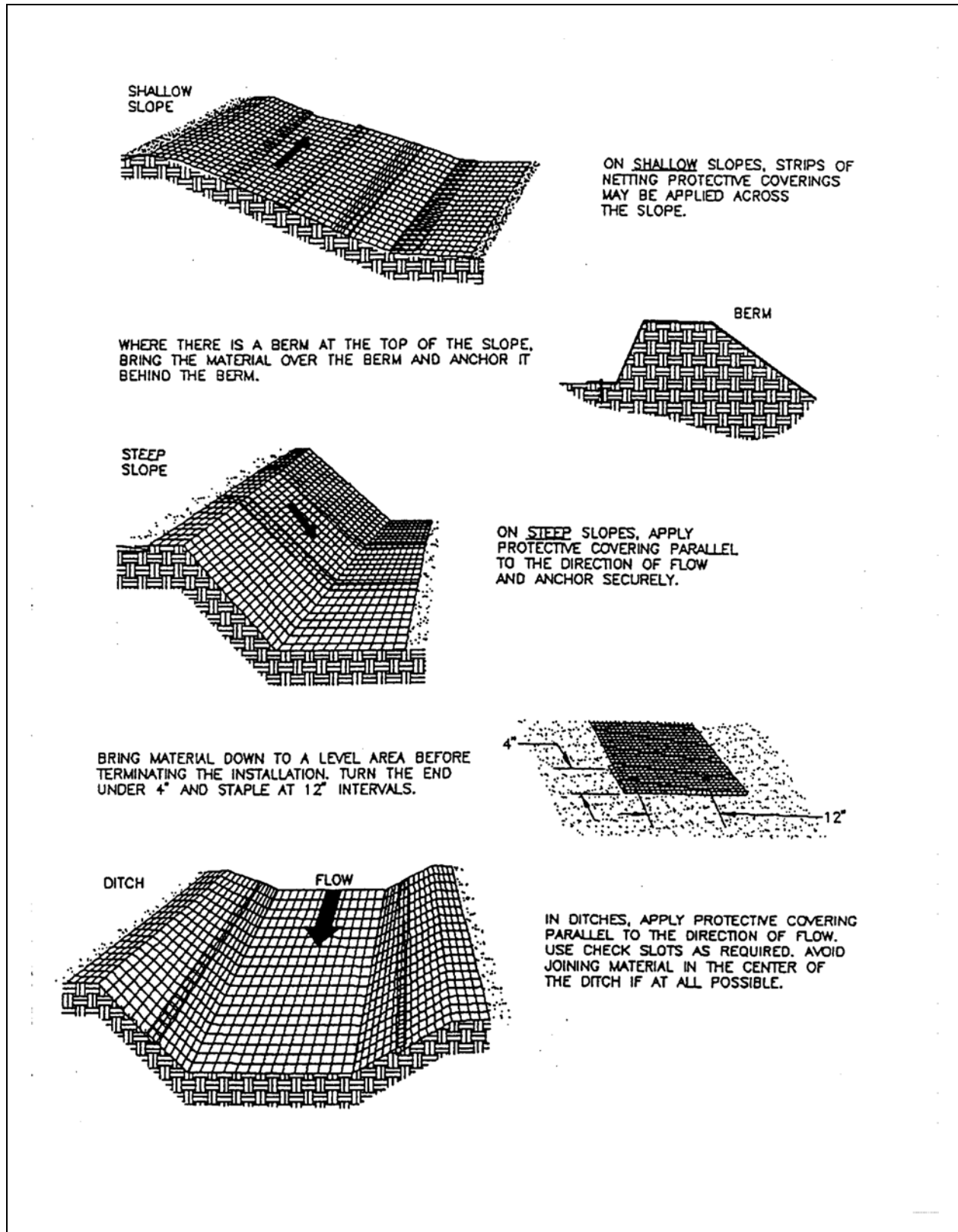
Plate 6.75a Typical Orientation of Treatment 1 - Soil Stabilization Blanket
