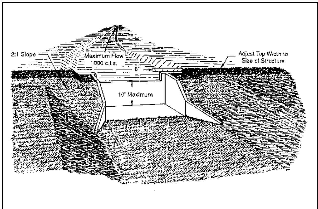
Plate 5.14a Waterway Drop Structure Source: NRCS
