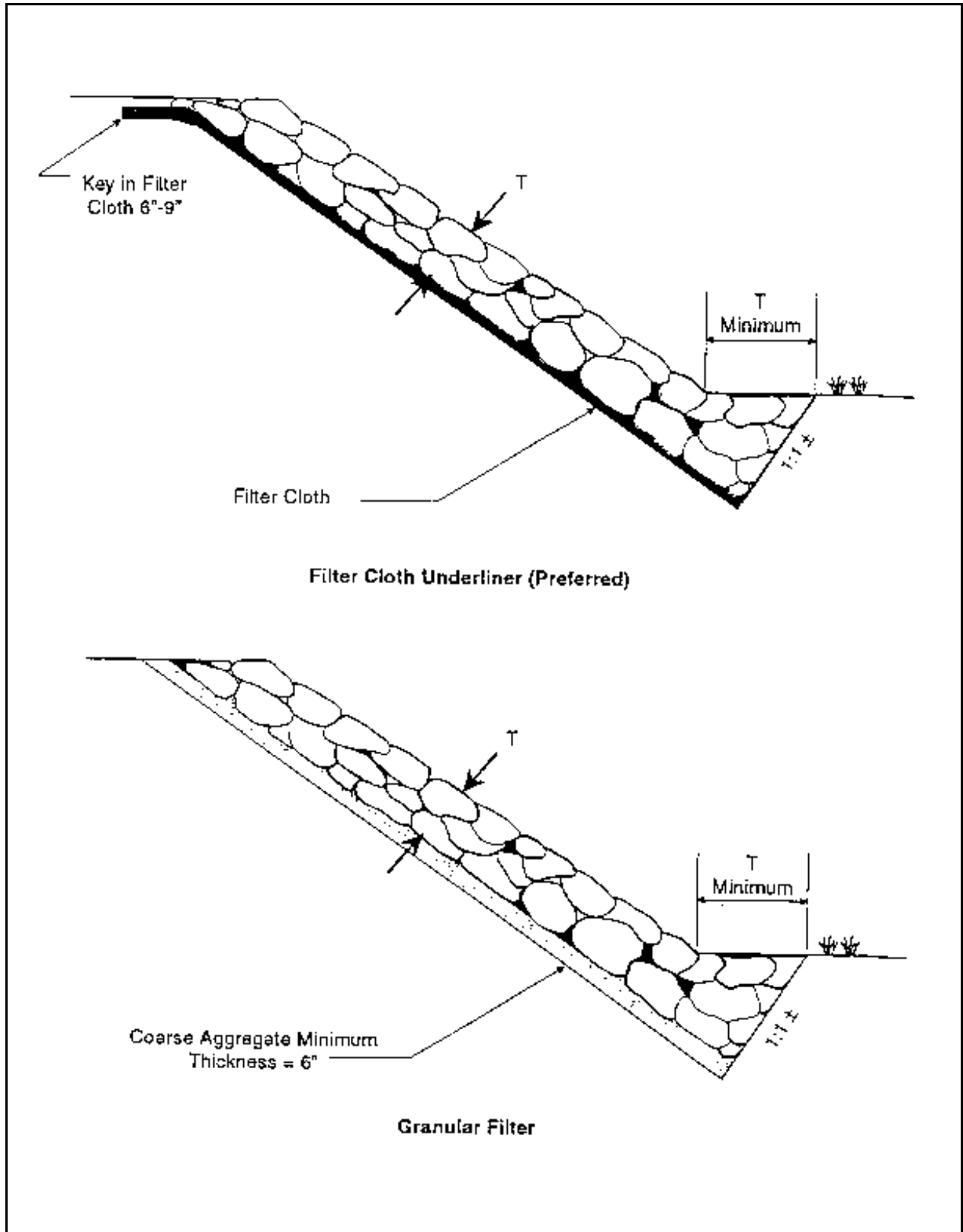
Plate 5.16c Toe Requirements for Bank Stabilization Source: Virginia Department of Highways and Transportation Drainage Manual
