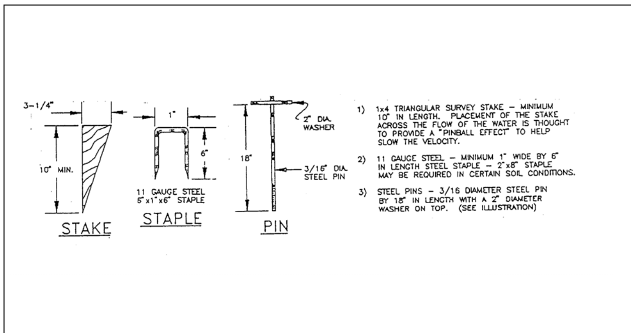
Plate 6.75g Stakes, Staples, and Pins for Installation Soil Stabilization Matting
