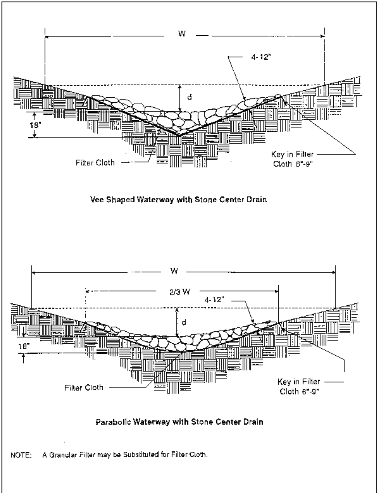
Plate 5.08b Typical Stone-Lined Waterways Source: NRCS
