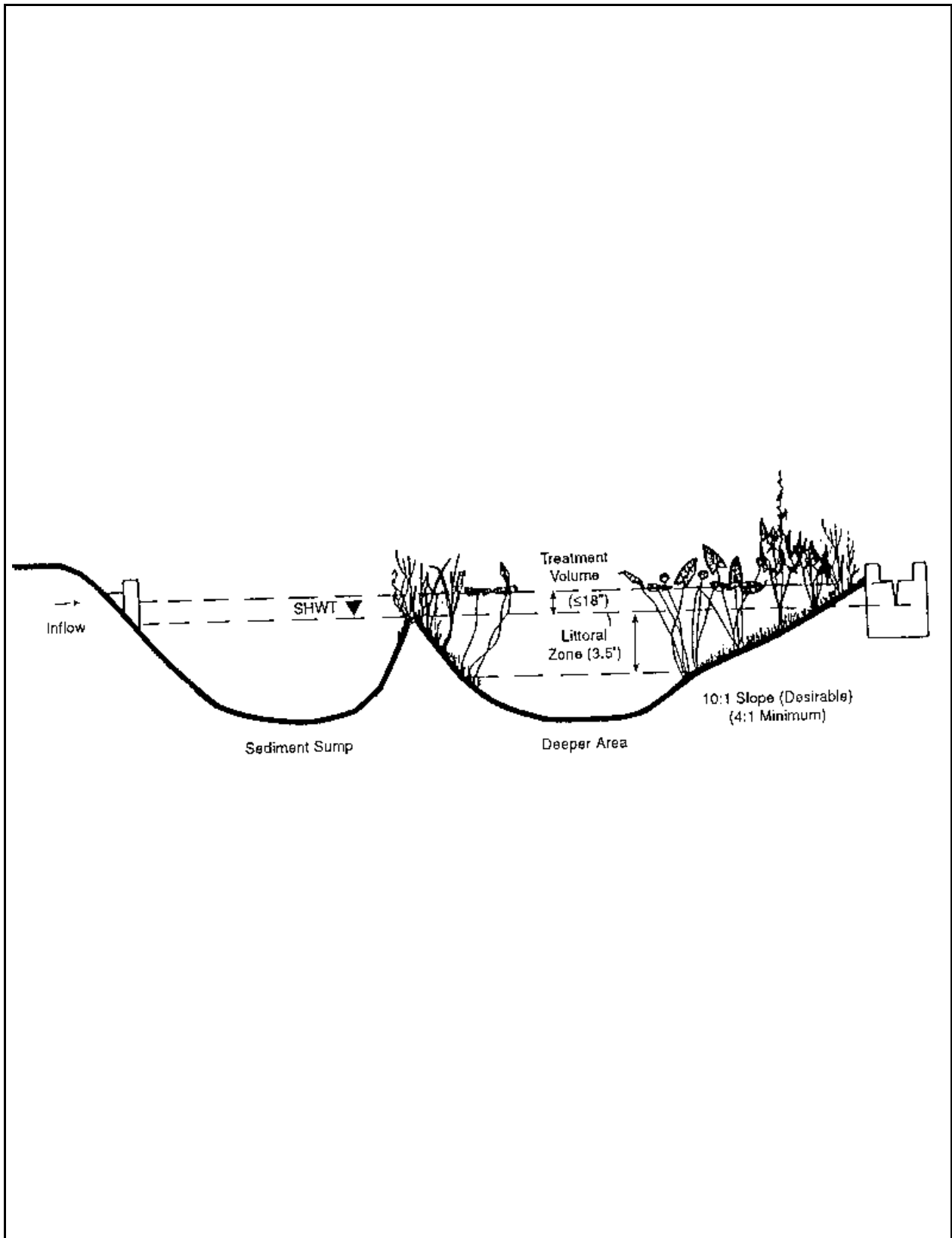
Plate 5.05d Wet Detention System, Pond Configuration - B
