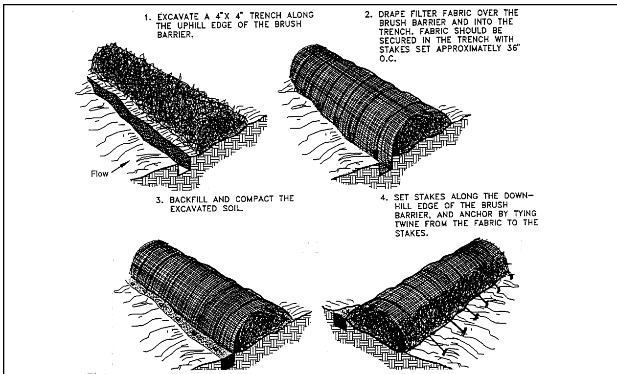
Plate 4.07a Construction of a Brush Barrier Covered with Filter Fabric
