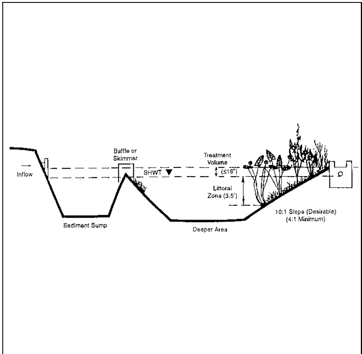
Plate 5.05c Wet Detention System, Pond Configuration - A
