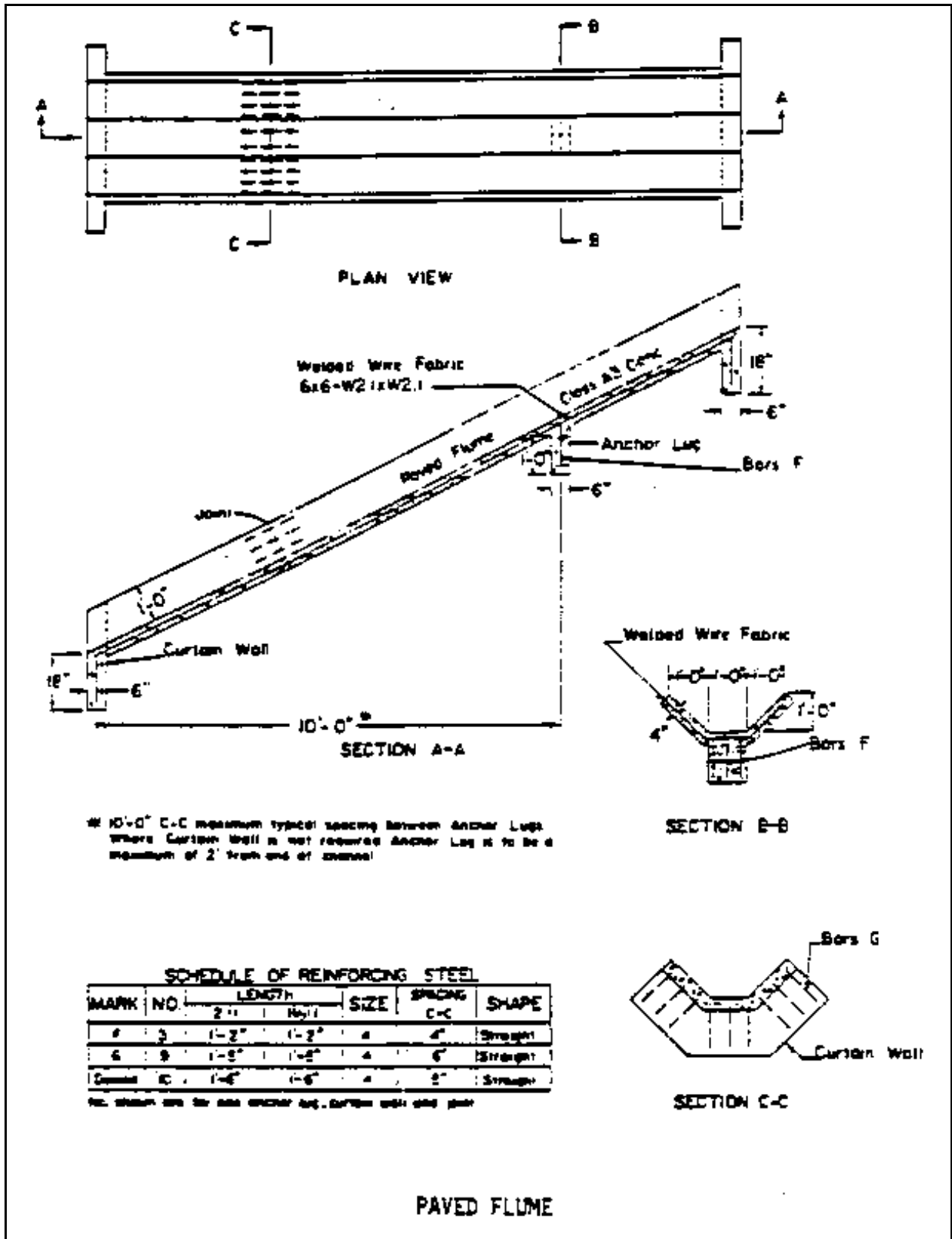
Plate 5.09a Paved Flume
