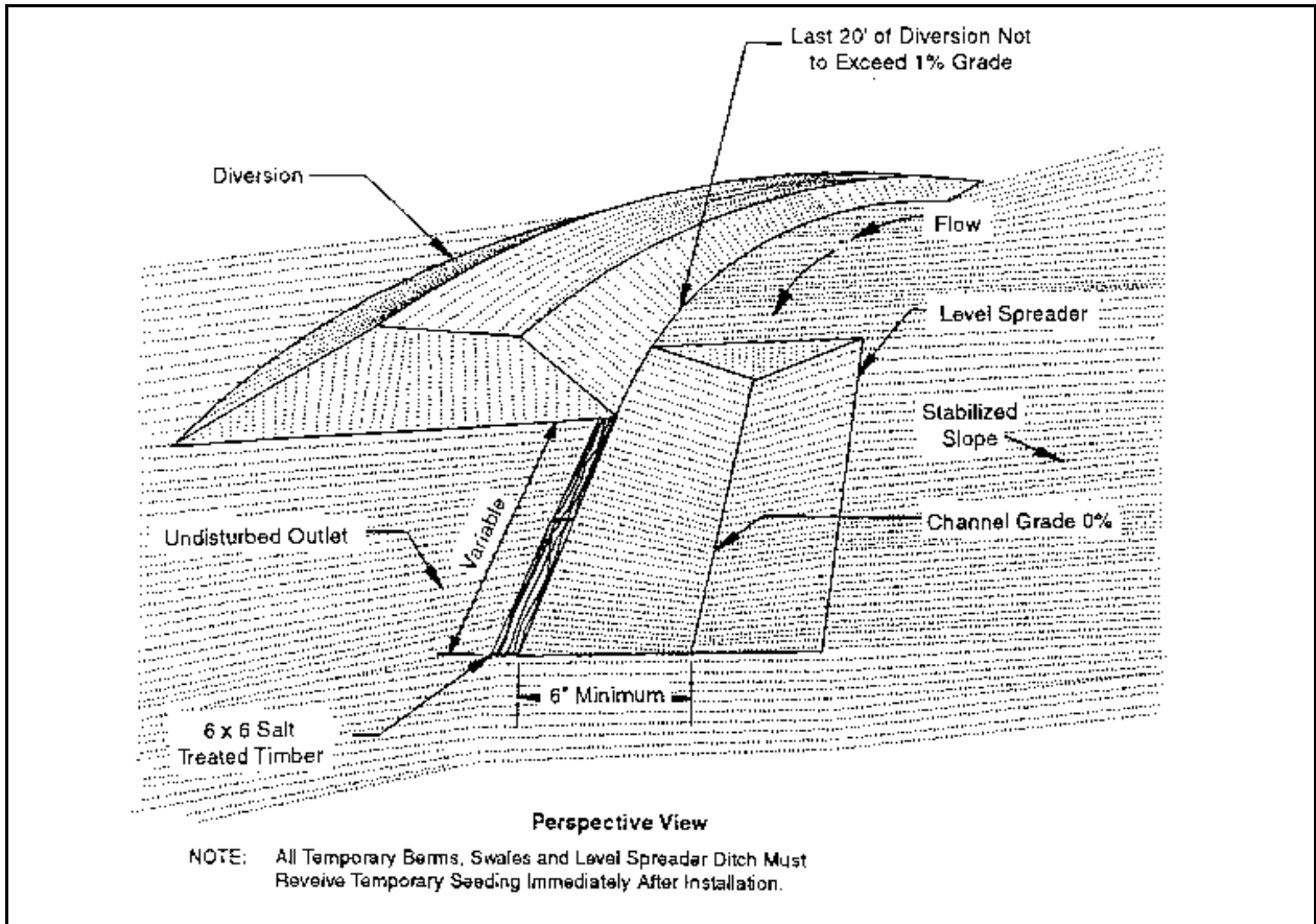
Plate 5.11a Level Spreader
