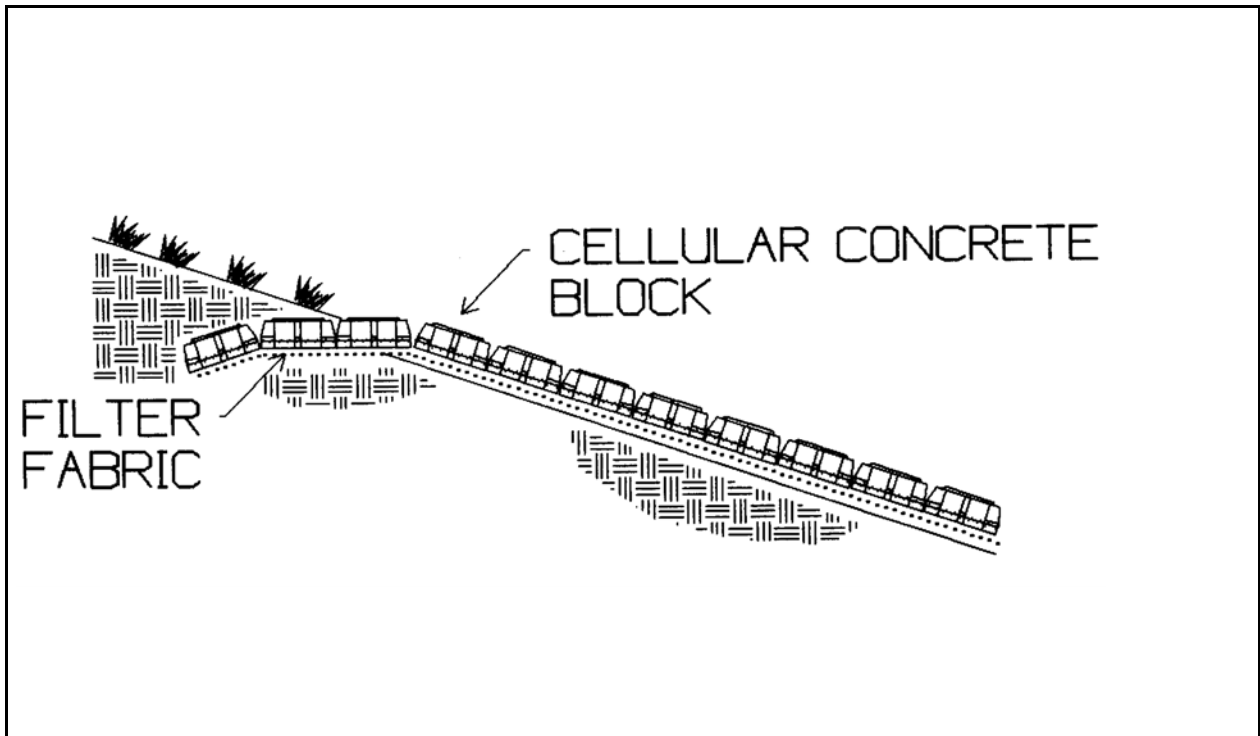
Plate 5.18a Slope Protection
