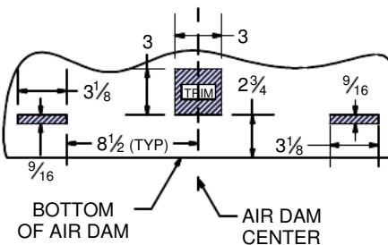
TRIM DIAGRAM (2010 MODELS ONLY)
