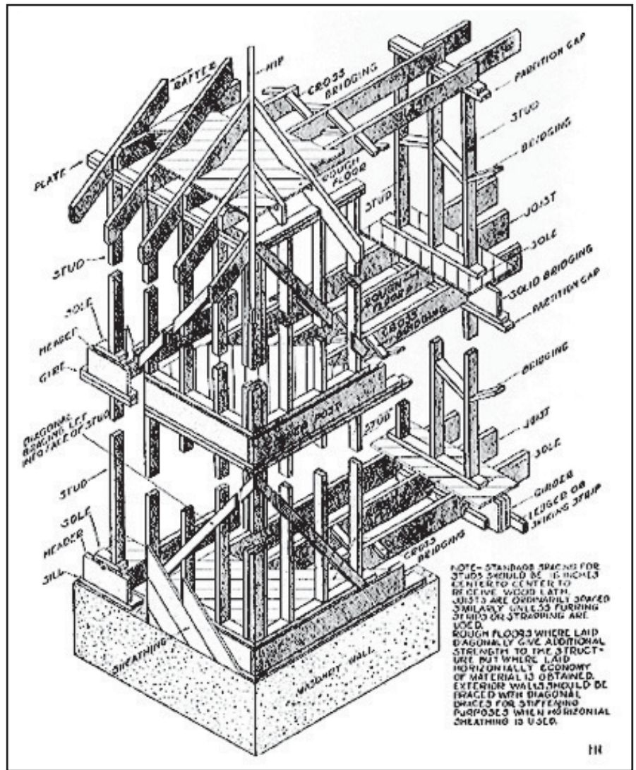
Figure 6. Platform Framing.
