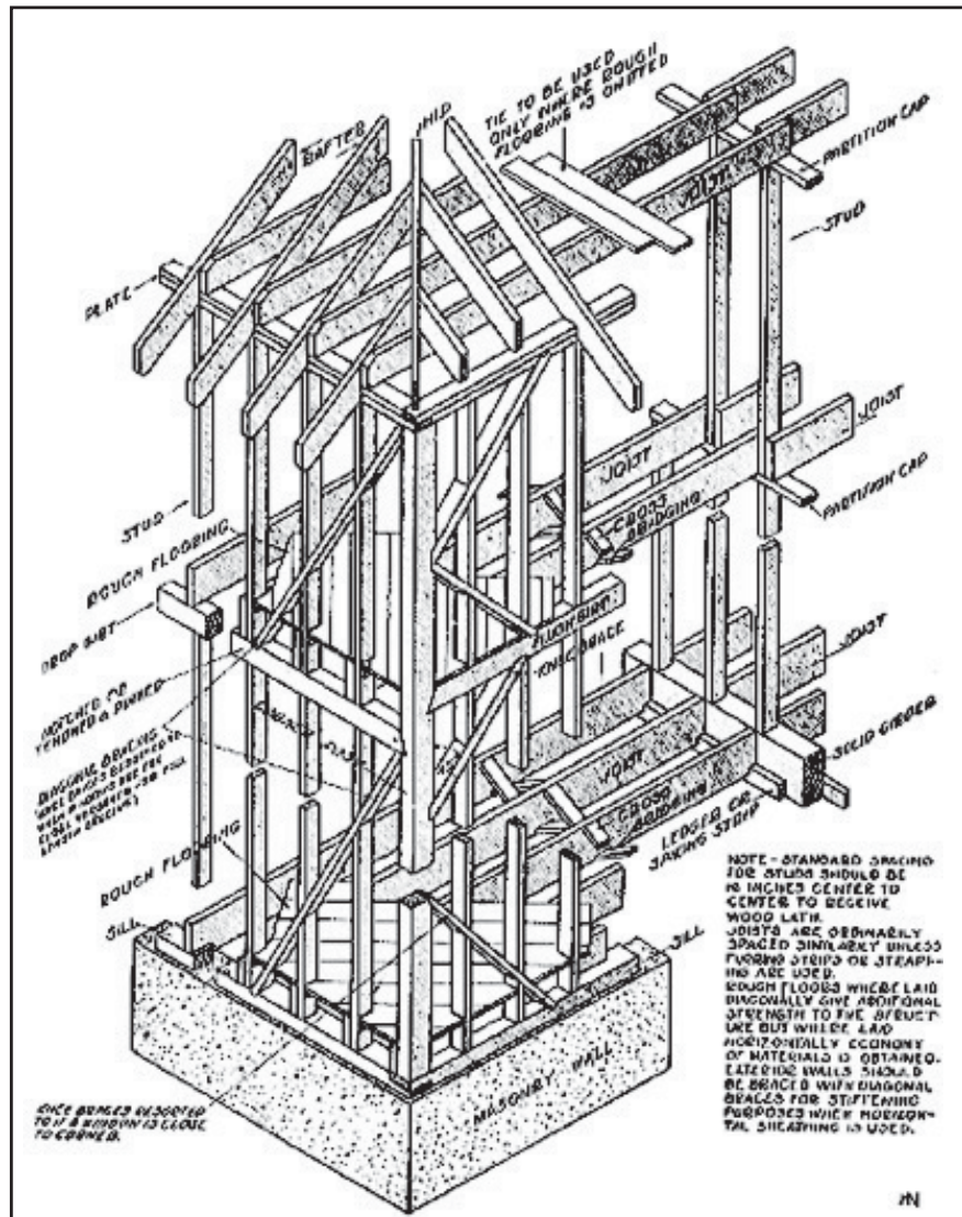
Figure 4. Braced Framing pre-1900.
