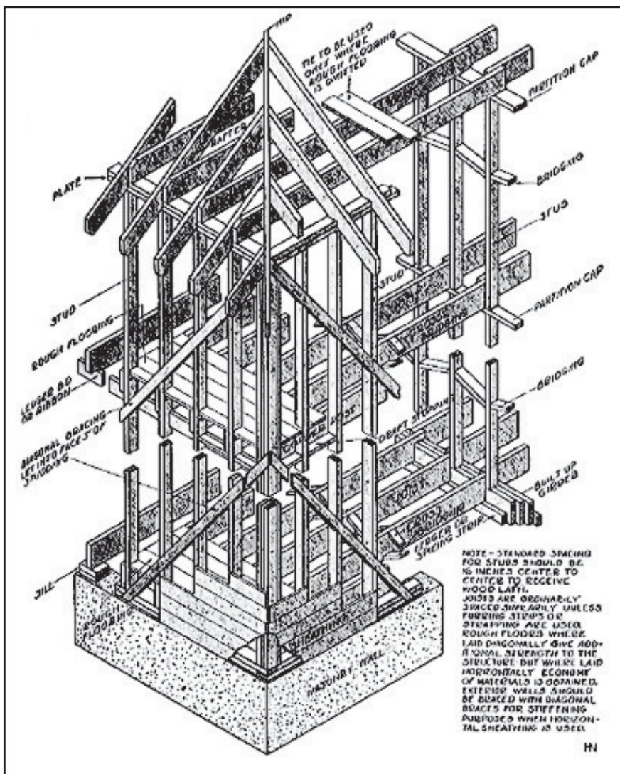
Figure 5. Balloon Framing Technique in Early 1900s.
