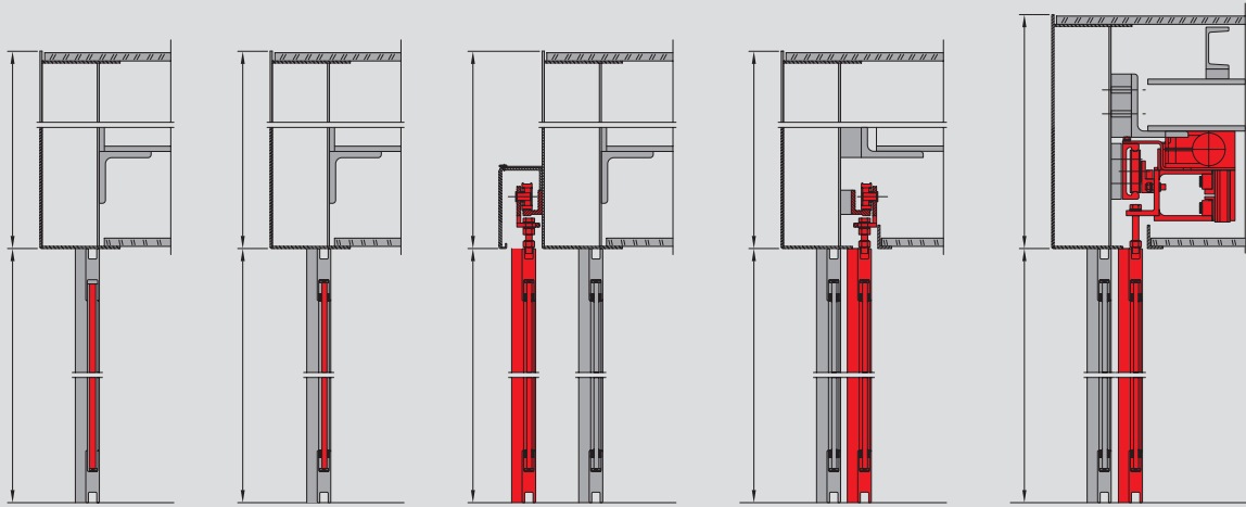
Drum wall with metal panelling
