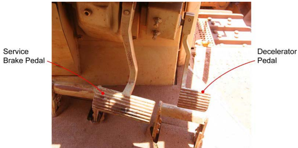
Foot Pedal Controls
