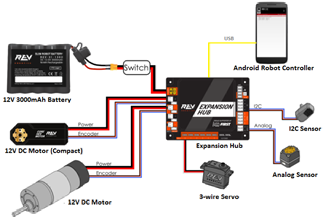
Figure 1: Expansion Hub Configuration
