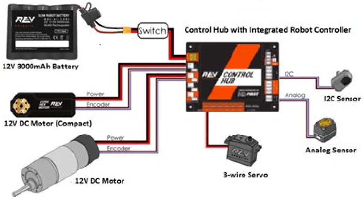
Figure 2: Control Hub Configuration
