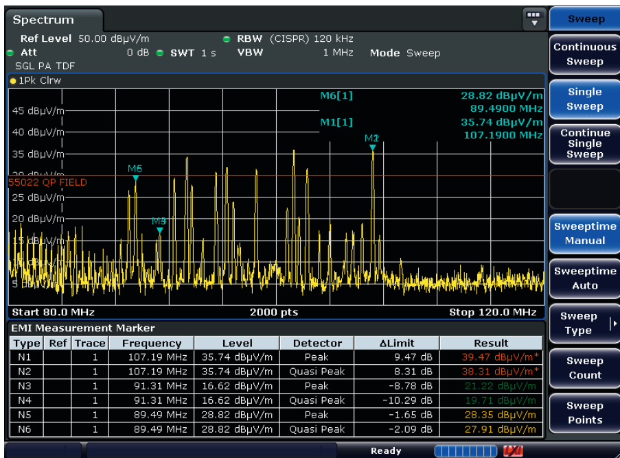
Single sweep with EMI measurement markers.
