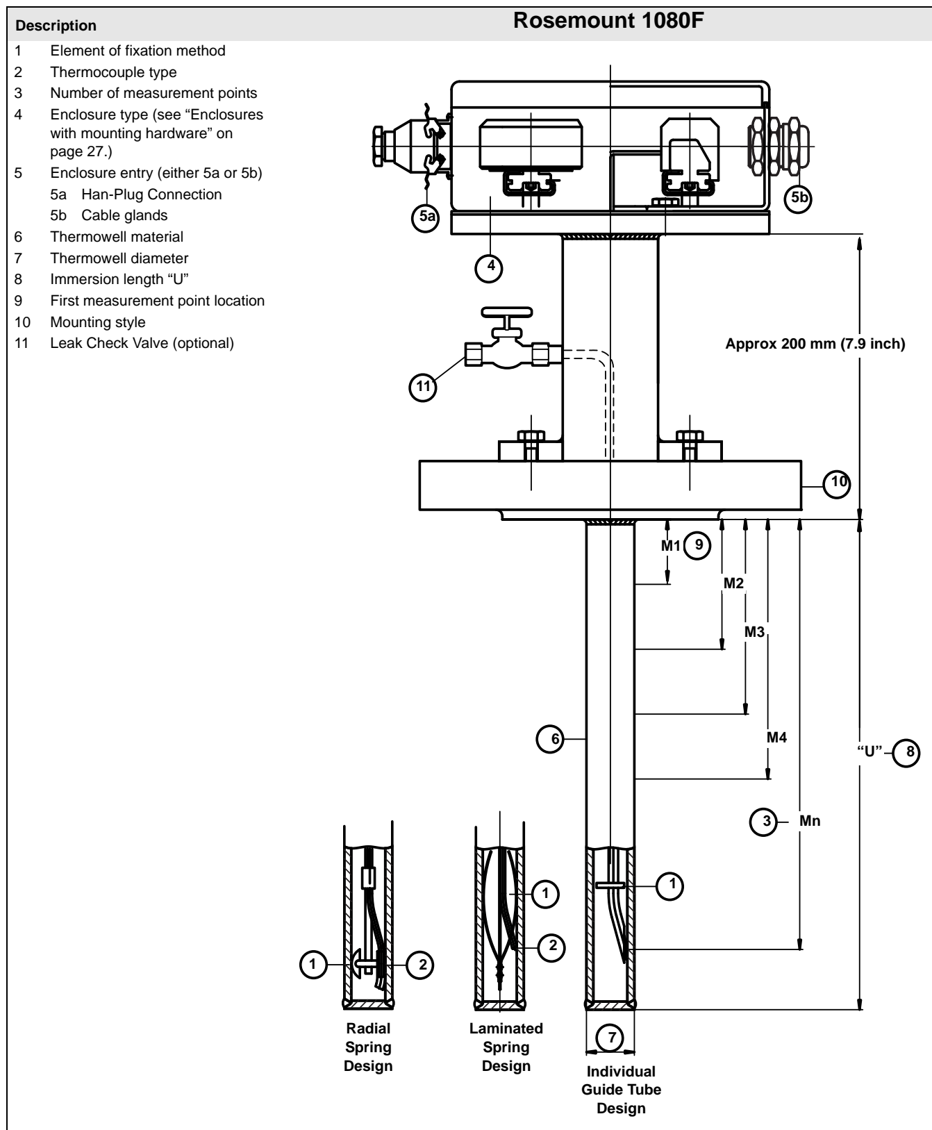
Figure 5. Multipoint Sensor Rosemount 1080F Thermocouple Multipoint Sensor. Contacting Fixture Design
