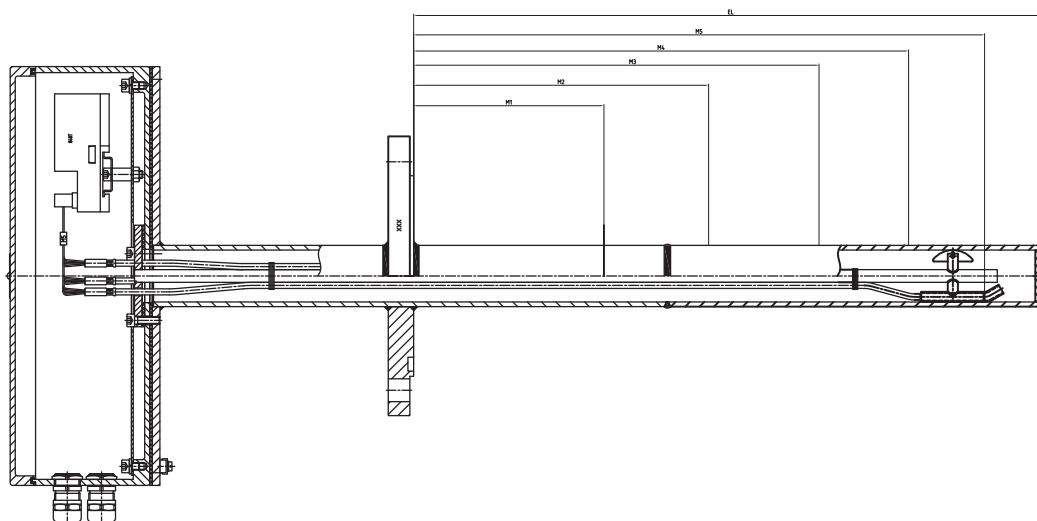
Radial Spring Multipoint Design
