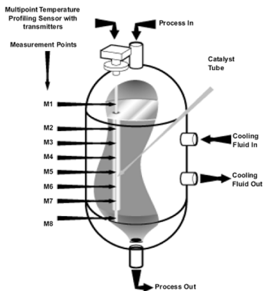
Figure 1. Reactor
