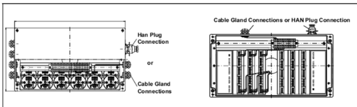
Figure 12. Enclosures
