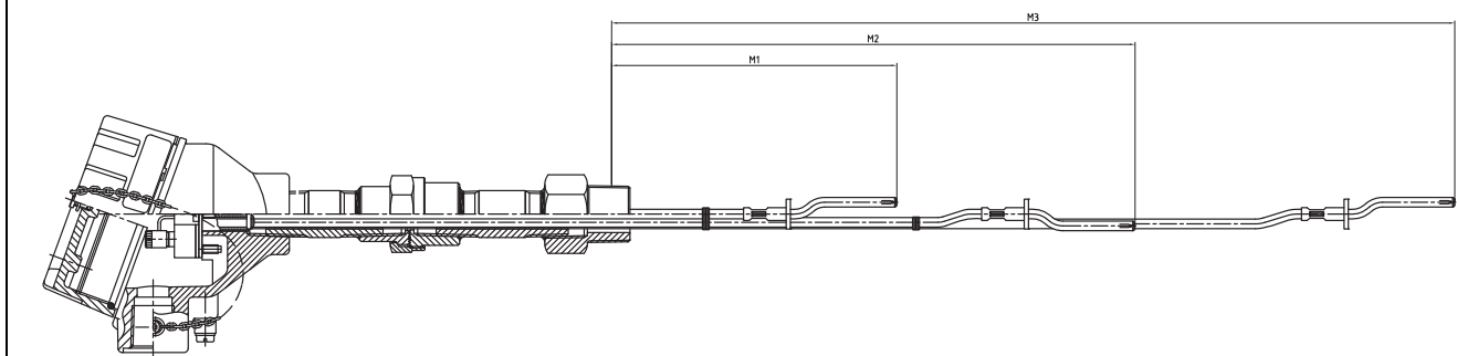
Spacer Multipoint Design
