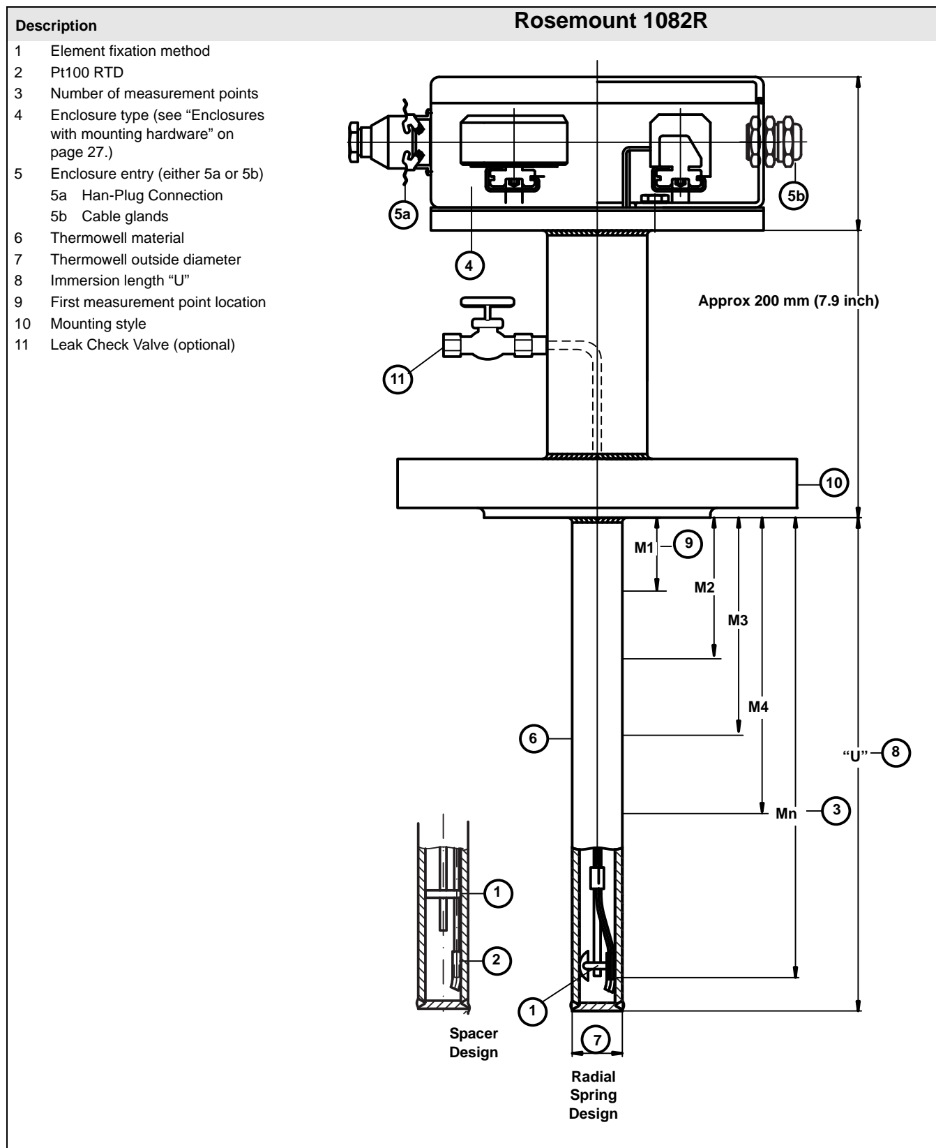
Figure 6. Multipoint Sensor Rosemount 1082R, Radial Spring and Spacer Design (Pt 100 RTD)
