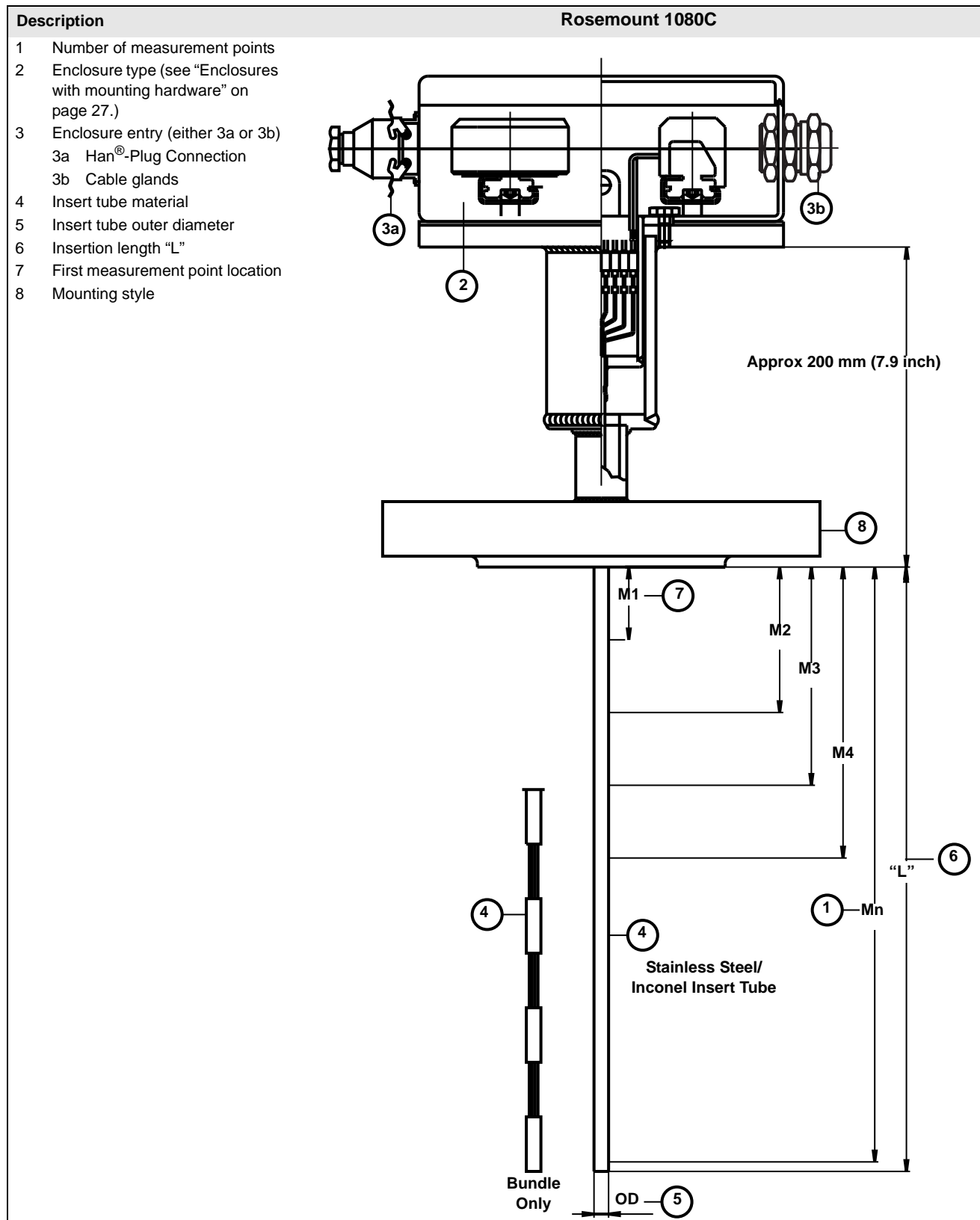
Figure 4. Multipoint Sensor Rosemount 1080C Compact
