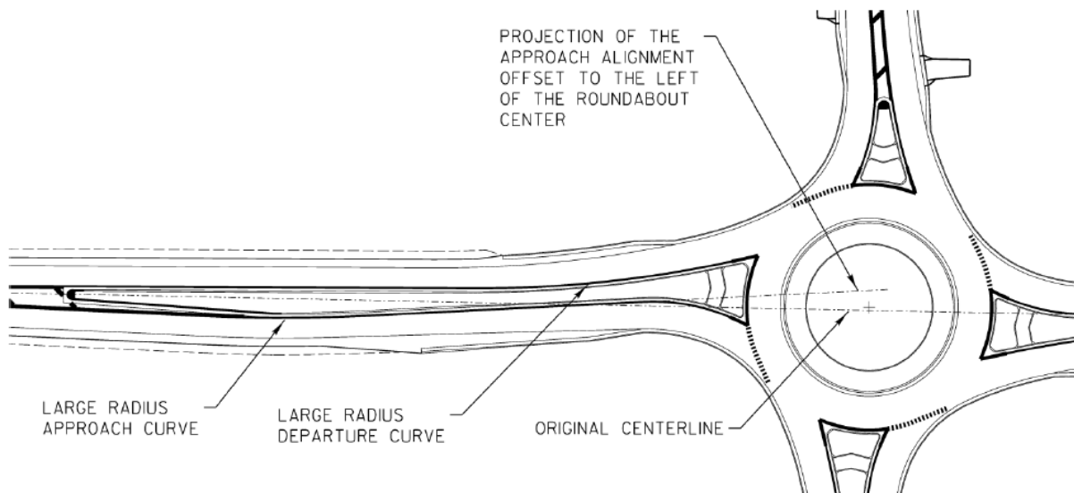
Figure 3.4 – Roundabout Entry Deflection (Source: WisDOT 4 )
