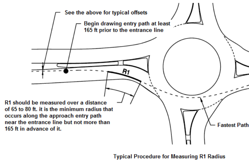
Figure 3.47 – Fastest Path Radii Construction (Source: NCHRP 672 2 )
