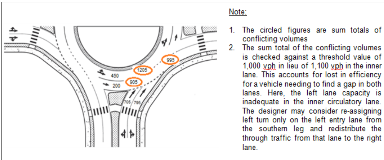
Figure 2.2 – Lane-by-Lane Checks for Capacity Limits on Two Lane Roundabout Approaches
