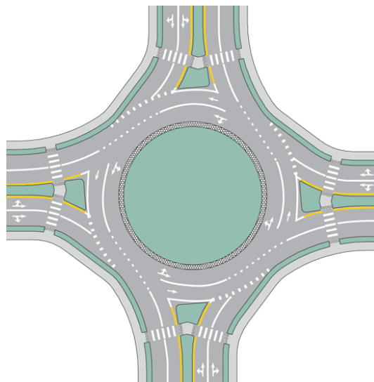
Figure 4.1 – Typical Pavement Marking Layout for Single Thru/Right lane and Left Turn lane (Source: MUTCD, 2009)
