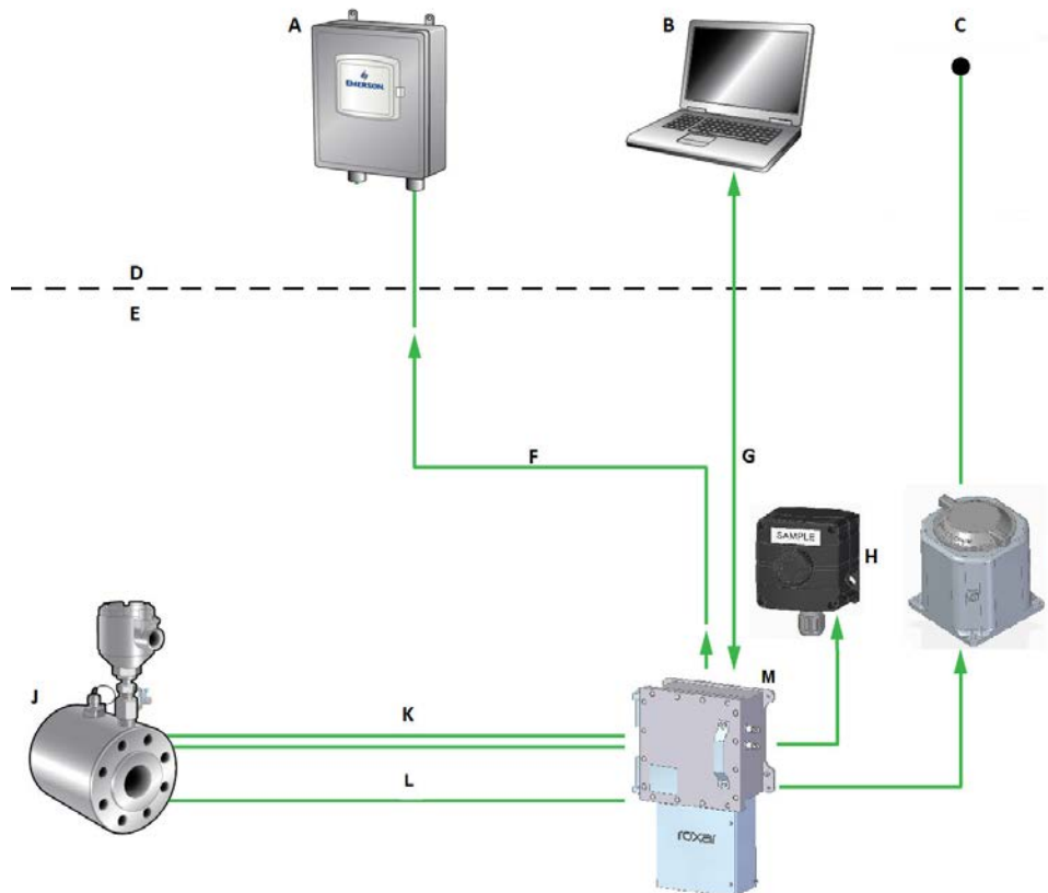
Figure 6: Typical Block Diagram for a Roar Water cut Meter
