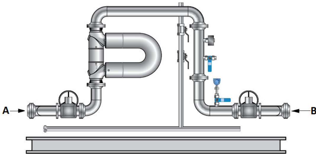
Figure 2: Roxar Watercut Meter Flow with inline Coriolis flow meter
