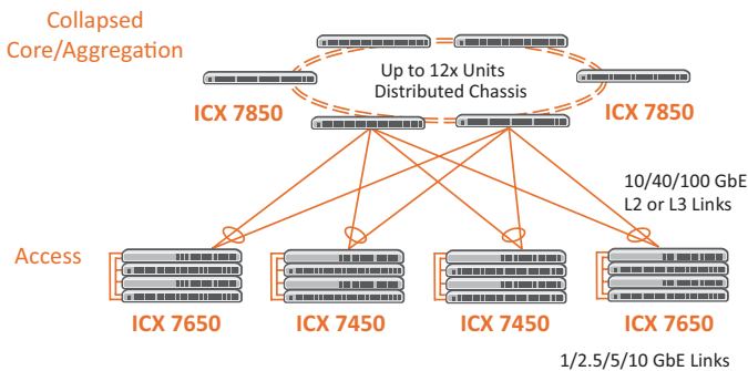
Figure 4: Two-tier campus network.
