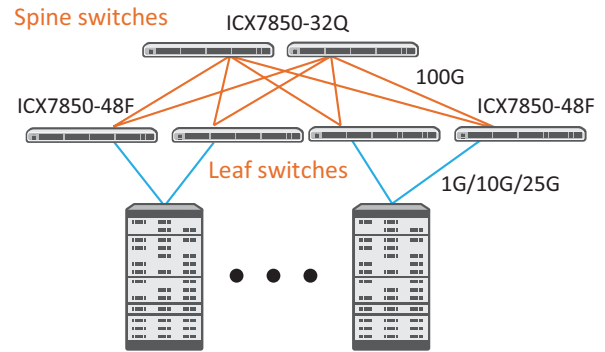
Figure 7: ICX 7850 spine-leaf solution.
