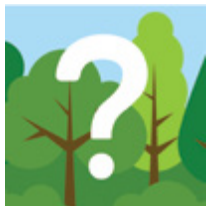
UNKNOWN ECOLOGY
