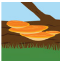
SAPROBE/DECOMPOSER
