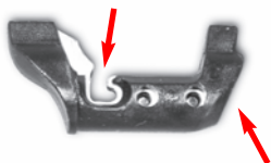
Magazine Catch Removed From Pistol - To Show Notch for Spring Rod
