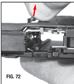
View From Top - Magazine Catch Spring Rod In The Notch
