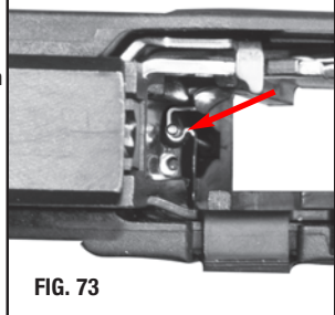
View From Top - Magazine Catch Spring Rod In The Notch
