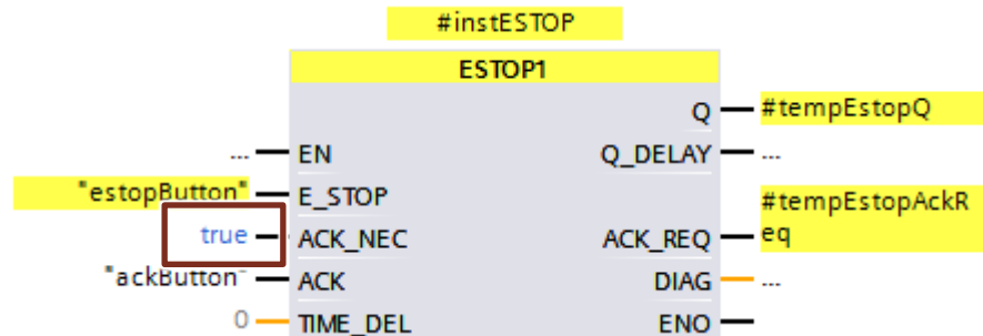
Figure 3-4: "TRUE" / "FALSE" signals as actual parameters
