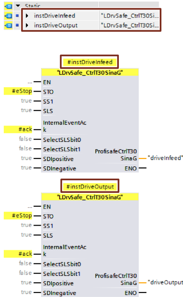
Figure 4-4: Multi-instances
