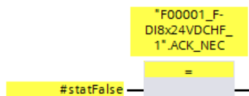
Figure 3-19: Programming automatic reintegration
