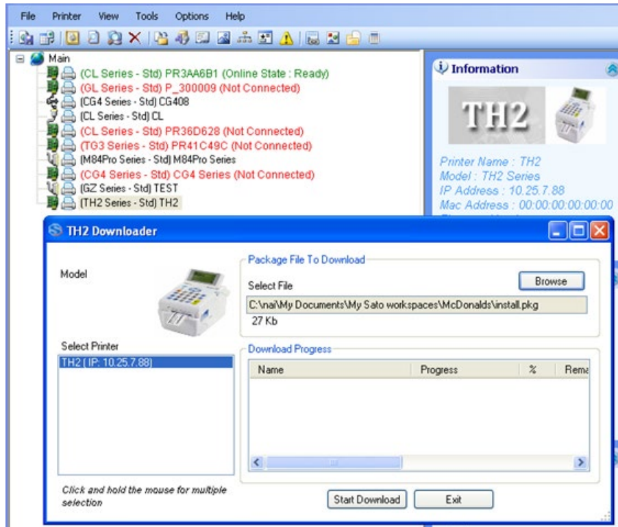
Figure 37 TH2 Downloader
