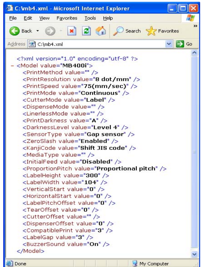
Figure 46 XML File
