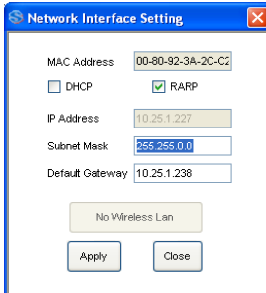
Figure 56 Network Setting
