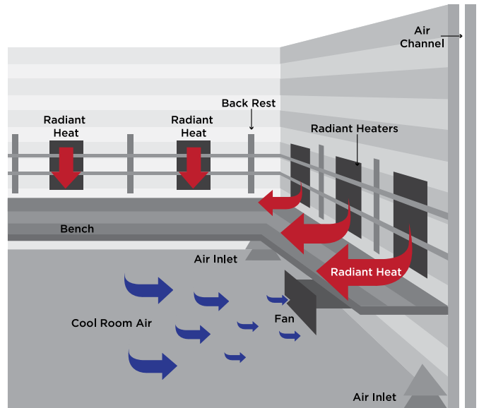
Rapid Even Air System (Convection Method for a Balanced Heated Sauna)* All Saunacore heating units are manufactured to meet the latest CSA, UL and CE safety requirements. *Available on 'Premium' and 'Max' Series
