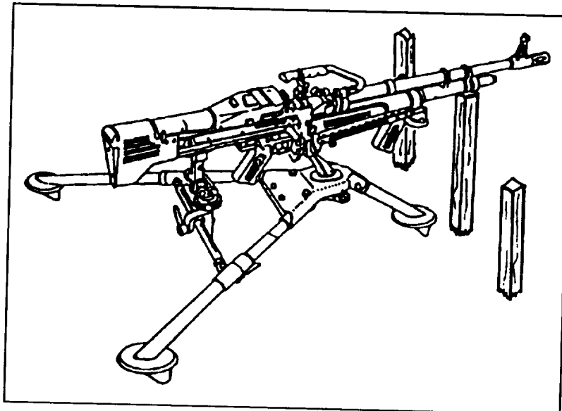
Figure 4-25.—Muzzle stakes.
