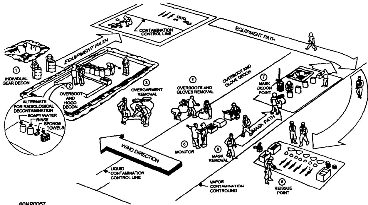
Figure 6-7.—Detailed troop decon layout.
