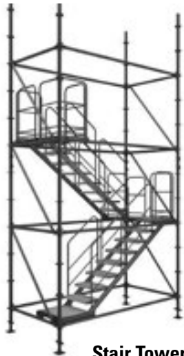
Stair Tower
