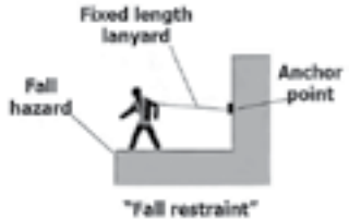
A personal fall restraint system
