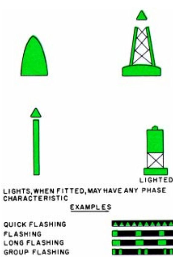
Figure 5-22.—IALA Maritime Buoyage System, International Buoyage Region A starboard-hand marks (buoys). C69.215
