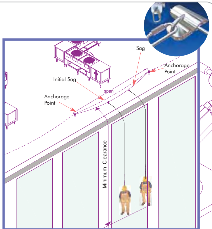
KEY LINE DIAGRAM ILLUSTRATING CLEARANCE REQUIREMENT IN A FALL ARREST SITUATION
