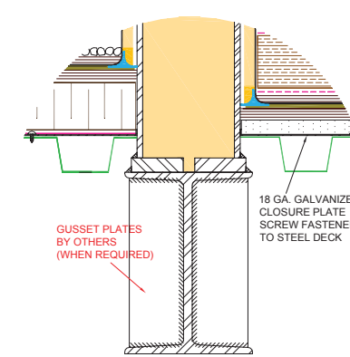
Welded (K-FARA-4-700)
