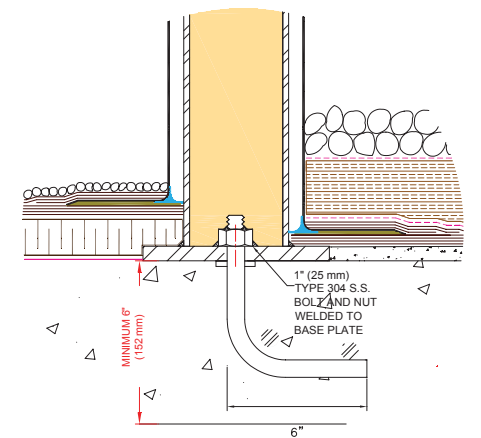
Cast-In-Place (K-FARA-5-701)
