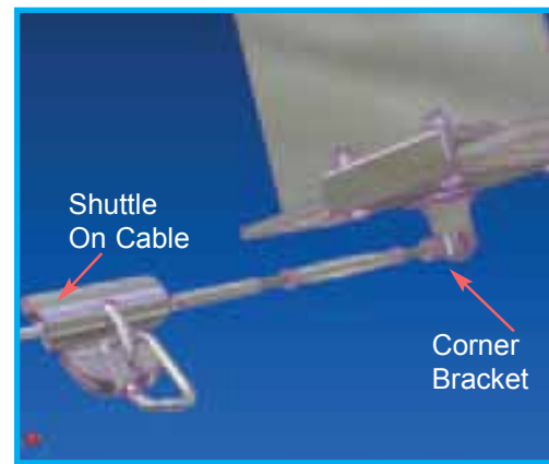
TERMINAL END ANCHOR WITH TENSIONER (Temporary. View From Below)
