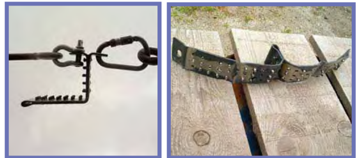
Thaler Energy Absorber (TEA) Before Load Test. Thaler Energy Absorber (TEA) After Load Test
