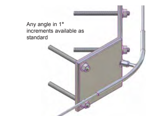
K-FARA-93-701-713 Any Angle Corner Anchor
