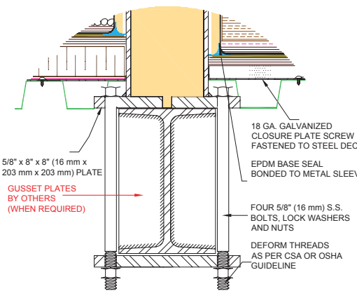
Bolt Around Beam (K-FARA-3-700)
