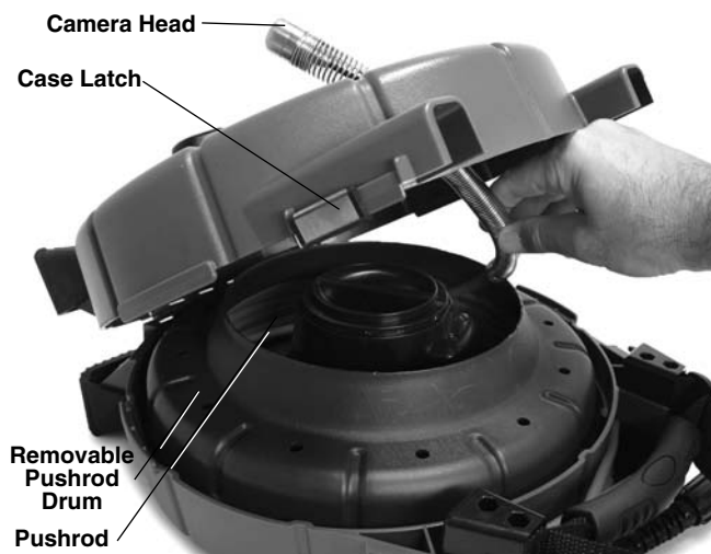
Figure 3 – Opening The Case
