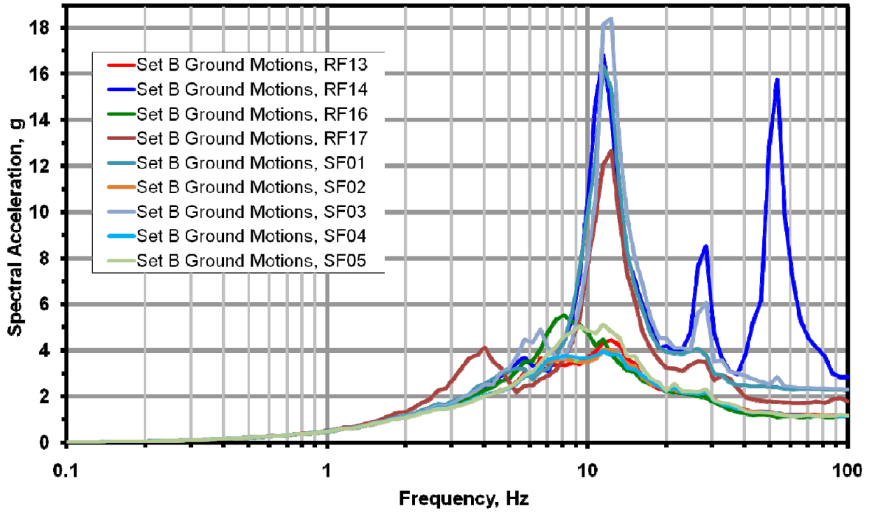
(a) Tower Top
