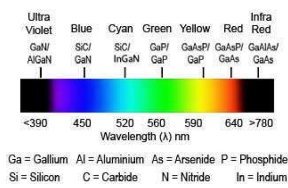
Figure 2.5.4. LED Colours
