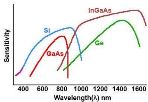
Fig.2.7.13 Relative Sensitivity of Photodiode Semiconductors
