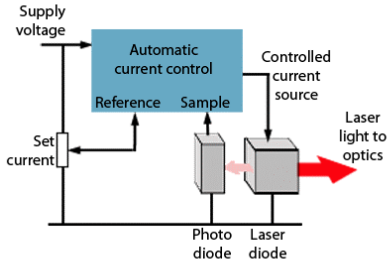
Fig. 2.6.6. Controlling the Laser Diode
