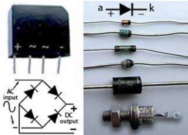
Fig. 2.8.4 Diode Polarity Markings.
