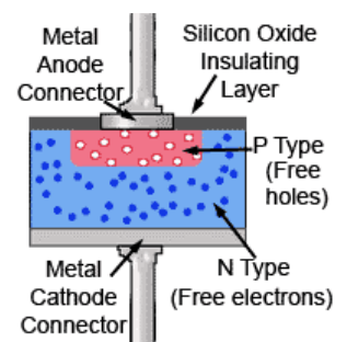
Fig 2.0.3 Silicon Planar Diode
