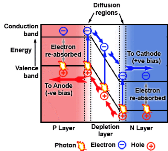
Fig.2.7.7 Energy Band Diagram of Photodiode Action
