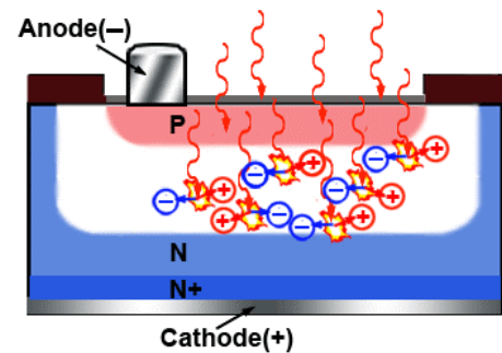
Fig. 2.7.4 Photons Create Electron/Hole Pairs
