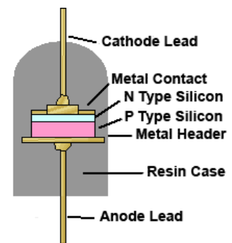
Figure 2.1.2. Silicon Rectifier Construction
