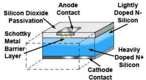
Figure 2.2.2. Small Signal Schottky Diode
