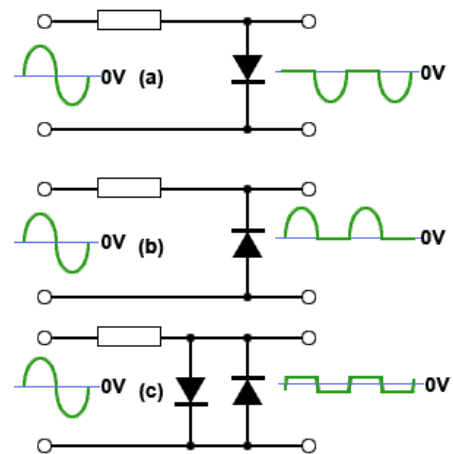
Figure 2.3.4. Clipping Action
