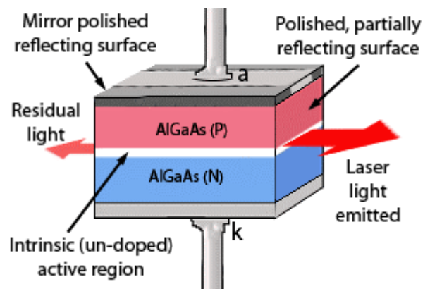
Fig. 2.6.2. Laser Diode Construction
