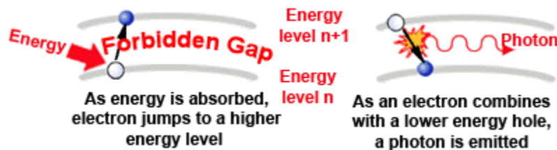
Fig. 2.6.3. The Absorption of Energy
