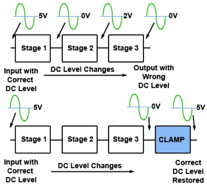
Figure 2.3.7. Clamping or DC Restoration
