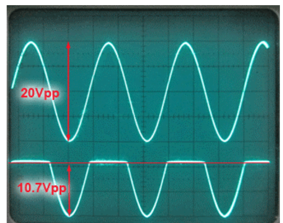
Figure 2.3.5. Clipping a 20Vpp Sine Wave
