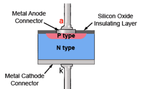
Figure 2.3.2. Simple Planar Diode
