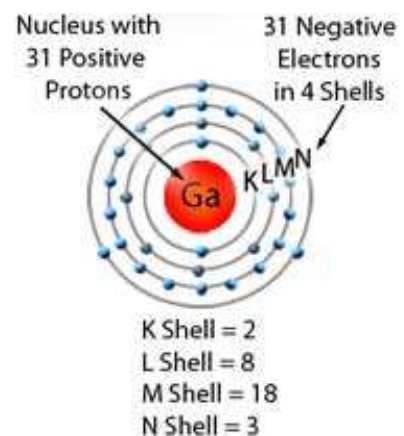
Fig. 2.6.1. An Atom of Gallium
