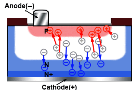
Fig. 2.7.5 Holes and Electrons are Attracted by Reverse Bias
