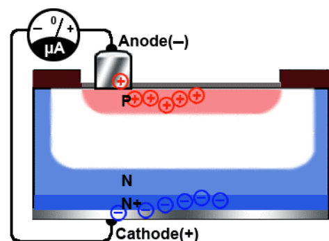
Fig. 2.7.6 Holes and Electrons Form a Photoelectric Current
