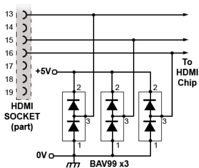
Figure 2.3.11. Protection Diodes
