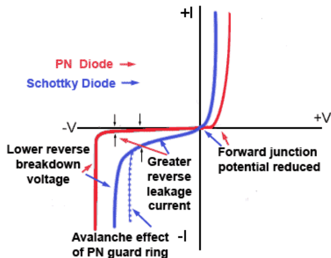
Figure 2.2.6. Schottky & PN Characteristics Compared
