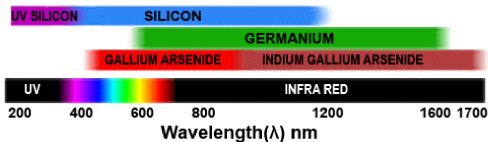
Fig. 2.7.10 Approximate Wavelength Ranges of Common Photodiode Materials
