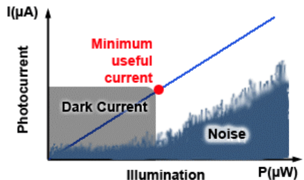
Fig. 2.7.9 Dark Current and Noise
