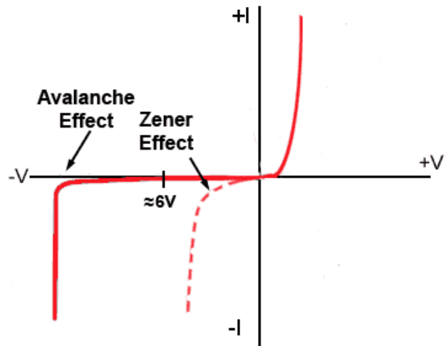
Figure 2.4.3. Zener & Avalanche Effects
