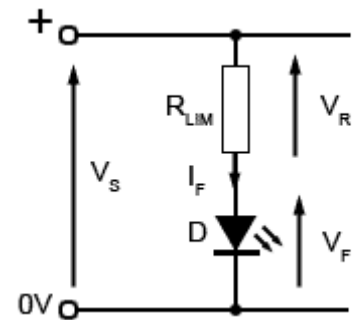
Figure 2.5.9. LED Current Limiting Resistor
