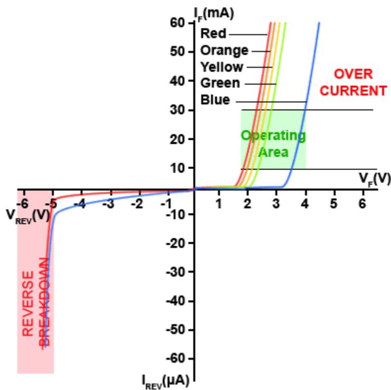
Figure 2.5.8. LED Characteristics Compared
