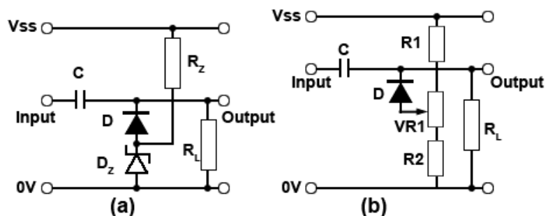
Figure 2.3.10. Changing Clamping Levels
