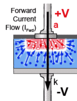
Fig 2.0.5 Diode Forward Conduction
