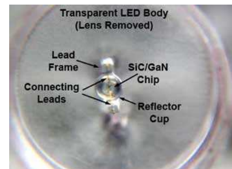
Figure 2.5.2. LED Construction (Side View)
