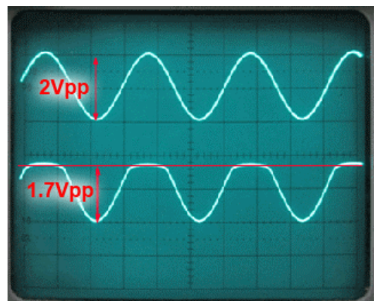
Figure 2.3.6. Clipping a 2Vpp Sine Wave
