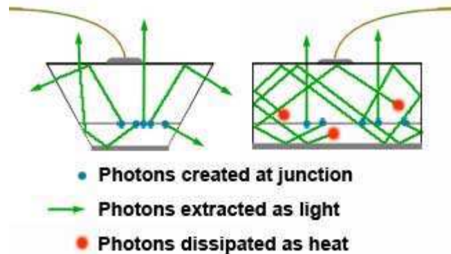
Figure 2.5.7. Internal Reflection
