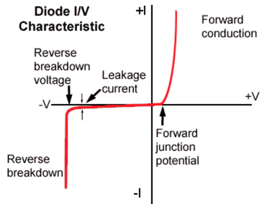
Fig 2.0.7. Typical Diode I/V Characteristic
