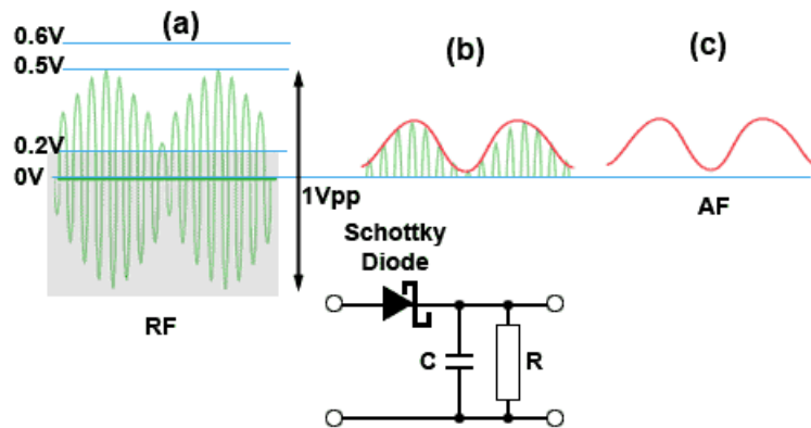
Figure 2.2.4. AM Demodulation Using a Schottky Diode
