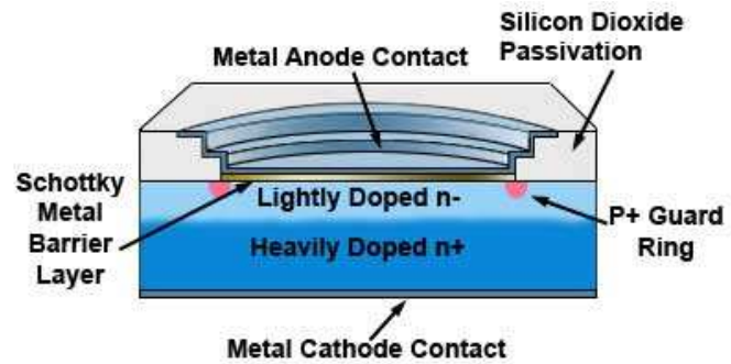
Figure 2.2.5. Schottky Rectifier Diode
