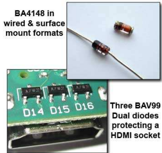
Figure 2.3.1. Small Signal Diodes
