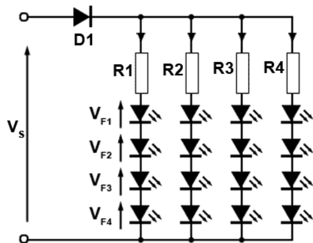
Figure 2.5.10. Series-Parallel LED Array
