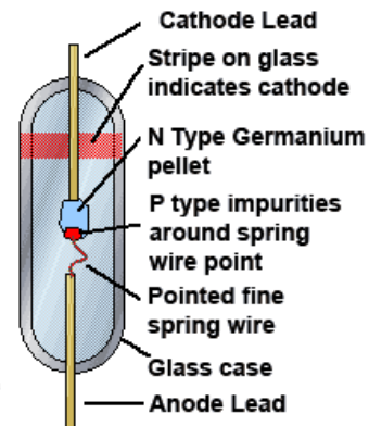
Figure 2.2.3. Germanium Point Contact Diode
