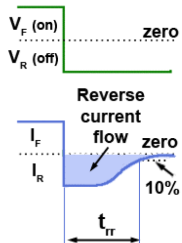
Fig 2.1.4 Reverse Recovery Time ( t_{rr} )
