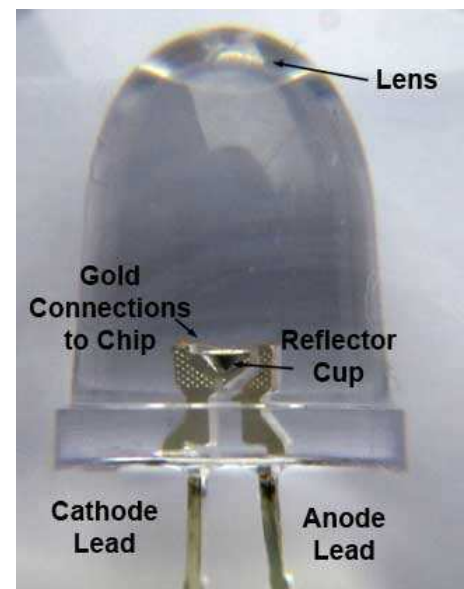
Figure 2.5.2. LED Construction (Side View)
