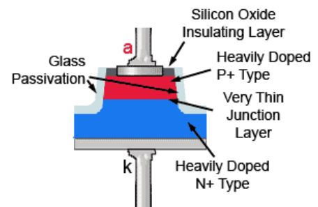
Figure 2.4.1. Zener Diode Construction
