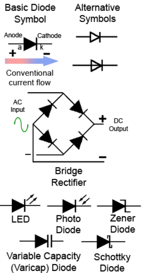
Fig 2.0.2 Diode Circuit Symbols
