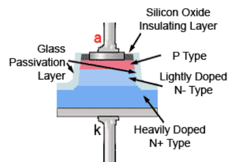
Figure 2.3.3. Simple Mesa Diode
