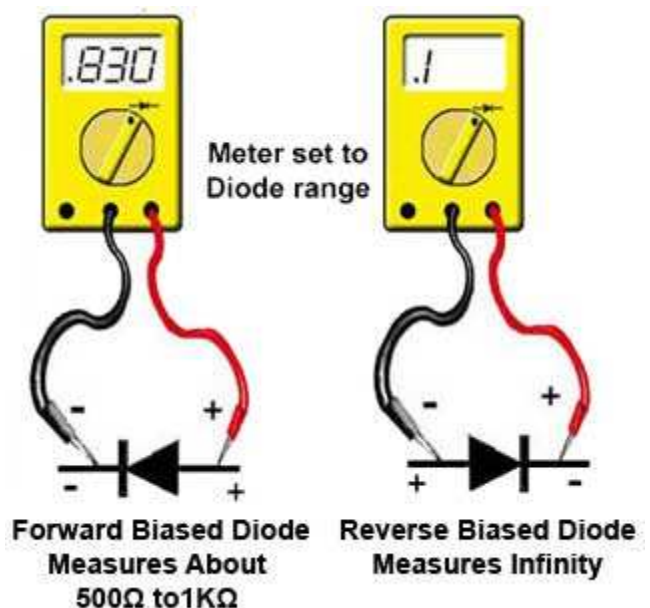
Fig. 2.8.3 Connecting a Digital Meter for Testing a Diode
