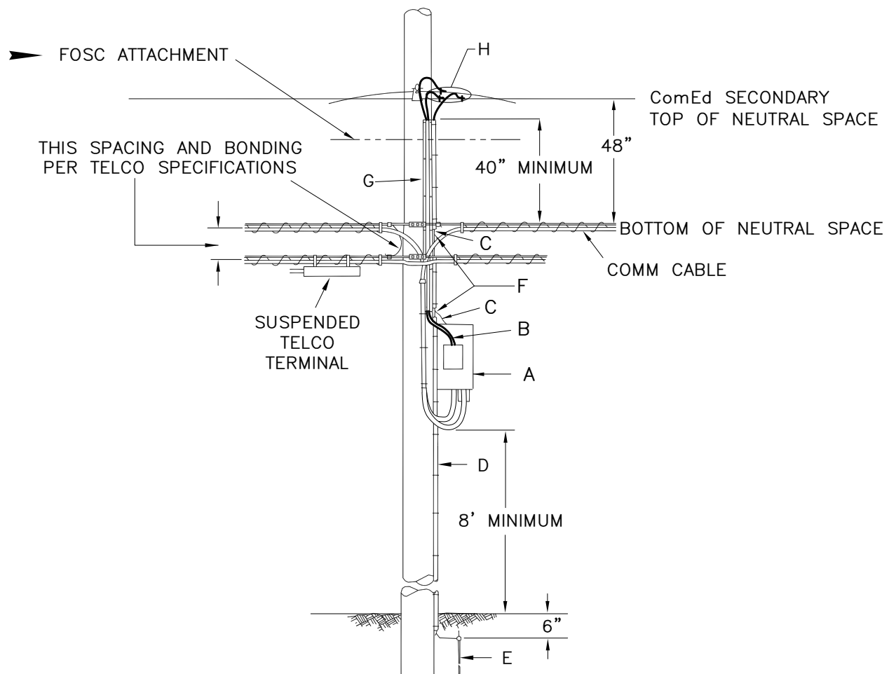
COMM POWER SUPPLY SERVICE SERVICE FROM OVERHEAD FACILITIES
