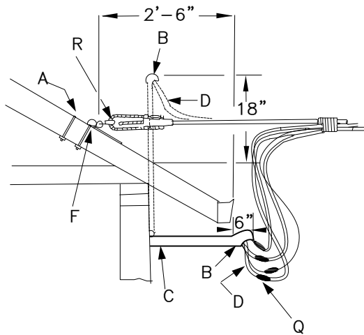
EXTENDED EAVES
