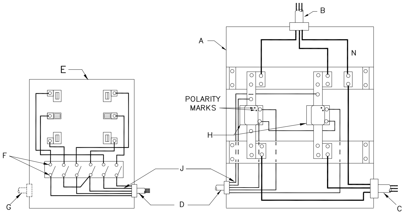
METER CONNECTION DEVICE
