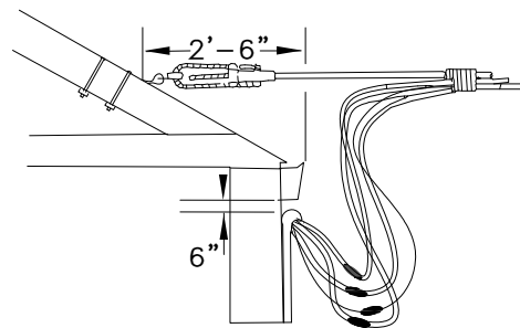
FLUSH EAVES
