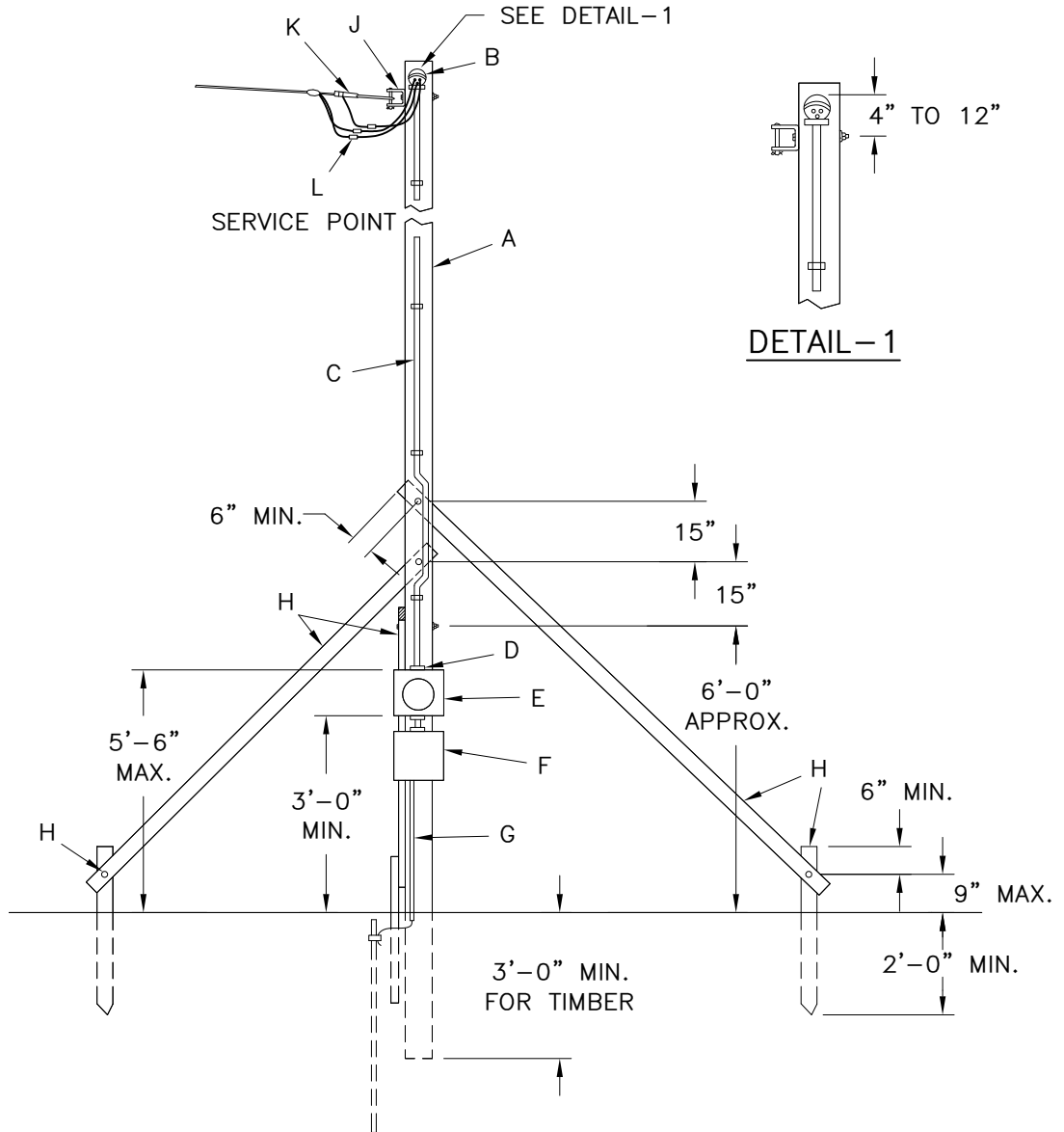
INSTALLATION OF CUSTOMER SERVICE POLE AND OUTDOOR METER CONNECTION DEVICE TEMPORARY SERVICE
