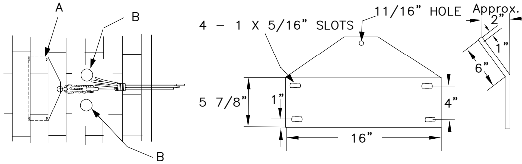
TYPE A ROOF PLATE
