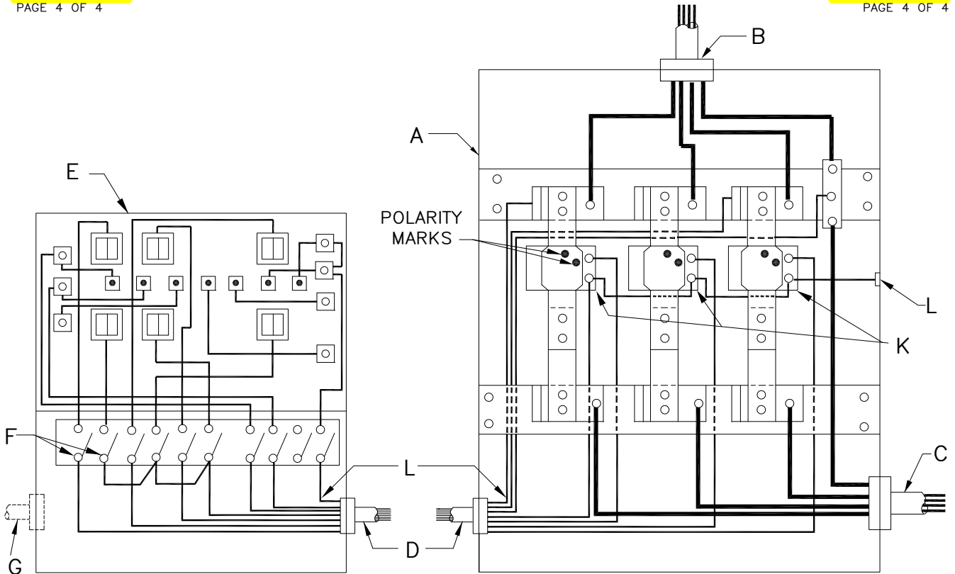
METER CONNECTION DEVICE
