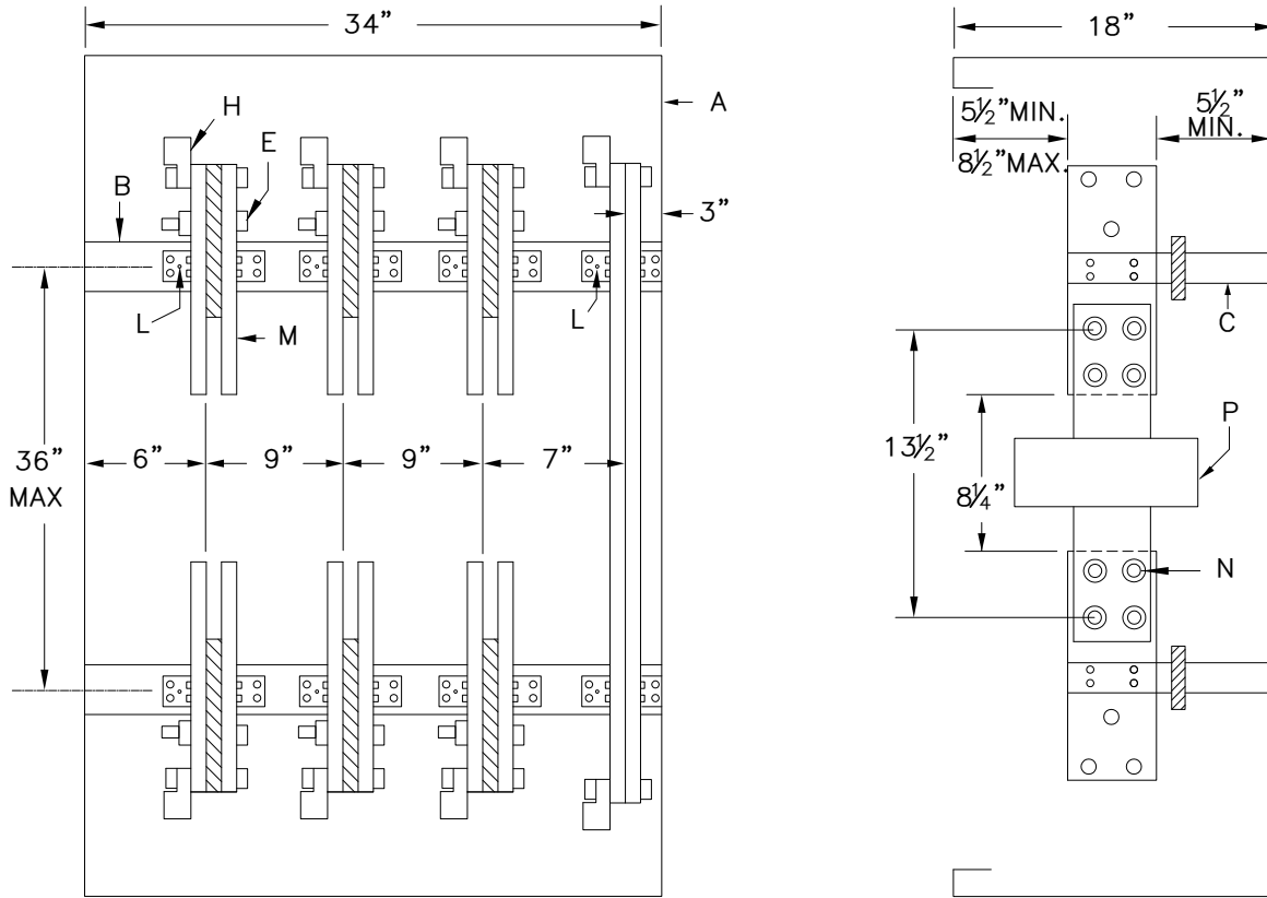
FIGURE 2 CURRENT TRANSFORMER COMPARTMENT > 800 AMPERES
