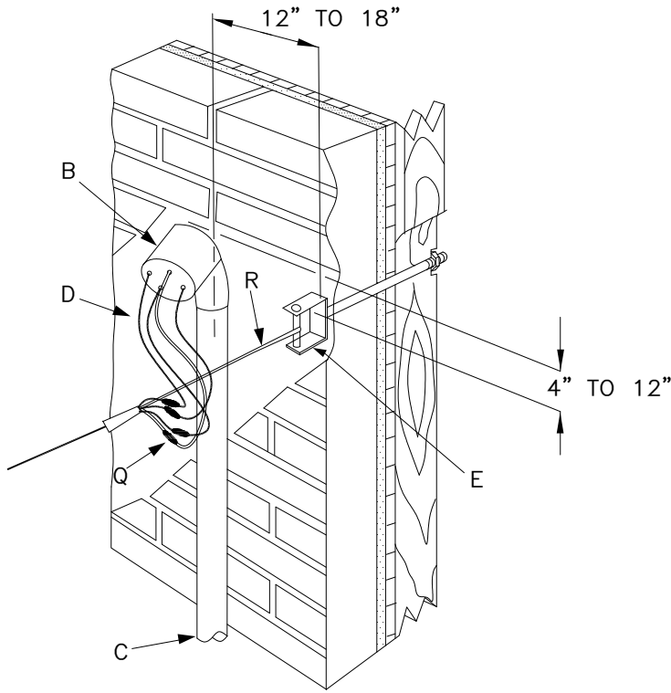
FIGURE-2 BRICK VENEER WALL INSTALLATION
