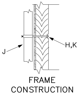
FIGURE-5 SERVICE ATTACHMENT WITH WOOD RISER
