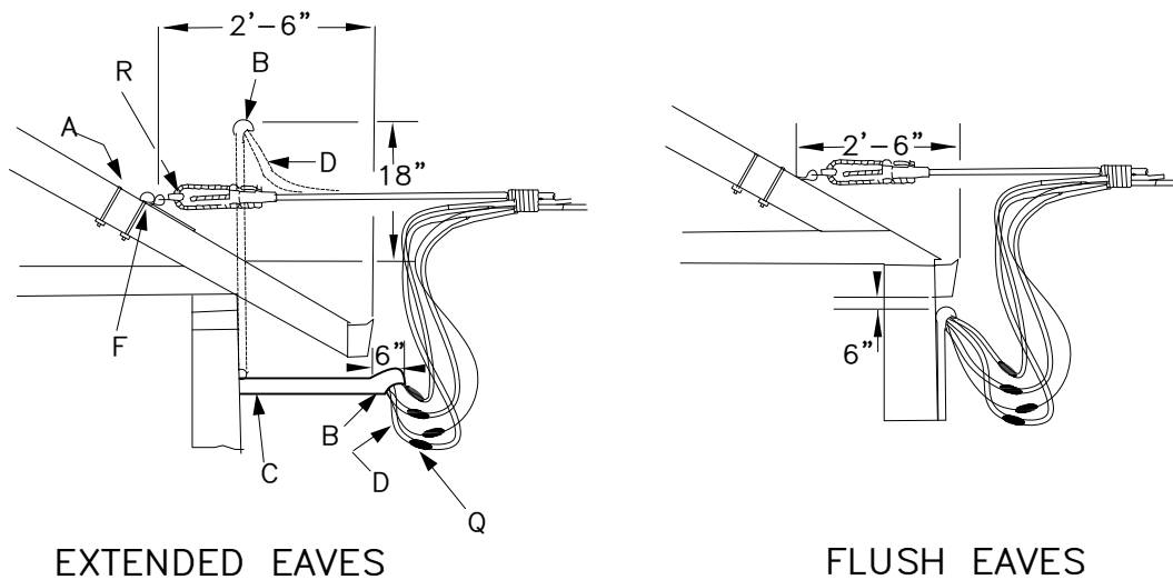
FIGURE-7 ROOF PLATE INSTALLATION
