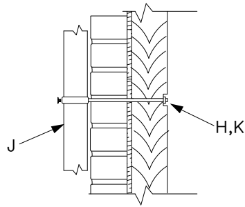
BRICK VENEER CONSTRUCTION
