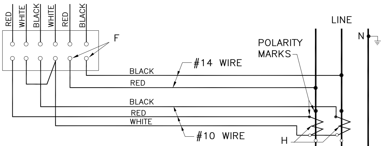
WIRING DIAGRAM
