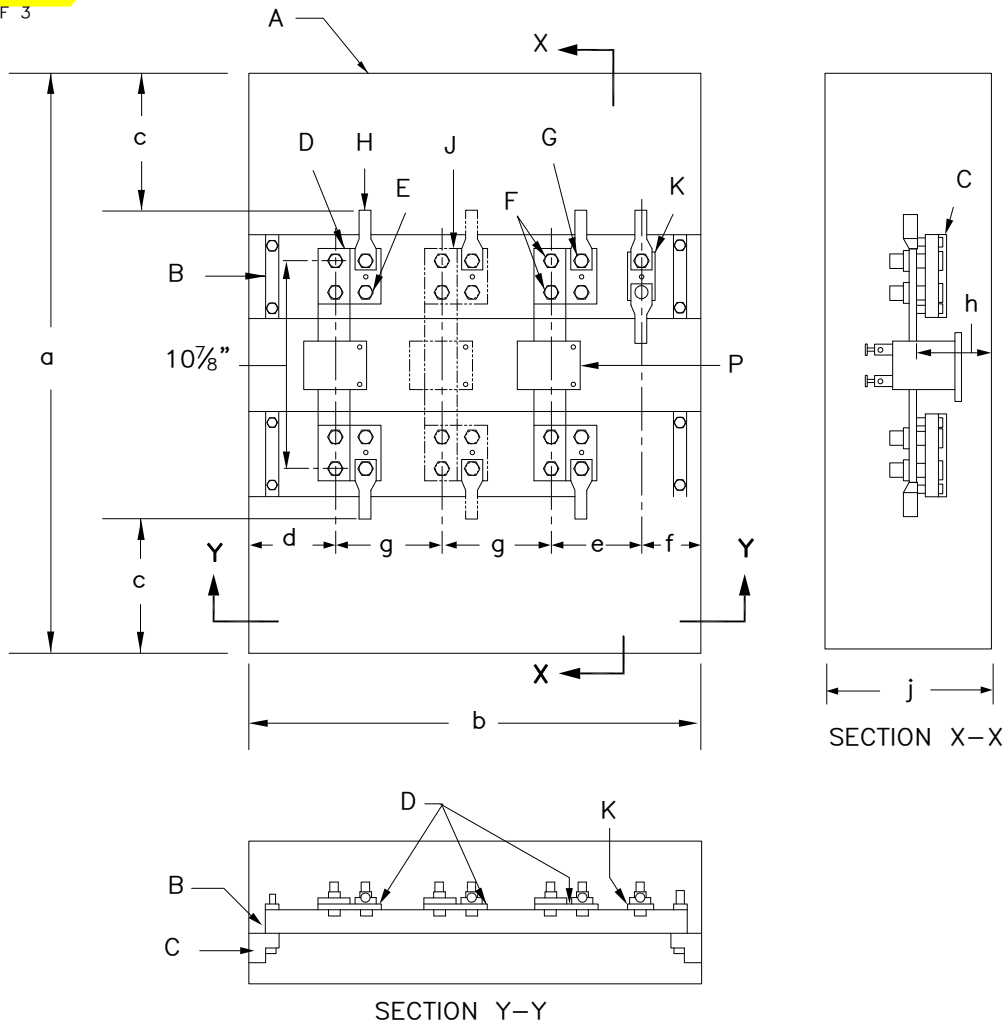
FIGURE 1 CURRENT TRANSFORMER COMPARTMENT ▶ ≤800 AMPERES
