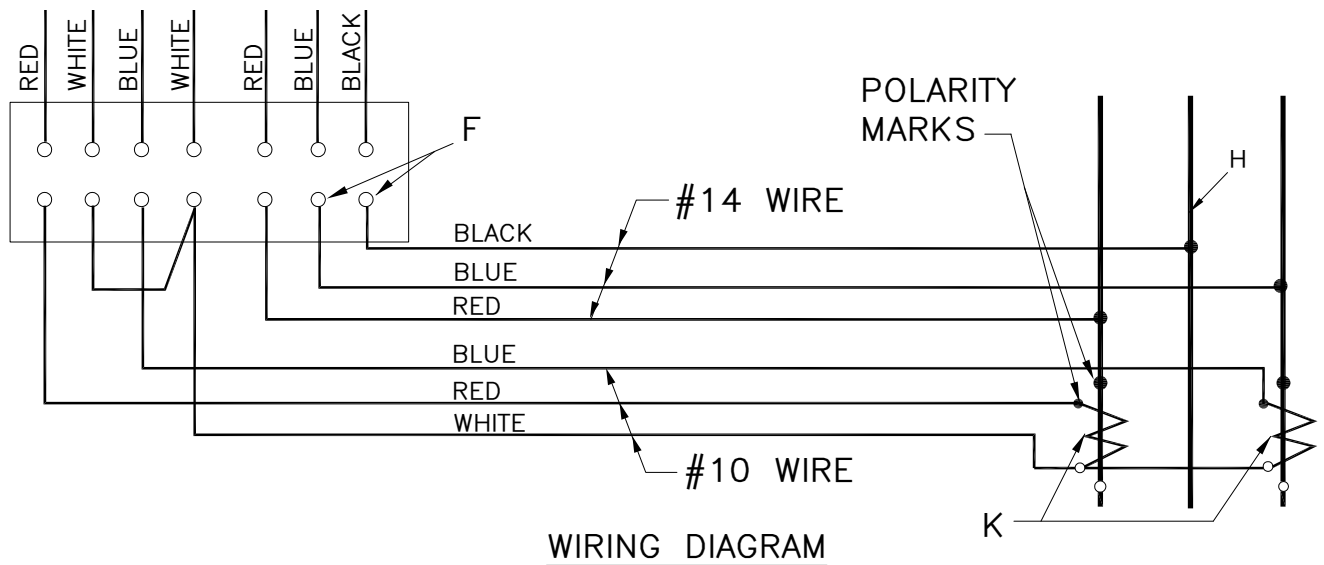
FIGURE 1 3-PHASE, 3-WIRE, 480V
