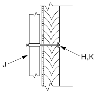
FRAME CONSTRUCTION
