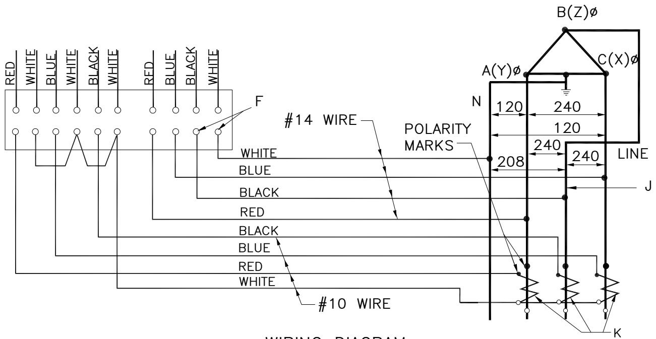
WIRING DIAGRAM
