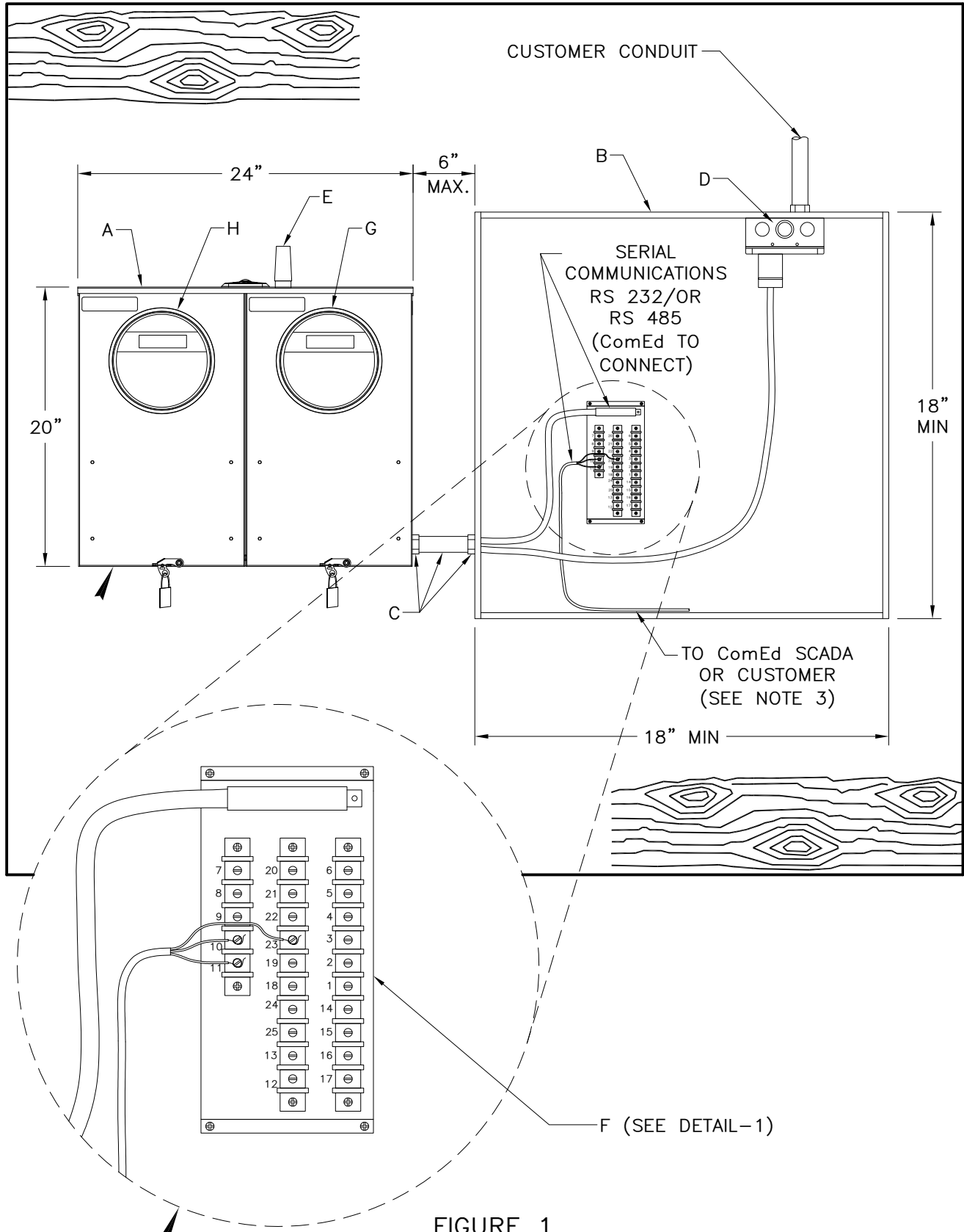
AMI METER ADJACENT TO SCADA METER WITH EMBEDDED CELL MODEM & SERIAL COMMUNICATIONS
