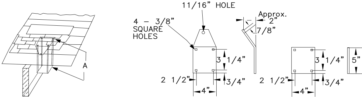
TYPE B ROOF PLATE
