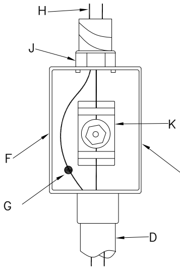
JUNCTION BOX
