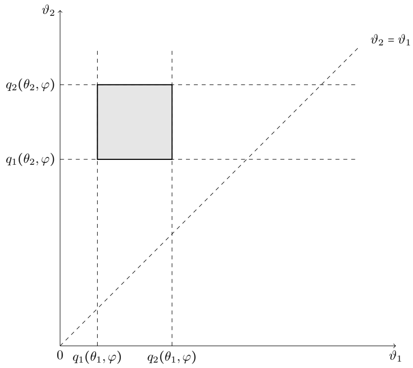
Figure C-2: area in the joint support where \vartheta_2 \geq \vartheta_1 (case 2)
