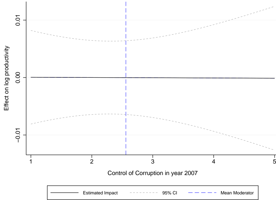
Figure 6: Impact of use unit increase in CSTRI (Mode 3) on y : Random assignment of w
