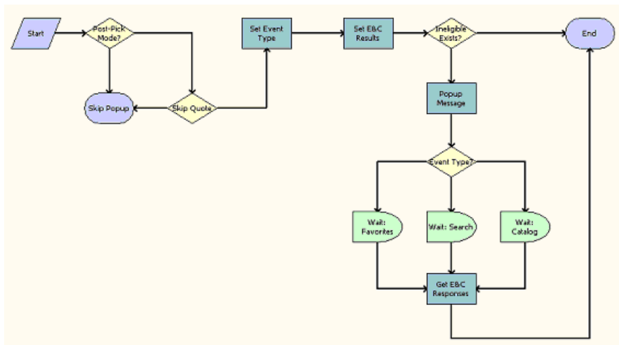
Figure 16. Compatibility Multiple Popup Workflow
