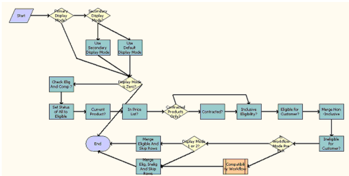
Figure 14. Product Eligibility & Compatibility - Default Workflow
