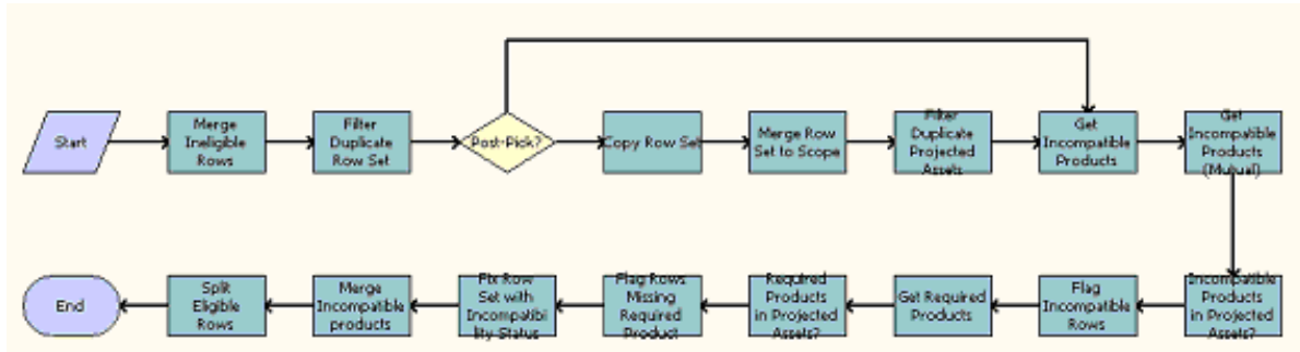
Figure 15. Product Compatibility - Default Workflow
