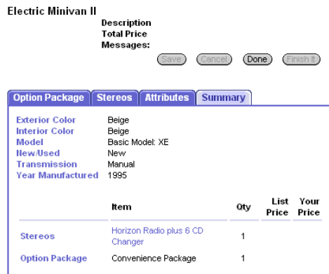
Figure 10. Example of a Summary Page
