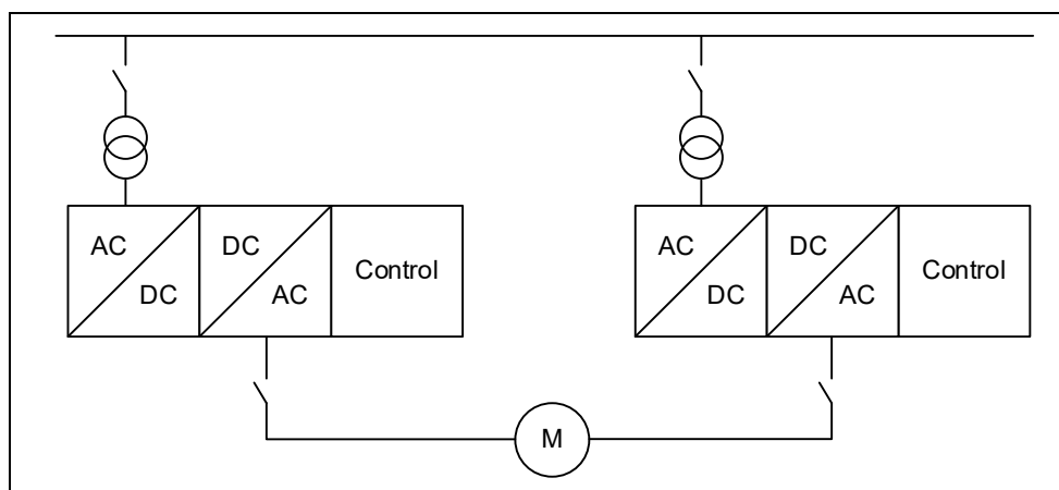
Fig. 7-4 Option L35: Redundant power section and control
