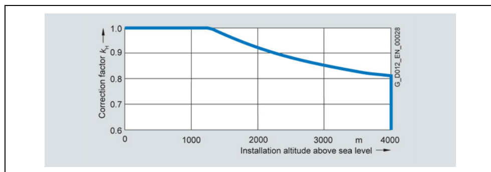
Fig. 5-15 Derating factor k_H for water cooling
