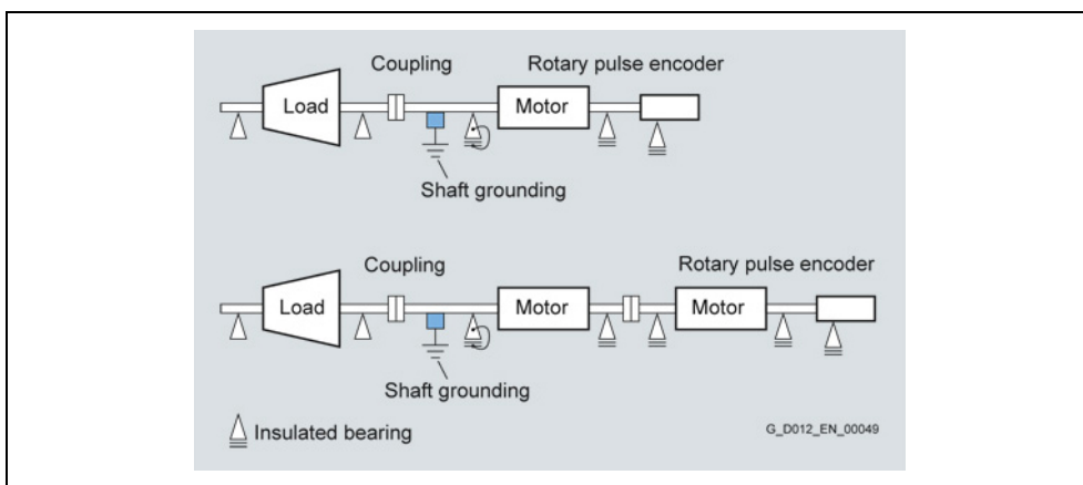
Fig. 11-3 Shaft grounding at the drive end
