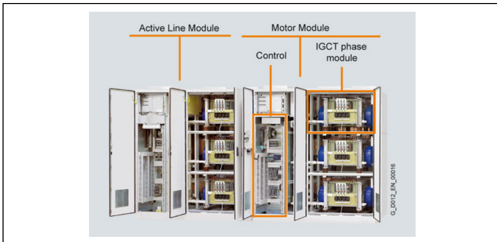
Fig. 5-2 SINAMICS SM150 in the IGCT version, internal design (without cooling unit)
