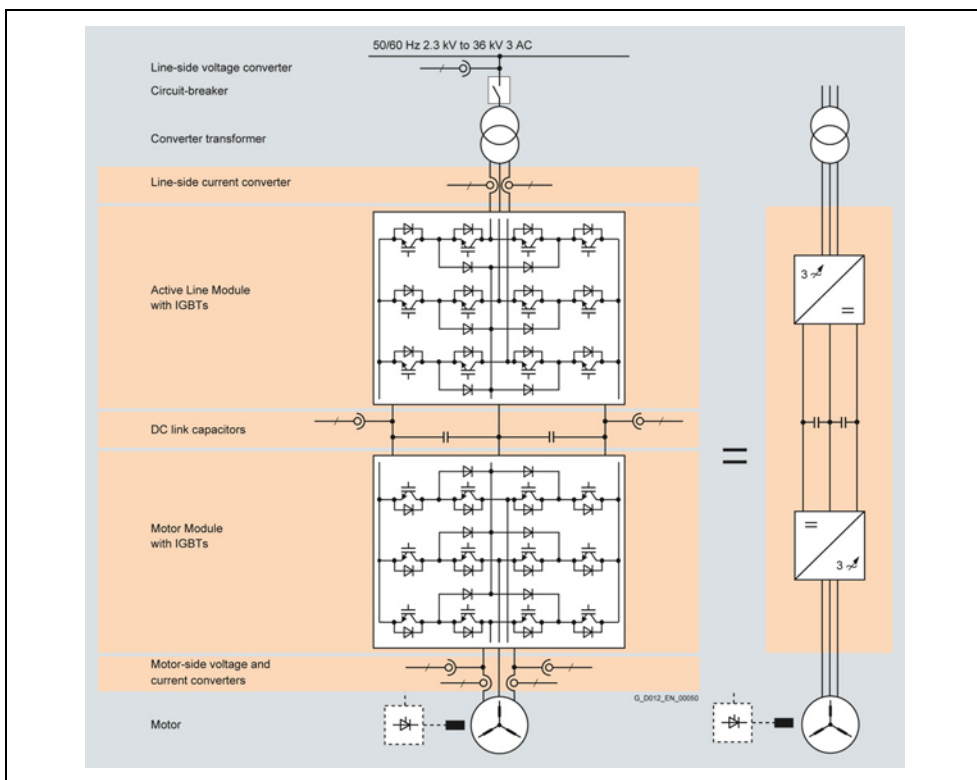
Fig. 4-3 Block diagram
