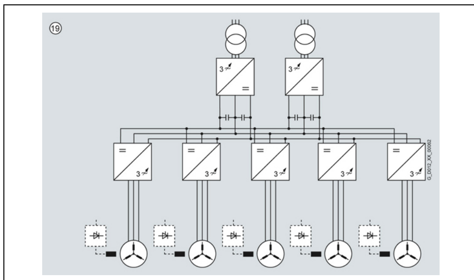
Fig. 5-12 DC bus configuration with two Active Line Modules and five motors connected to a common DC link
