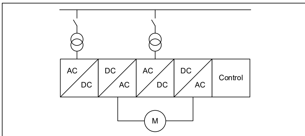
Fig. 7-5 Option L38: Redundant power section for parallel connection
