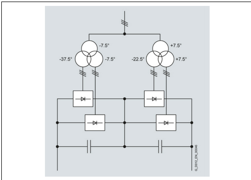
Fig. 7-8 SINAMICS GM150 in the IGBT version, 24-pulse infeed by connecting two Basic Line Modules in parallel (absolute values of the individual phase shift angles as example only)
