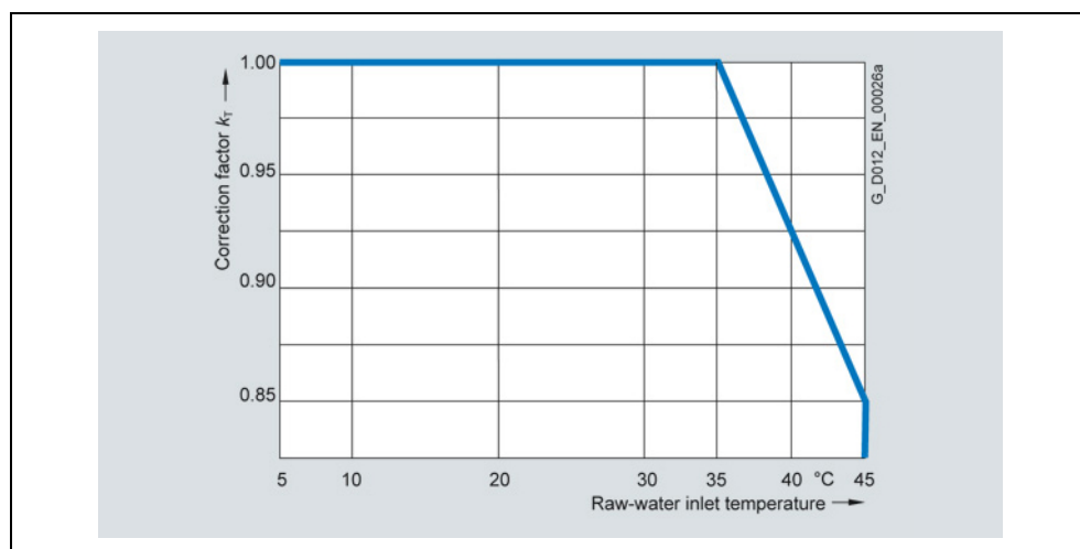
Fig. 5-16 Derating factor k_T (raw water intake temperature)
