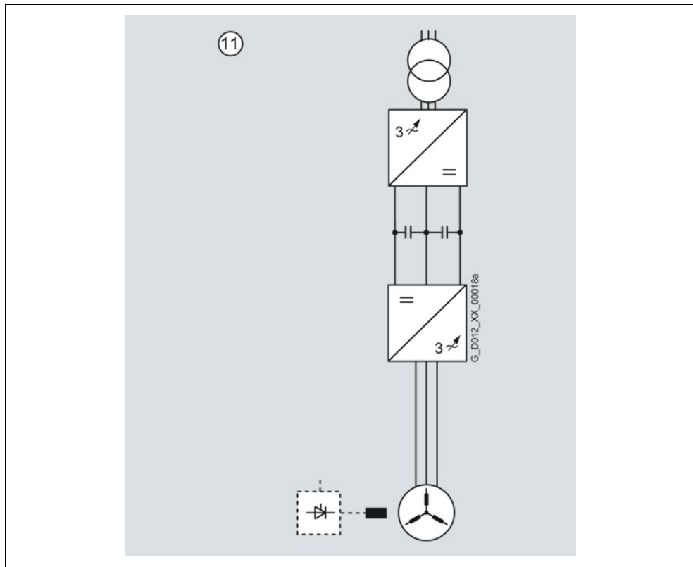
Fig. 4-4 Basic circuit
