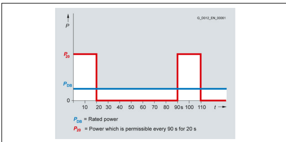
Fig. 7-7 Load diagram
