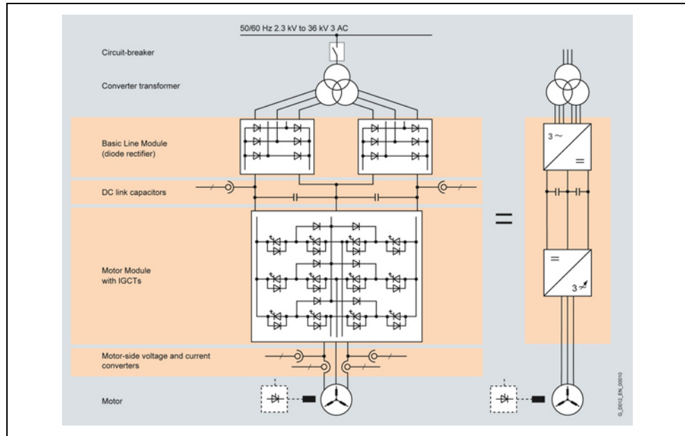
Fig. 3-3 Block diagram
