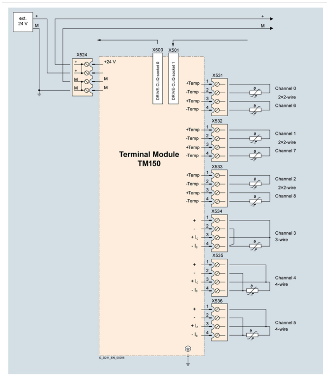
Fig. 7-2 Connection example, TM150 Terminal Module
