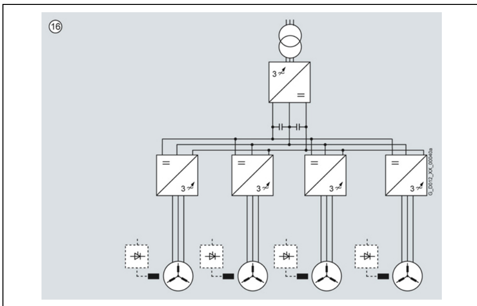
Fig. 5-9 DC bus configuration with four motors connected to a common DC link
