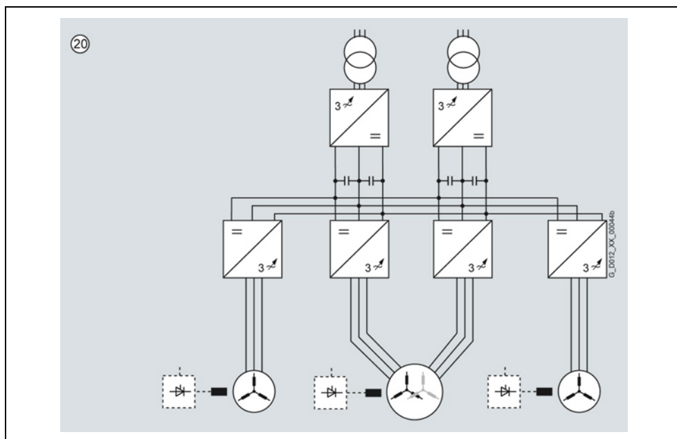
Fig. 5-13 DC bus configuration with two Active Line Modules and three motors connected to a common DC link (2 × 10 MVA, 1 × 20 MVA)
