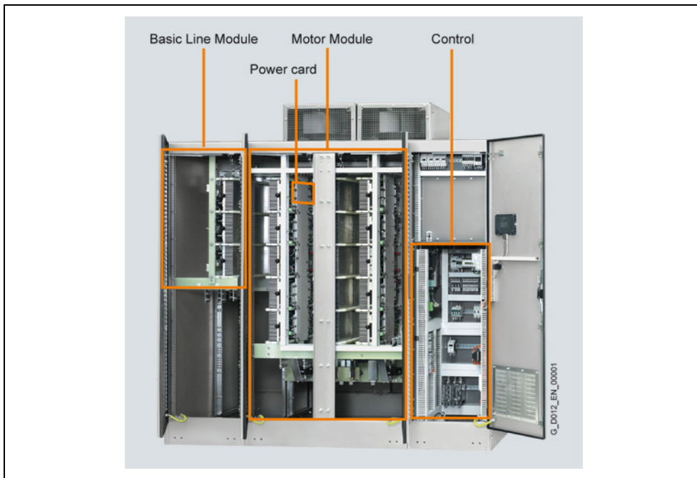
Fig. 2-2 SINAMICS GM150 as air-cooled IGBT version, internal design
