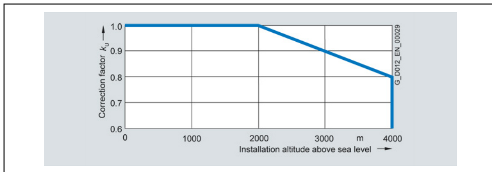
Fig. 5-17 Derating factor k_u
