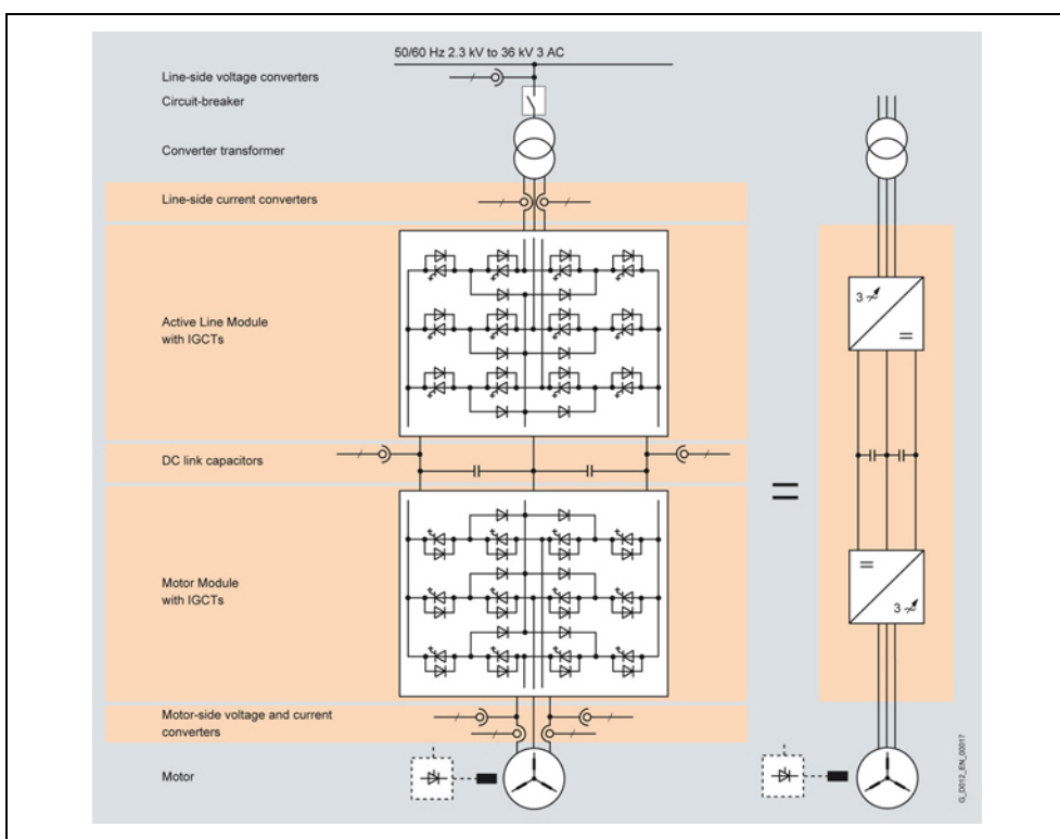
Fig. 5-3 Block diagram
