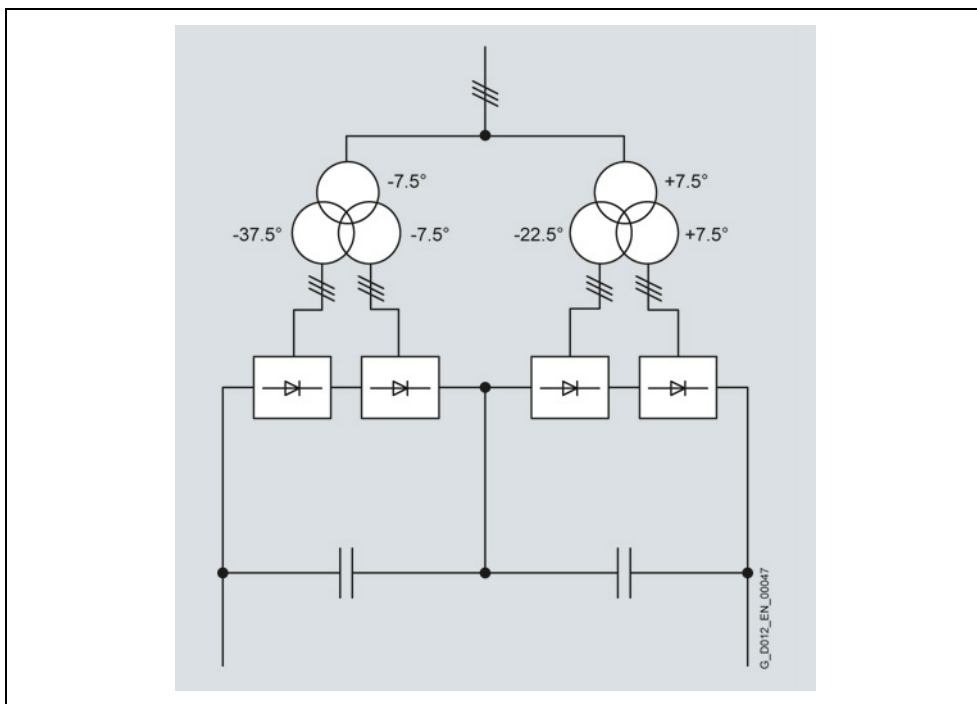
Fig. 7-9 SINAMICS GM150 in the IGCT version, 24-pulse infeed by connecting two Basic Line Modules in series (absolute values of the individual phase offset angles are examples only)
