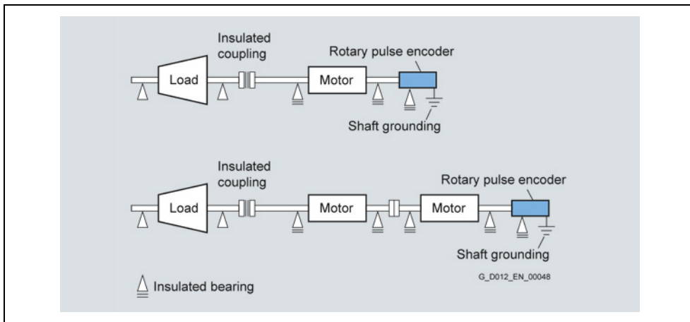
Fig. 11-2 Shaft grounding at the non-drive end
