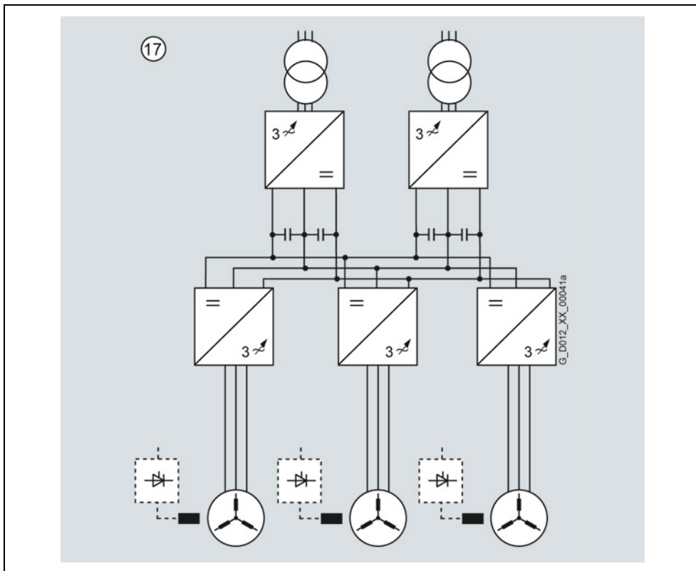
Bild 5-10 DC bus configuration with two Active Line Modules and three motors connected to a common DC link
