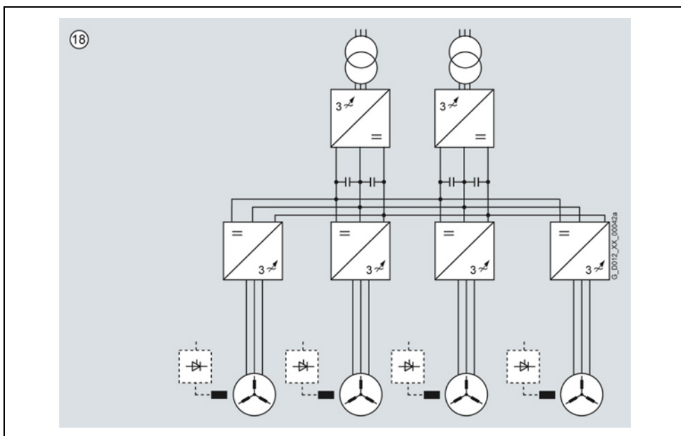
Fig. 5-11 DC bus configuration with two Active Line Modules and four motors connected to a common DC link
