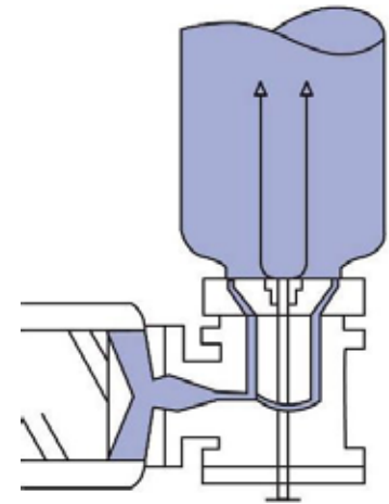
The polyethylene granulates are melted in five extruders and blown to a slide each.
