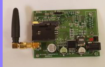
TTL GPRS Modem Board
