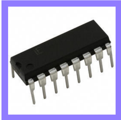
ISL83202IPZ- 55V, 1A Peak Current H-Bridge FET Driver
