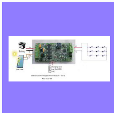
10w Solar Street Light Driver Module
