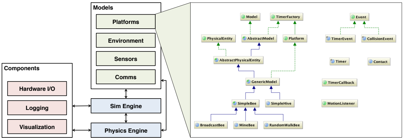
Figure 1: The Simbeotic architecture. Domain models are plugged into a discrete event simulation engine. The kinematic state of models with physical presence is managed by an integrated physics engine. Several levels of abstraction in the model layer provide flexibility and convenience to modelers. The simulation architecture can be augmented by user-supplied plugin components.
