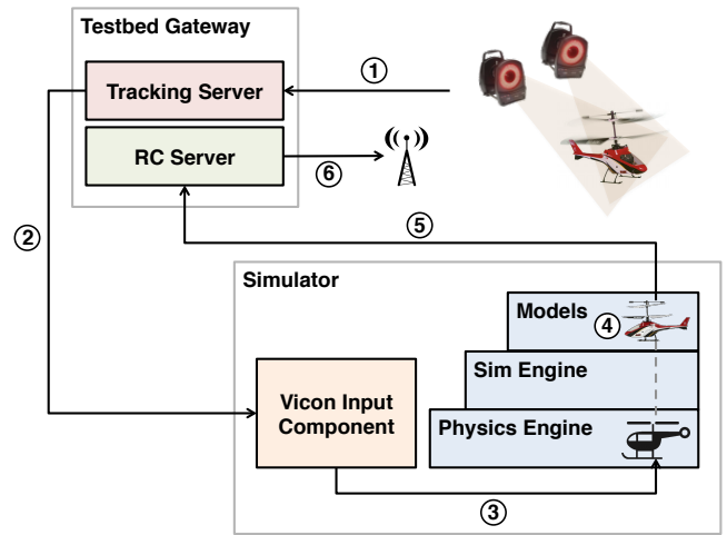
Figure 5: The HWIL cycle in Simbeotic. Vicon cameras track the position and orientation of a helicopter and push frames to a tracking server (1), which pushes updates (2) to registered clients. A Vicon input component in Simbeotic receives the update and overrides the kinematic state (3) of the corresponding object in the physics engine. When the ghost model executes an event (4) it has the most recent state of the helicopter. If a command is issued, it is sent to the RC command server (5) where it is dispatched by the RF transmitter (6) to the helicopter.
