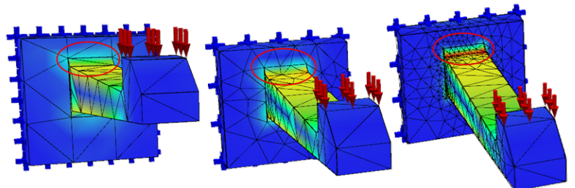
Initial Mesh - Error 13% Refinement 1 - Error 8% Refinement 2 - Error < 5% h-Adaptivity refines the mesh until an error threshold is achieved
