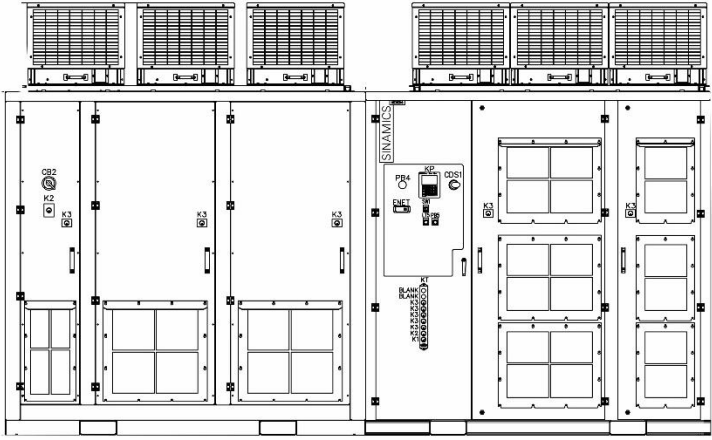
6SR4 9/12/15/18 cell 500-750A Drawing G
