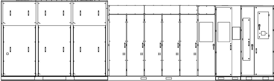
GH180 9-24 cell 880-1375A with option cabinet (width 36") Drawing
