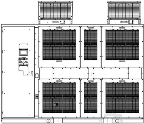
6SR5 12/15 cell 200-260A Drawing E
