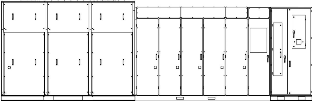
GH180 9-24 cell 880-1375A Drawing M
