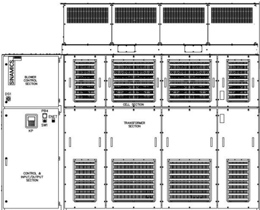
6SR4 9/12 cell 315-375A Drawing F
