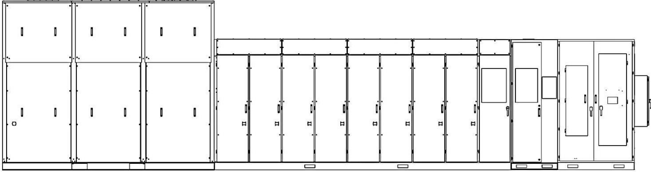
GH180 24 cell 880-1375A with option cabinet, 60" cooling cabinet and control box of the external Liquid-to-Air Heat Exchanger Drawing N
