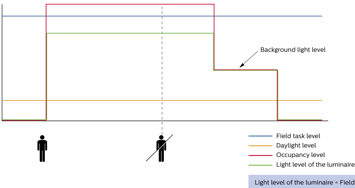
Figure 6. Lighting control behavior with low daylight level.
