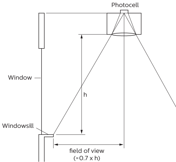
Figure 3. Sensor placement.
