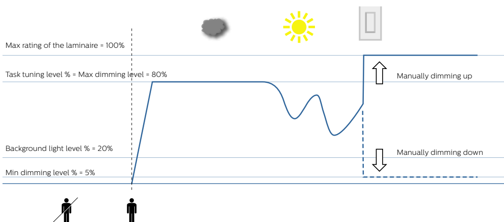
Figure 8. Automatic lighting control with manual dimming override.
