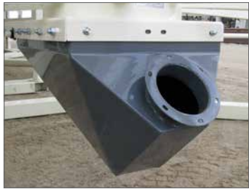
Auger Boots Fastens under slide gate assembly. Standard & Flex Auger boots available.
