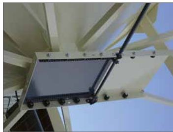
S.S. Slide Gate Assembly Complete Stainless Steel assembly.
