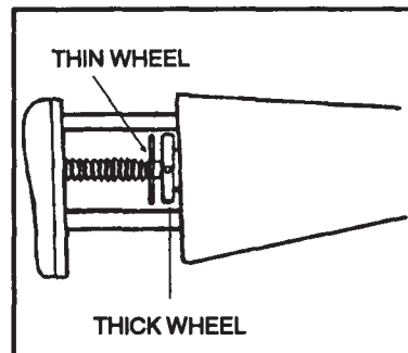
Figure 2-7. Stock adjustment.
