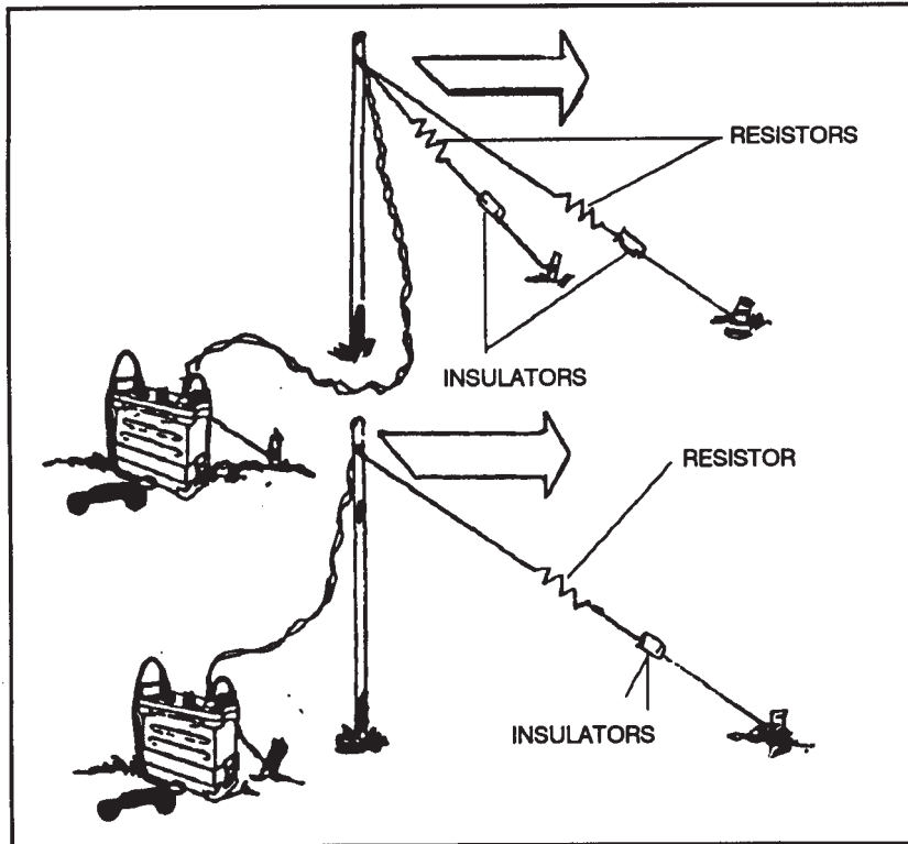
Figure 7-12. Sloping-V antenna.
