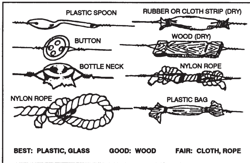
Figure 7-2. Improvised Insulators.
