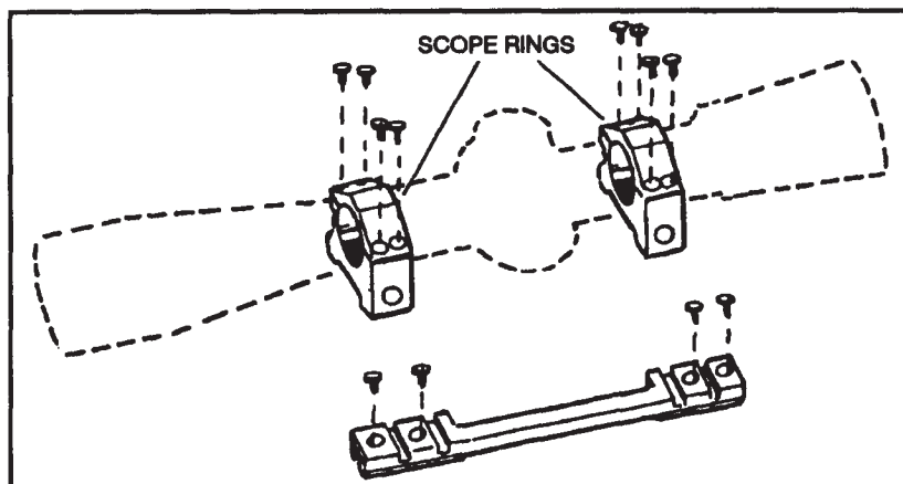
Figure 2-20. Scope mount.
