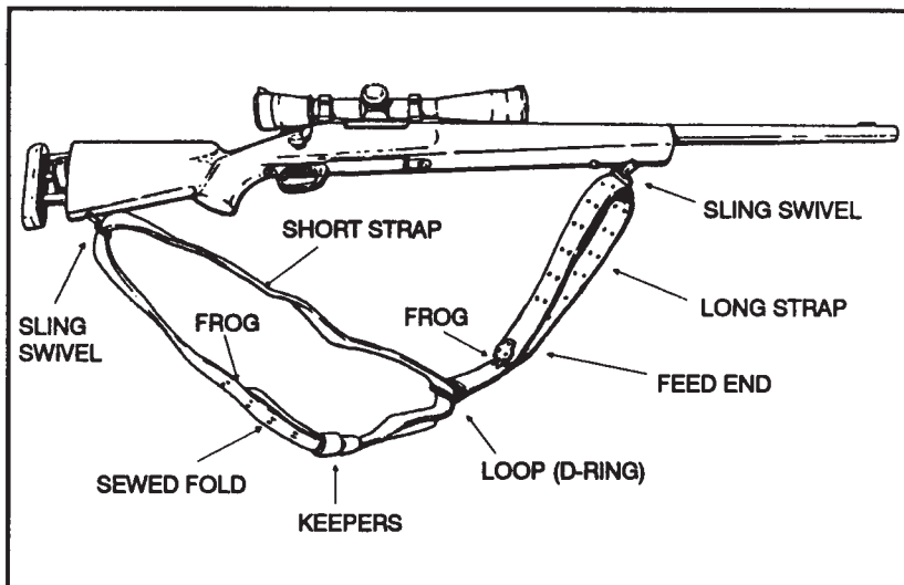
Figure 2-8. Leather Sling.
