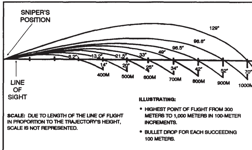
Figure 3-25. Trajectory chart.
