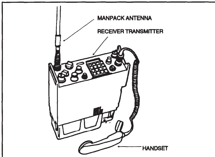
Figure 2-36. AN/PRC-119 radio.
