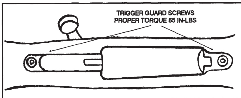
Figure 2-15. Trigger guard screws.
