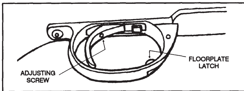
Figure 2-6. Trigger adjustment.
