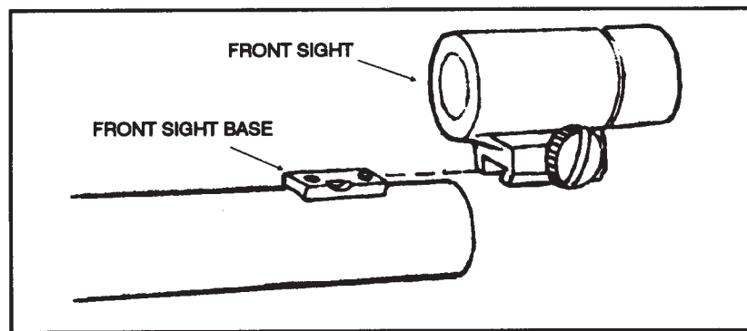
Figure 2-22. Front sight attachment.
