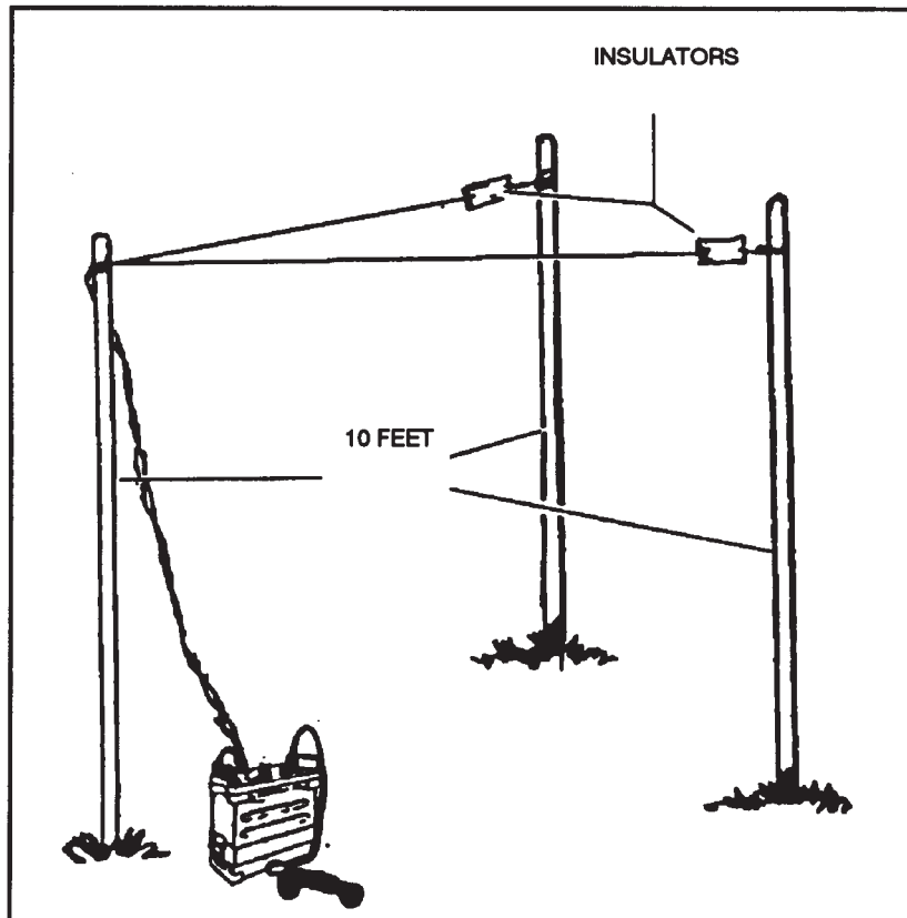
Figure 7-11. V antenna.
