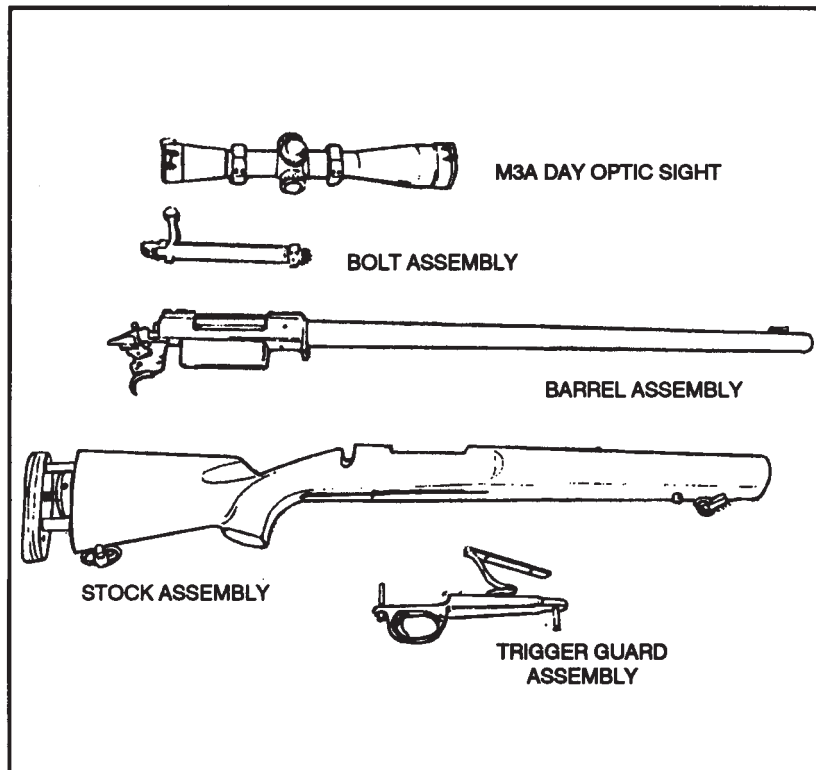
Figure 2-16. Disassembled weapon.
