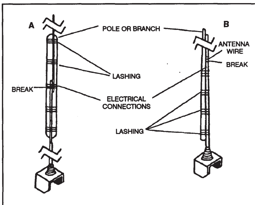
Figure 7-1. Emergency repair of broken whip antenna.
