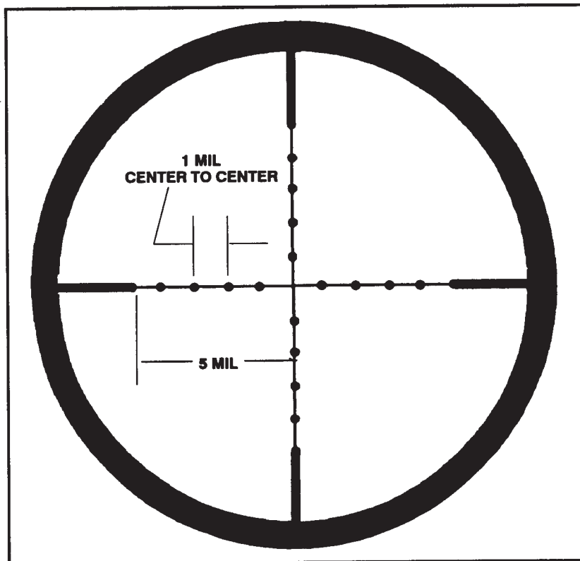
Figure 2-21. Mil-dot reticle.
