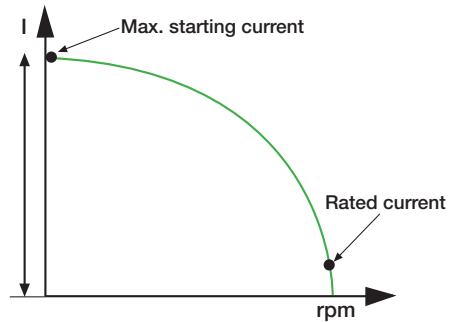
Current curve at D.O.L. start
