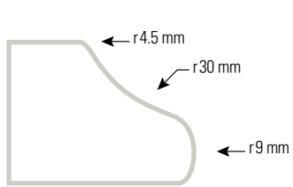
BIG OGEE GRANDE DOUCINE
