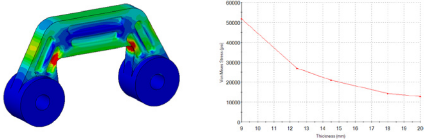
FIGURE 3: PARAMETER SENSITIVITY STUDY—STRESS VS. THICKNESS
