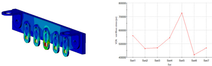
FIGURE 4: SETUP FOR MULTIPARAMETER SENSITIVITY STUDY USING DESIGN SCENARIOS
