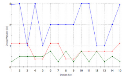
FIGURE 7: OPTIMIZATION OF SPINDLE SHAPE WITH VARIABLE FILLET RADIIUSES
