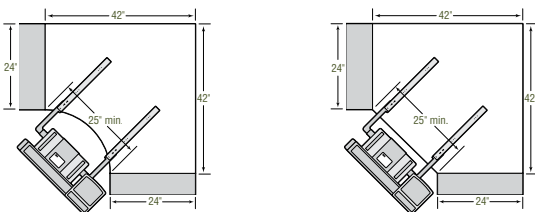
42" X 24" L Curved corner work surface
